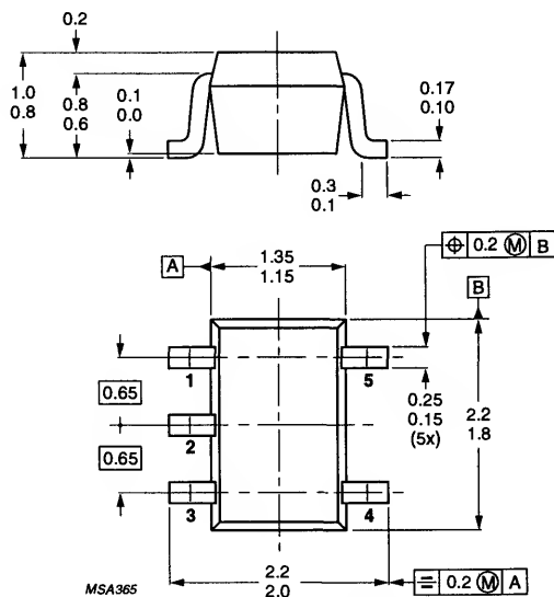
SC70(a)
