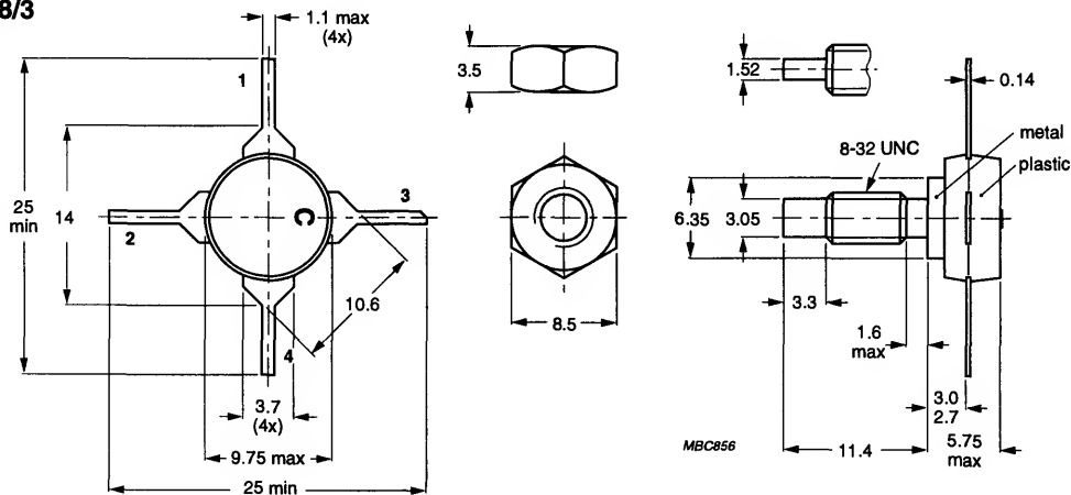
SOT48/3
