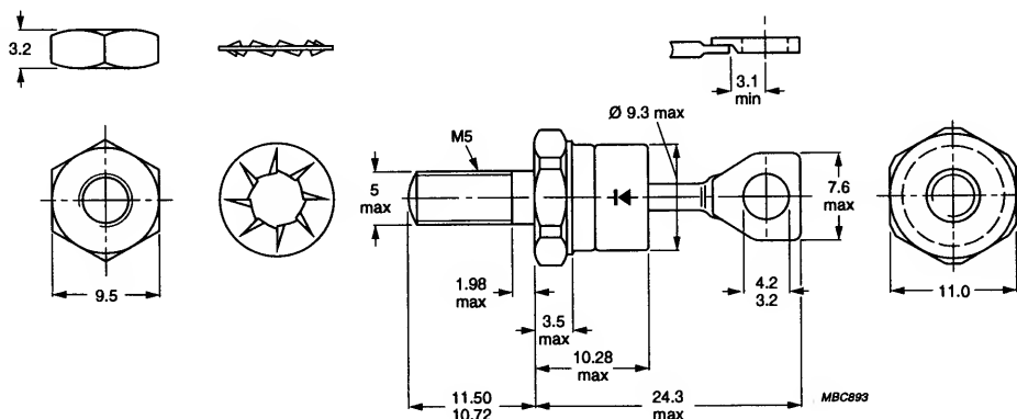
DO-4(2)
