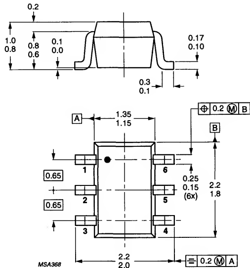
SC70(b)
