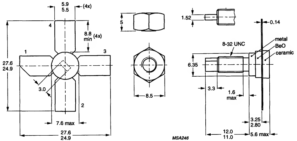
SOT122A
