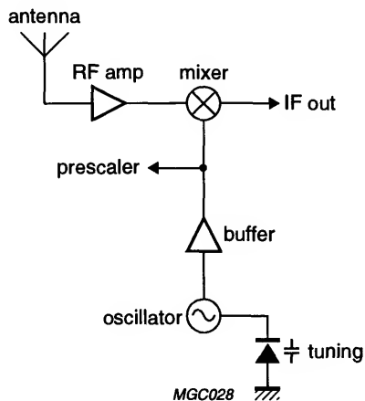
Fig.1 Typical front-end section for pagers
