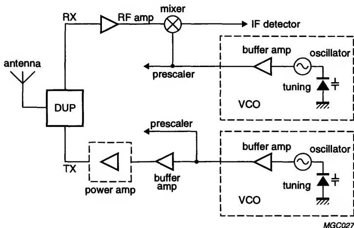
Fig.2 Typical RF section for cordless and cellular phones
