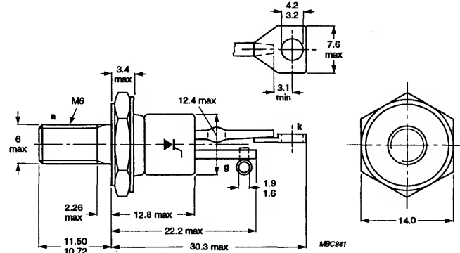
TO-48(2)
