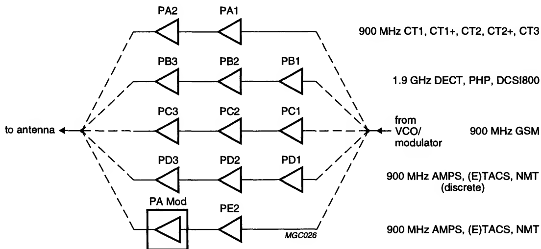
Fig.3 Typical power amplifier section for cordless and cellular phones
