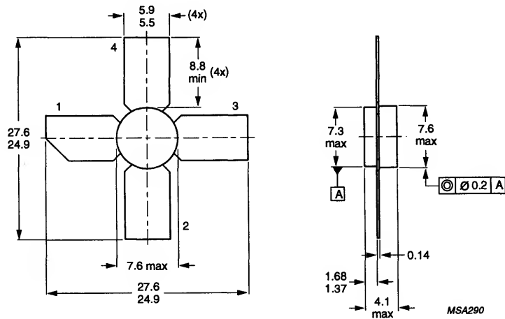
SOT122D
