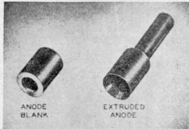
Fig. 9—Fabrication of anode.
