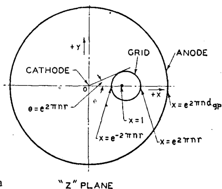
Fig. 4—Cross section of the triode of Fig. 3 transformed from the w plane to the z plane.
