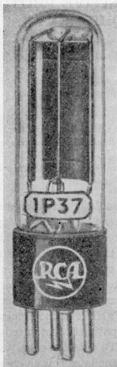
FIG. 8. Photograph of 1P37 .
