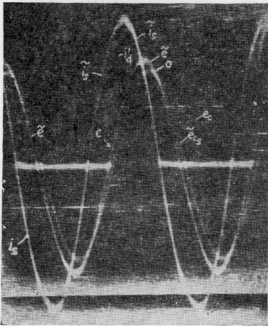
Fig. 31—Oscillograms taken with circuit of Fig. 30.
