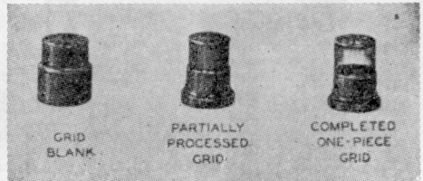
Fig. 8—Fabrication of one-piece grid.
