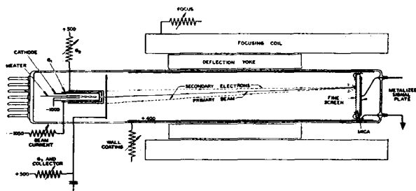
Fig. 4—Schematic diagram of SDT storage tube.
