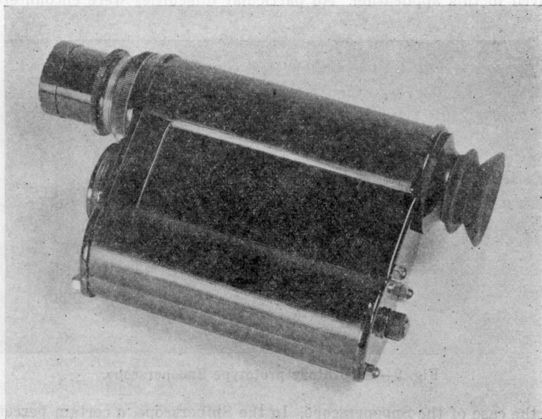
Fig. 8—Experimental telescope.
