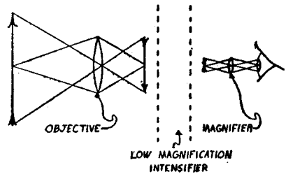
Fig. 7—Low magnification brightness intensifier.
