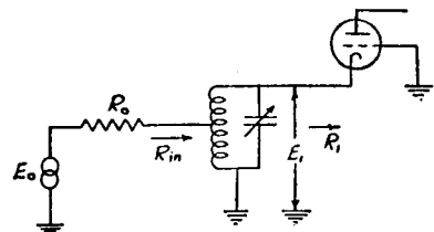
Fig. 6—Antenna input circuit for grounded-grid amplifier.
