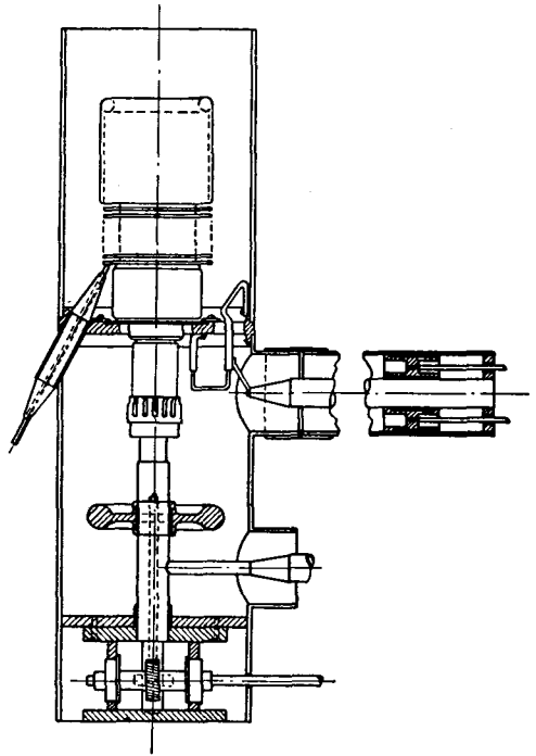
Fig. 4—Cross section of the "half-wave" oscillator circuit.
