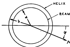
Fig. 2—Cross sectional view of traveling-wave tube defining the coordinate system used. Positive direction of z is into the page.
