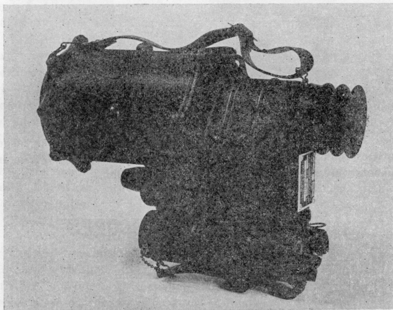
Fig. 1—Infrared telescope.
