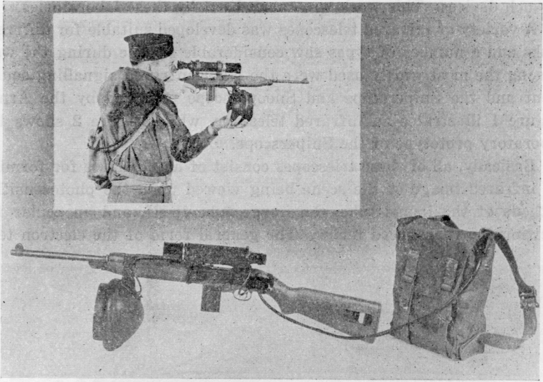
Fig. 2—Laboratory prototype sniperscope.
