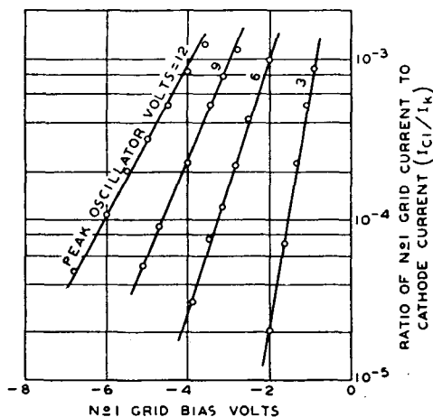
Fig. 15—Signal-grid (grid No. 1) current in a typical mixer with a 20-megacycle oscillator voltage applied to grid No. 3. E_{c3} = -10 volts. E_{c2 \text{ and } 4} = 100 volts, E_b = 250 volts.
