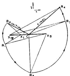
Fig. 7—The graphical construction for the transverse field of Fig. 6. The radius vector representing the initial circular motion is CR_0 , its magnitude being drawn proportional to the actual radius in centimeters, determined by
