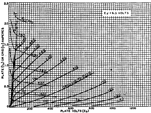
Fig. 12—Characteristic curves.
