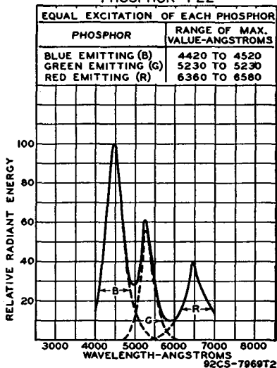
SPECTRAL-ENERGY EMISSION CHARACTERISTIC OF GROUP PHOSPHOR P22
