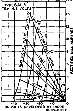
AVERAGE CHARACTERISTICS HALF-WAVE RECTIFICATION-SINGLE DIODE
