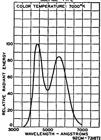
SPECTRAL-ENERGY EMISSION CHARACTERISTIC OF PHOSPHOR P4 SULFIDE TYPE
