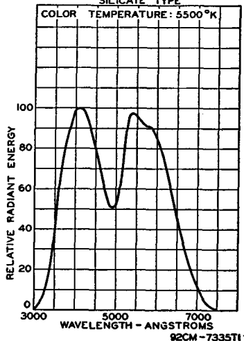
SPECTRAL-ENERGY EMISSION CHARACTERISTIC OF PHOSPHOR P4 SILICATE TYPE
