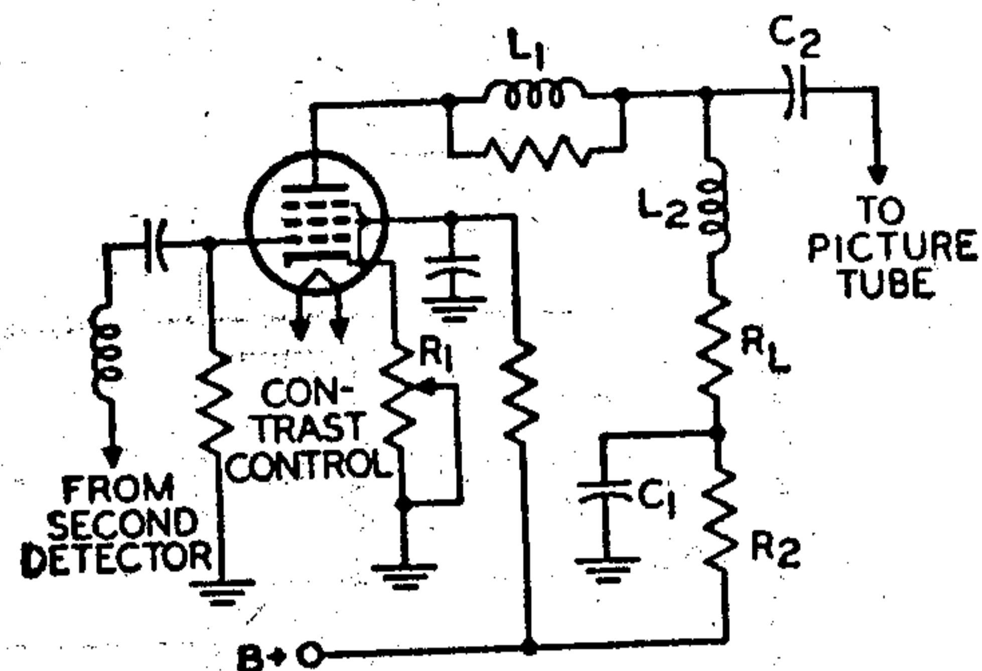
Fig. 76—Typical video amplifier stage.
