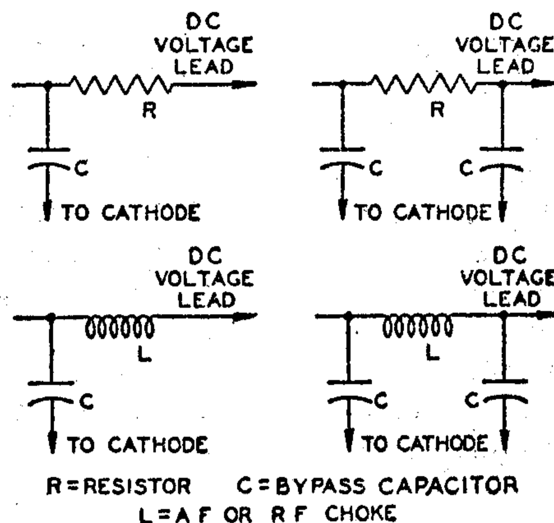
Fig. 120—Typical filter circuits.
