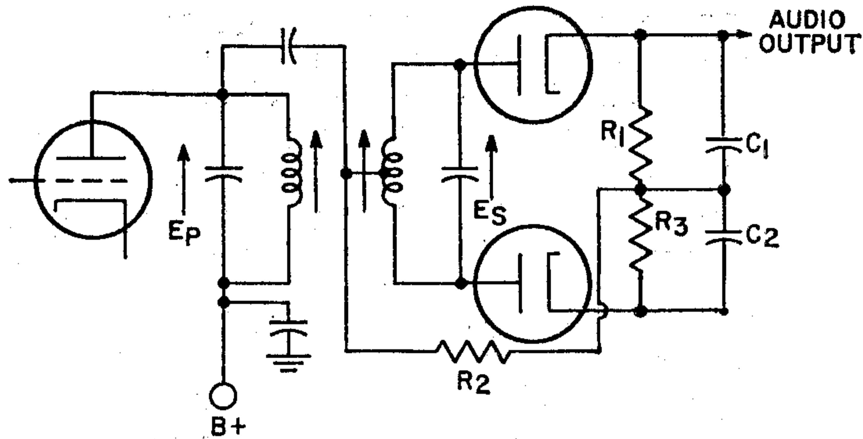
Fig. 30—Balanced phase-shift discriminator circuit.
