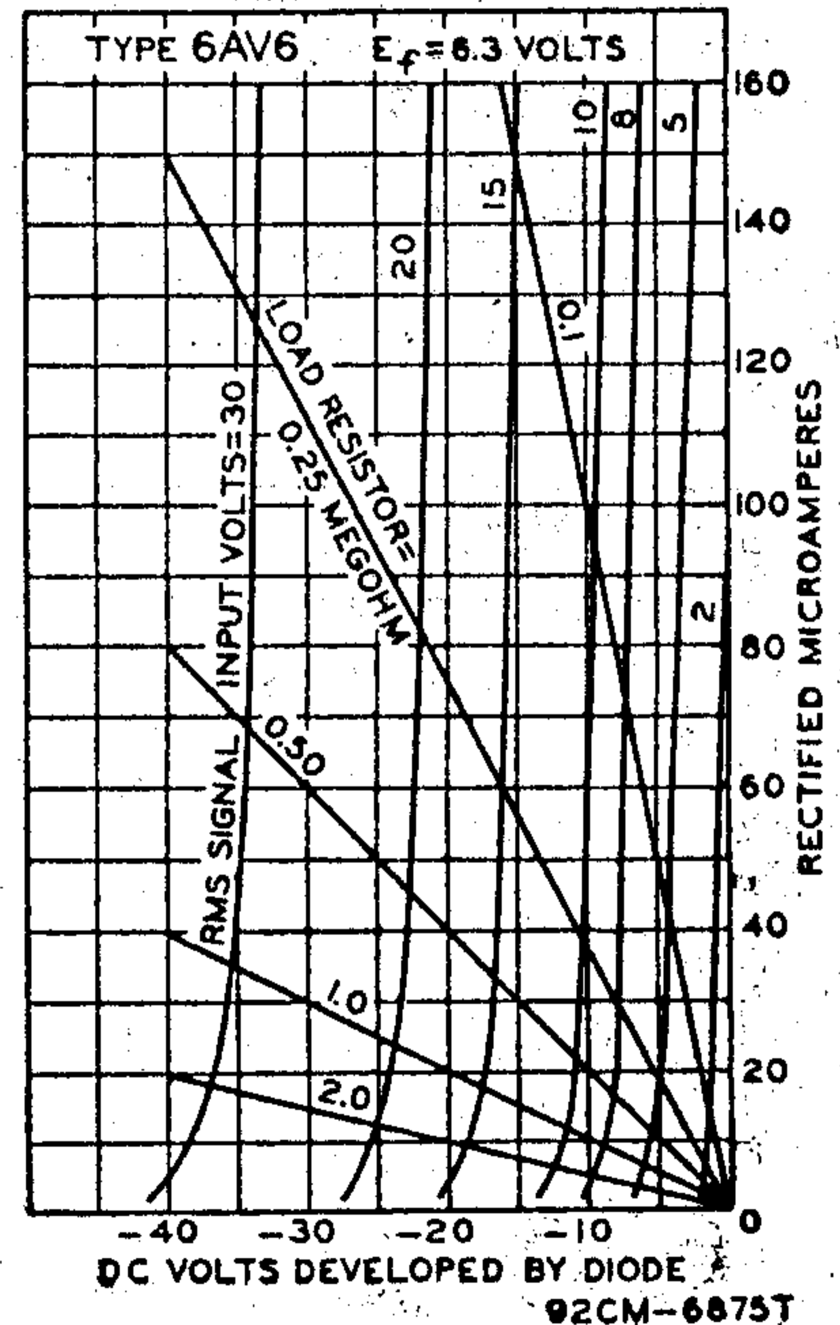
AVERAGE DIODE CHARACTERISTICS HALF-WAVE RECTIFICATION-SINGLE DIODE UNIT
