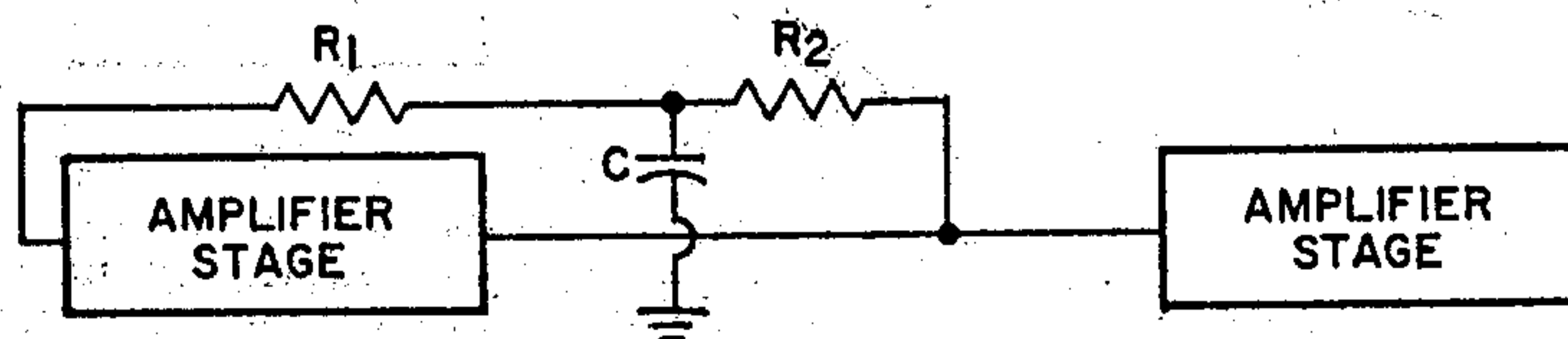
Fig. 55—Negative-feedback frequency-compensation network.
