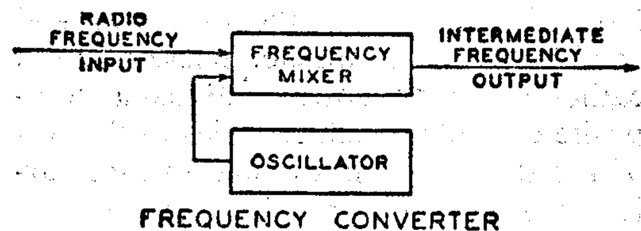
Fig. 106—Block diagram of simple frequency-converter circuit.
