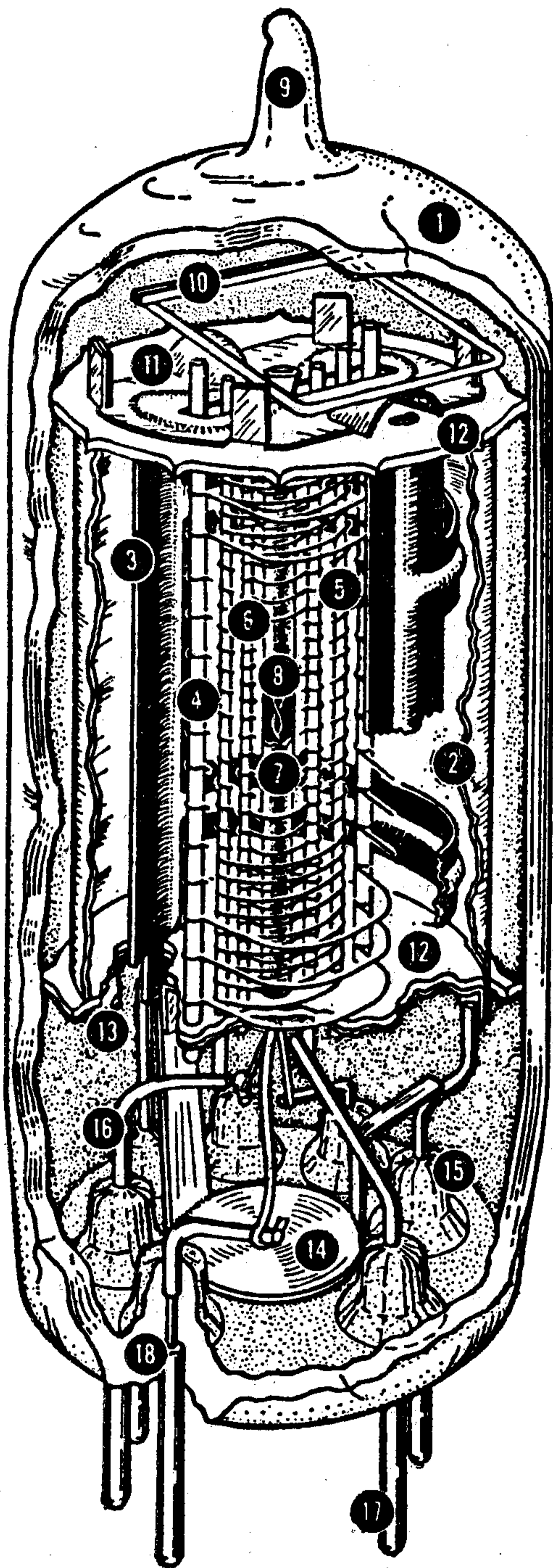
Structure of a Miniature Tube
