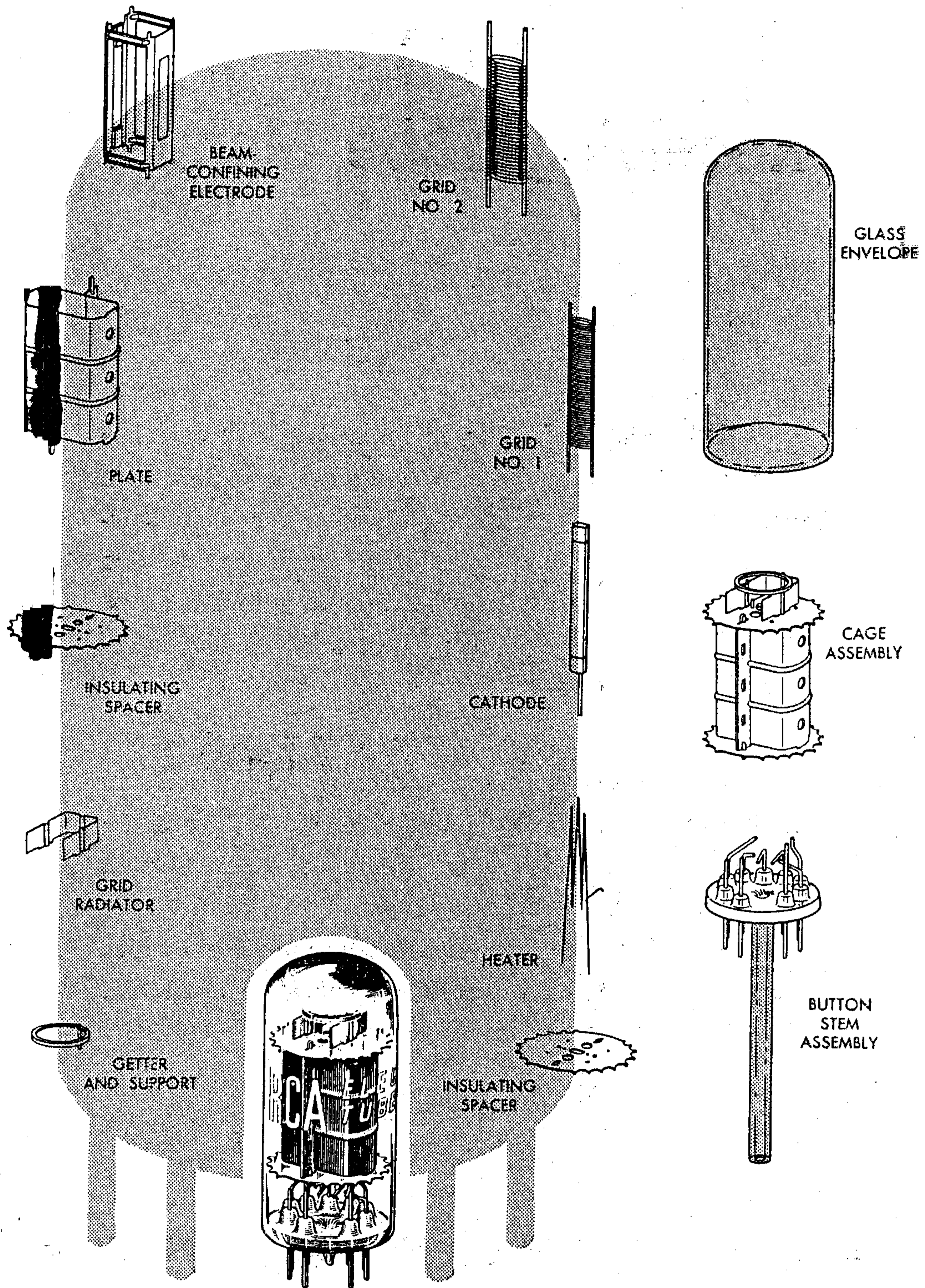
PARTS OF A NOVAR TUBE
