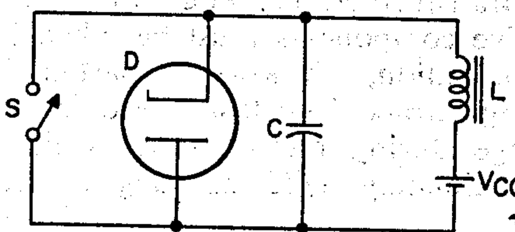
Fig. 88—Incorporation of damper diode.
