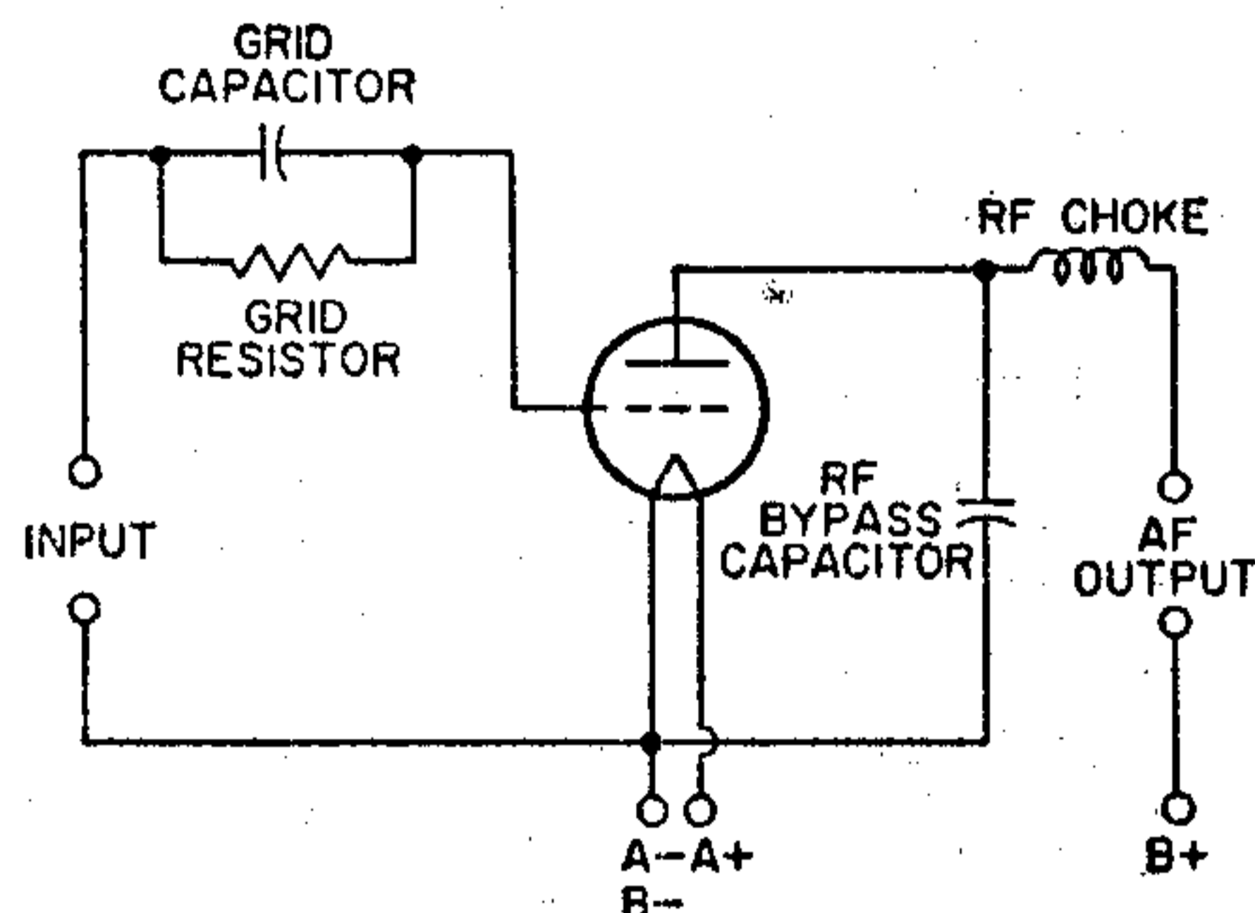
Fig. 27—Detector circuit using grid-resistor-and-capacitor bias.
