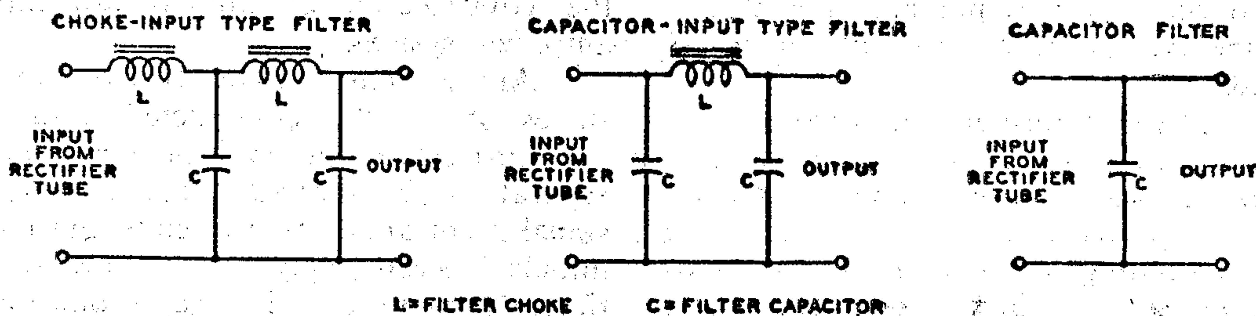
Fig. 121—Typical smoothing filters for rectifier tubes.
