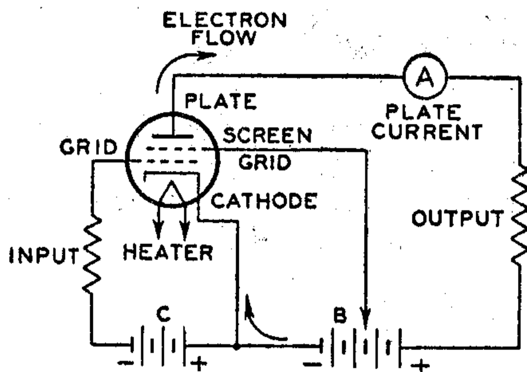
Fig. 7—Basic tetrode circuit.
