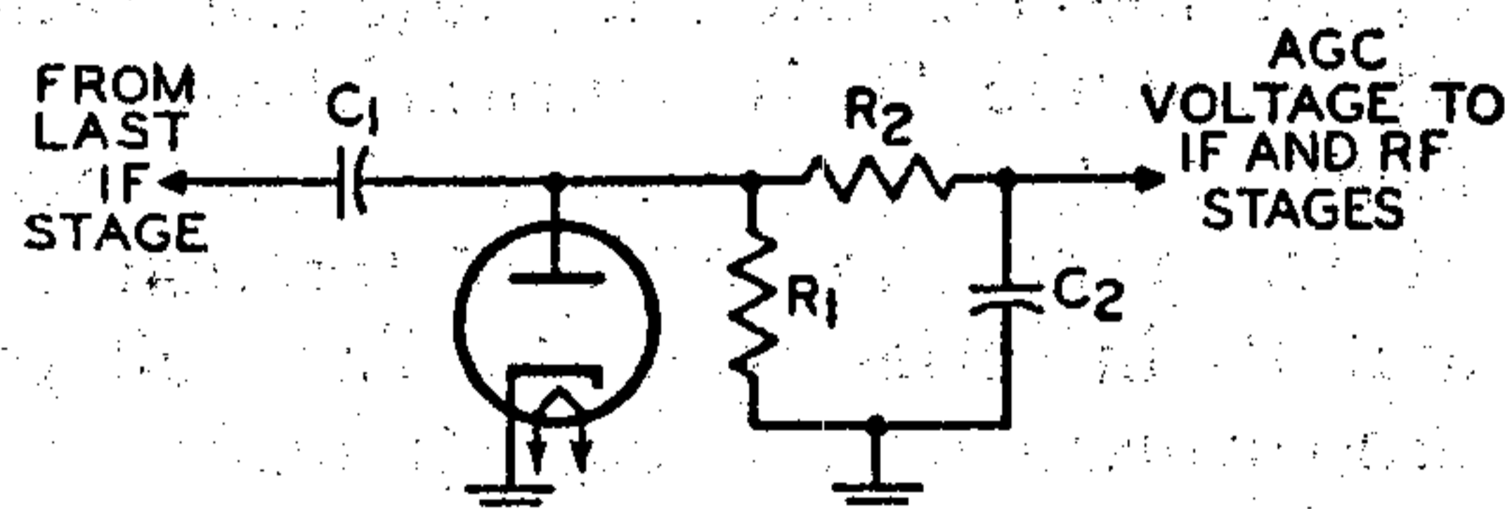
Fig. 63—Automatic-gain control (agc) circuit.
