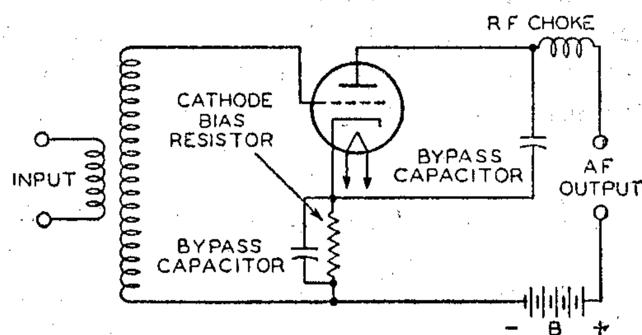
Fig. 26—Grid-bias detector circuit.
