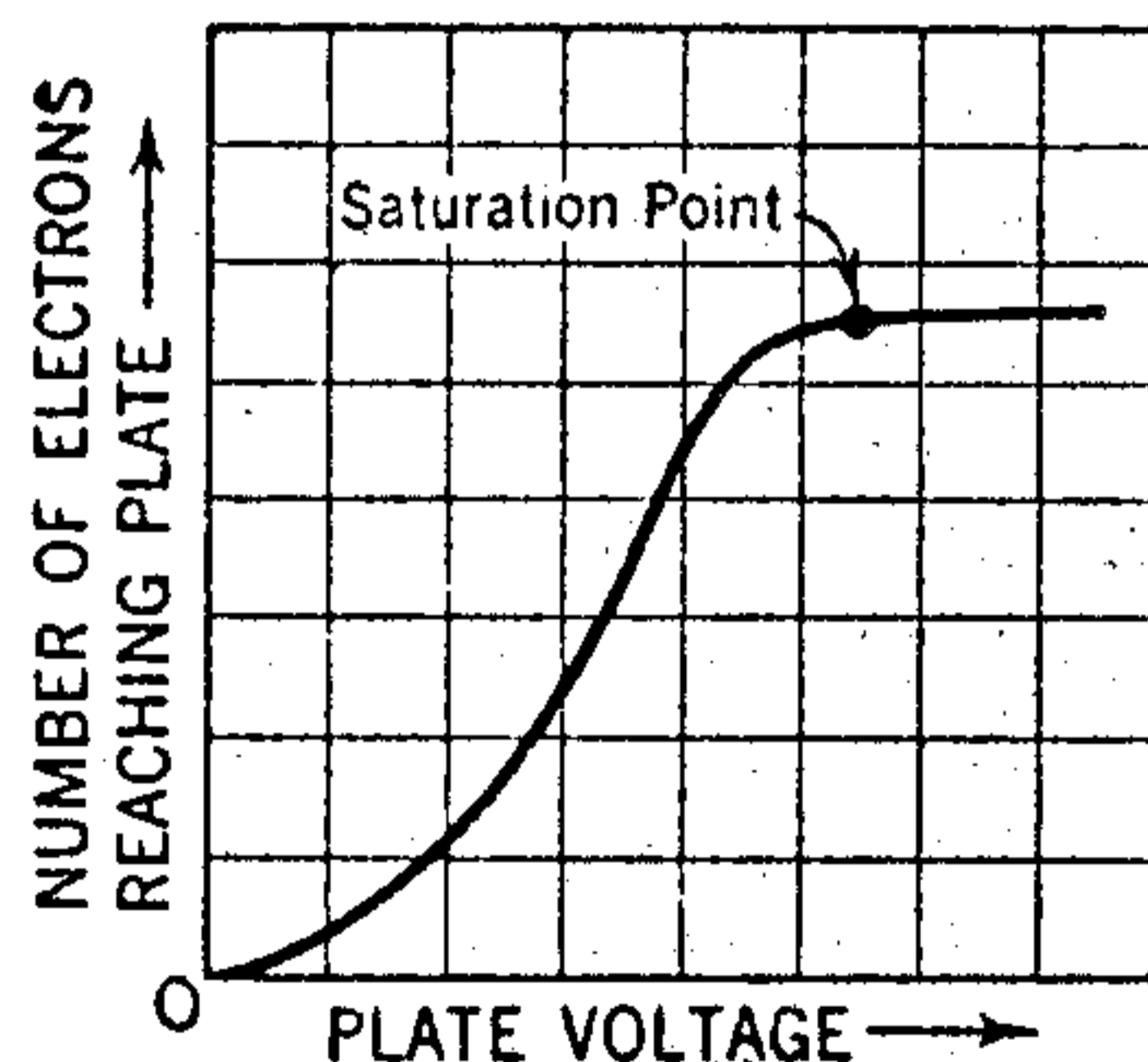
Fig. 5—Current characteristic of diode tube.
