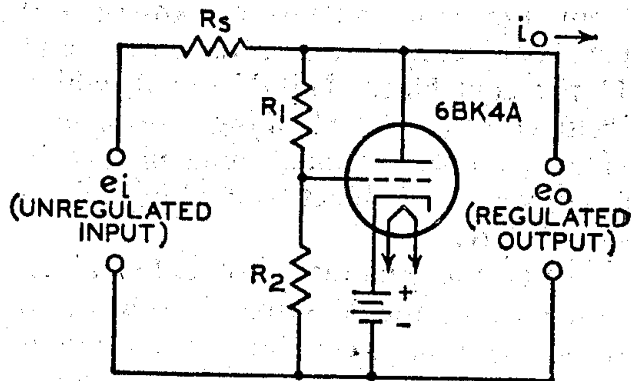
Fig. 92—High-voltage regulator circuit for color television.
