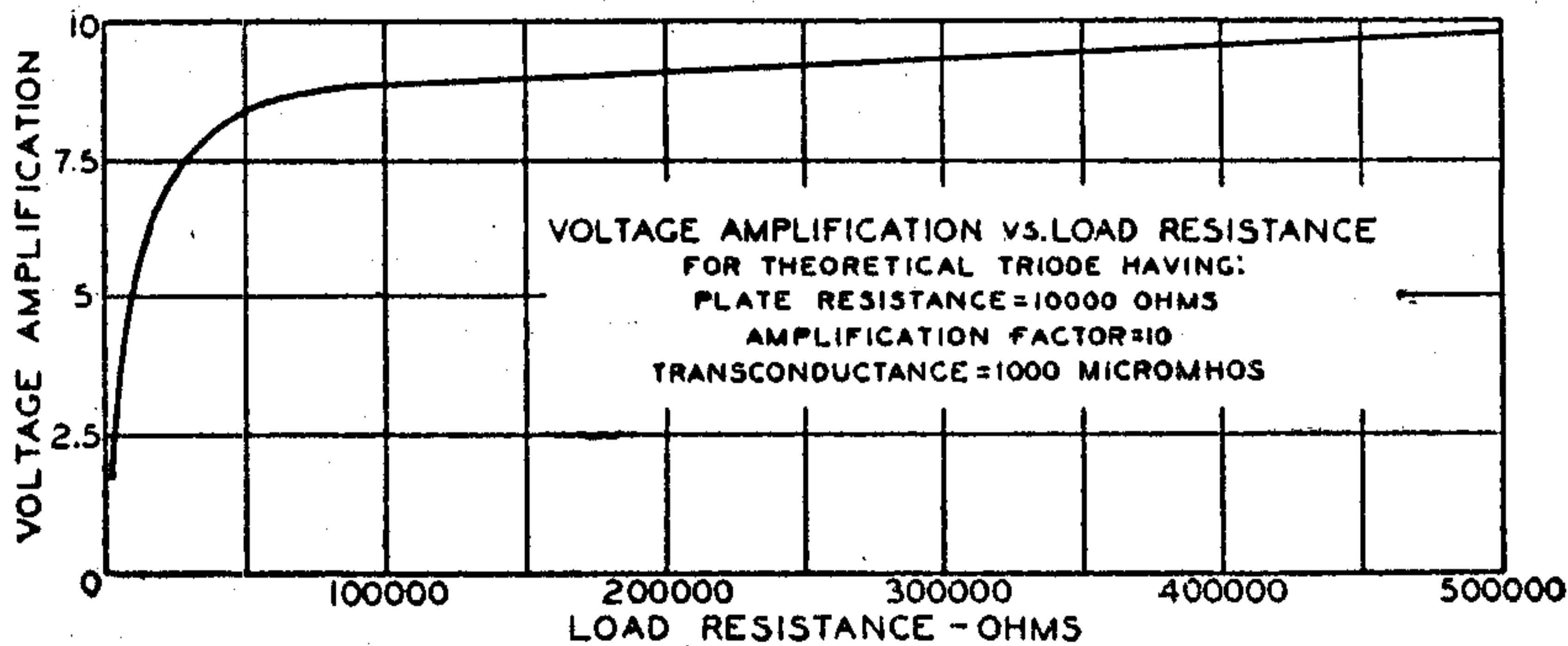
Fig. 36—Gain curve for triode amplifier circuit.
