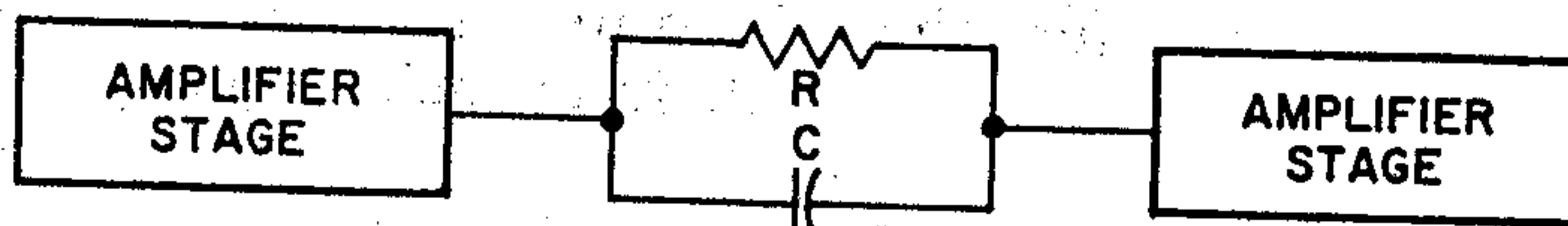
Fig. 54—Simple RC frequency-compensation network.
