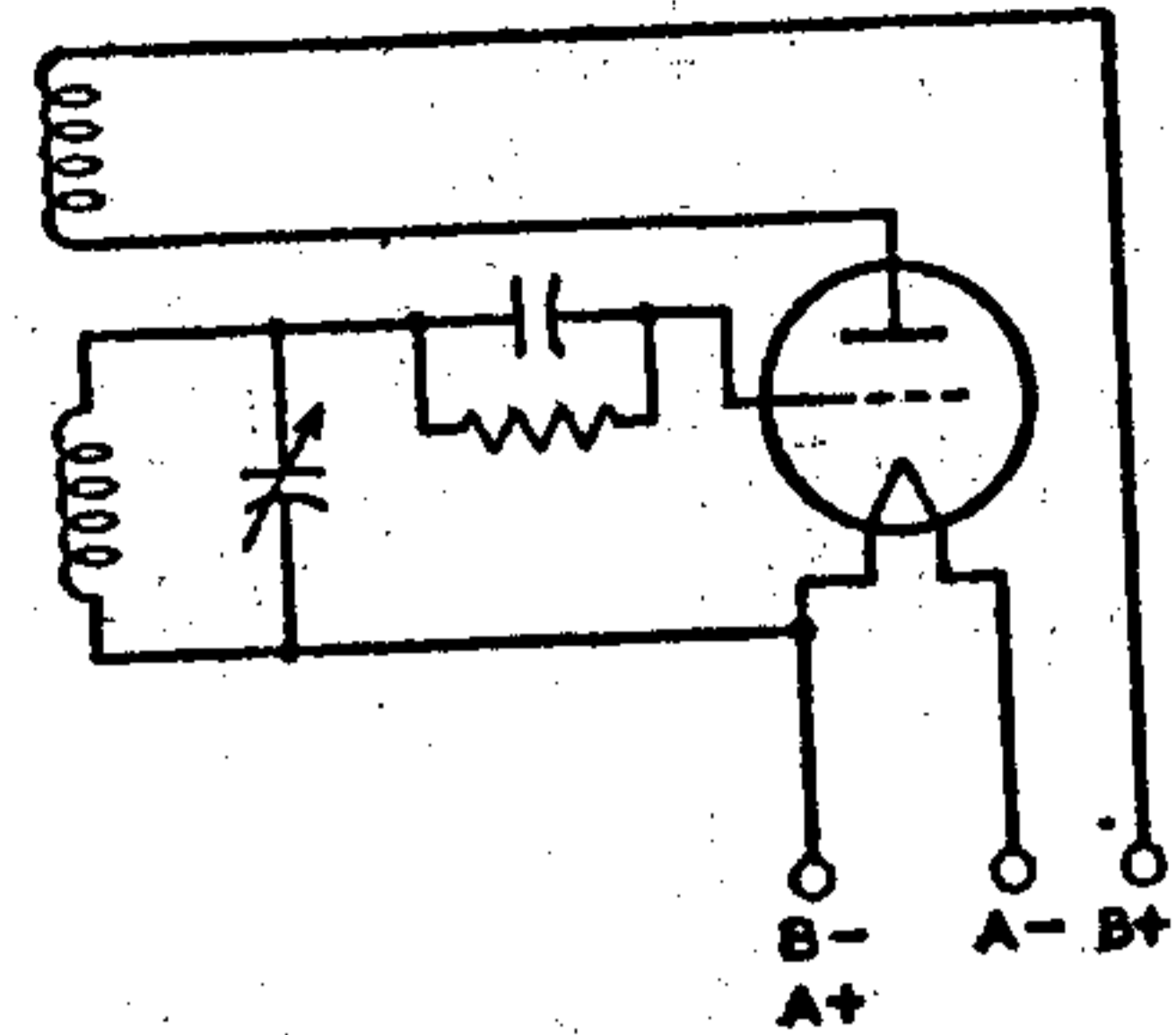
Fig. 98—Tuned-grid triode oscillator circuit using filament-type tube.
