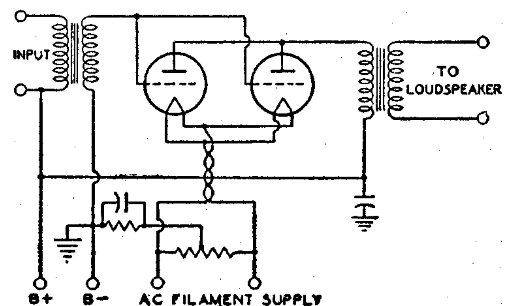
Fig. 39—Power amplifier with tubes connected in parallel.
