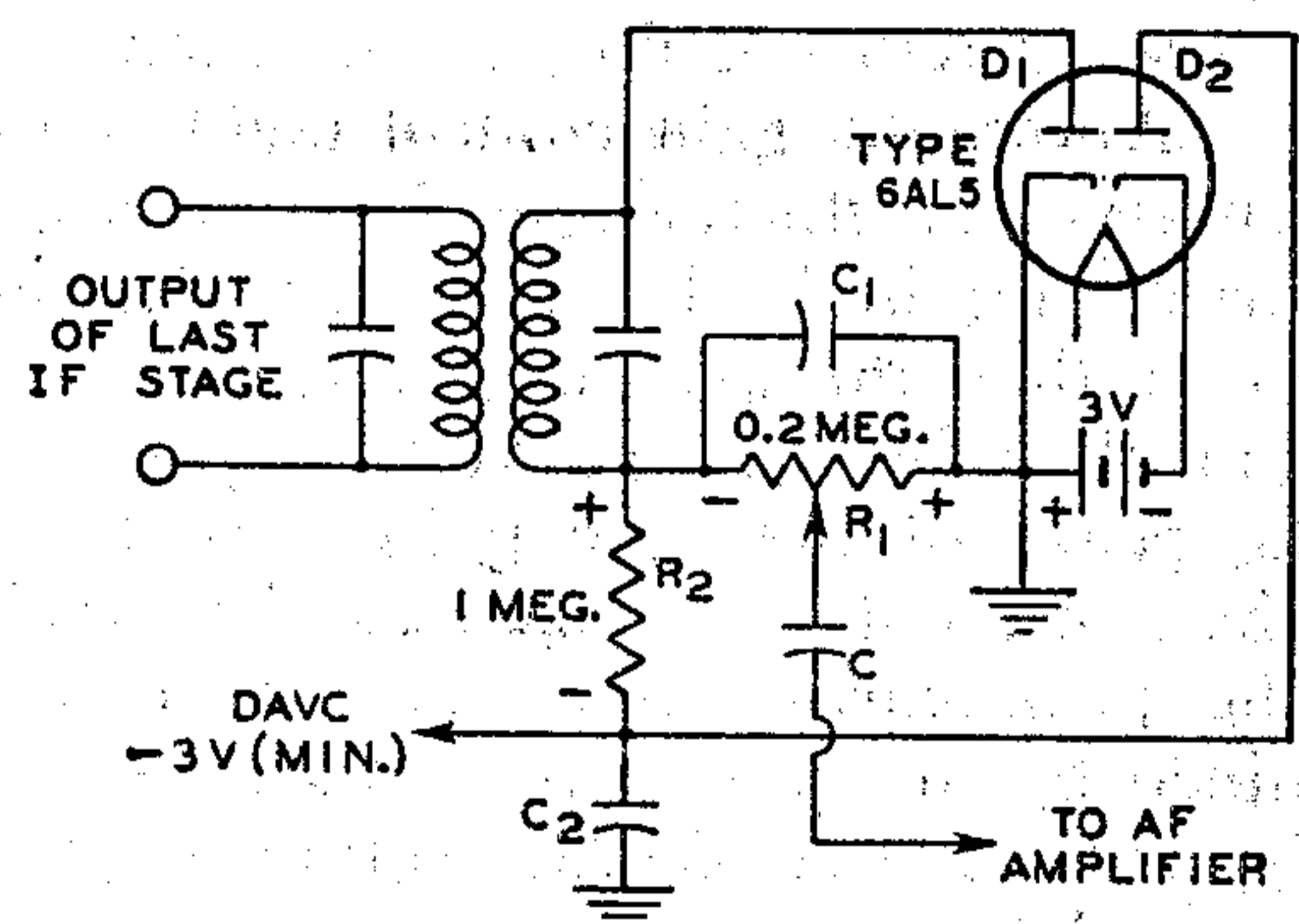
Fig. 62—Delayed avc (davc) circuit.
