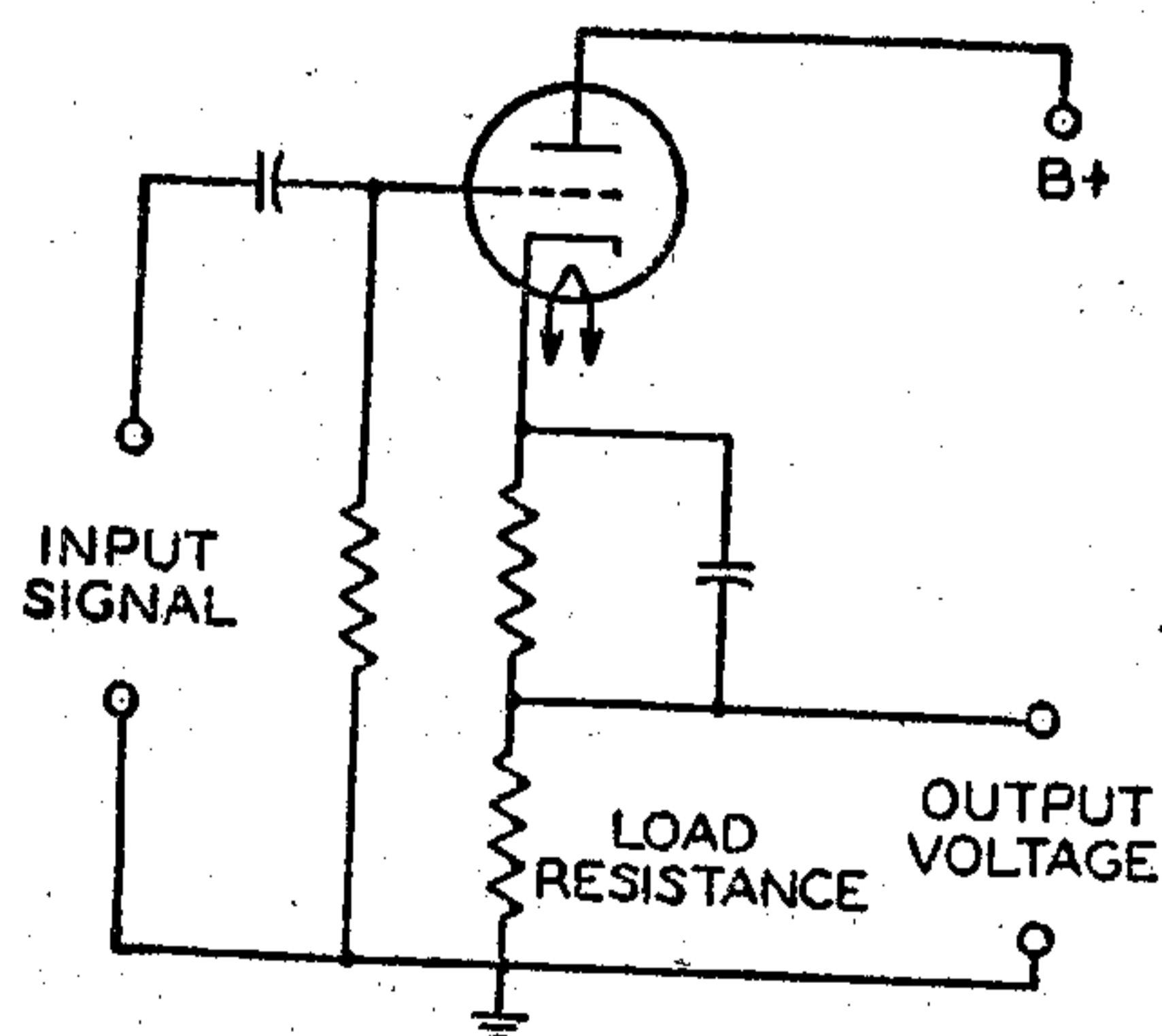
Fig. 52—Cathode-follower circuit modified for increased bias.
