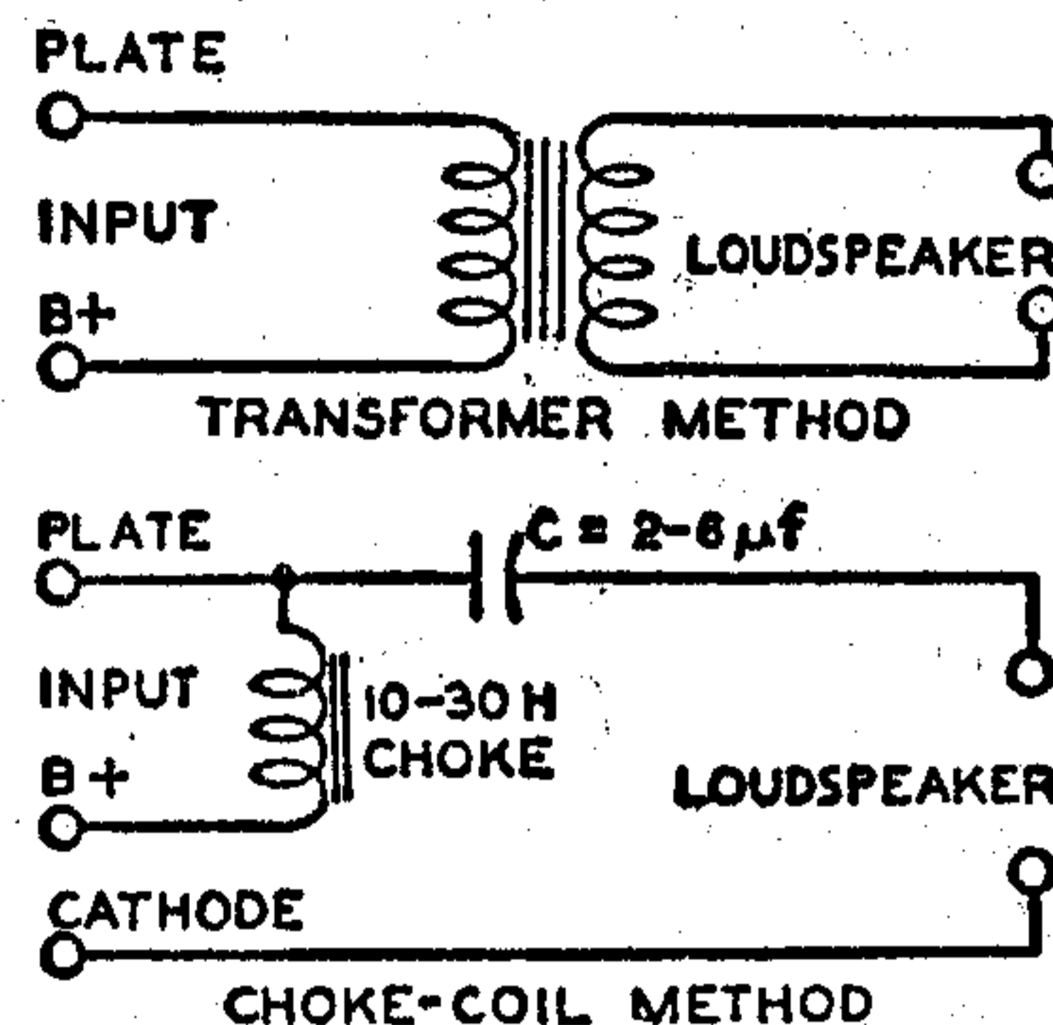
Fig. 123—Typical output-coupling devices.
