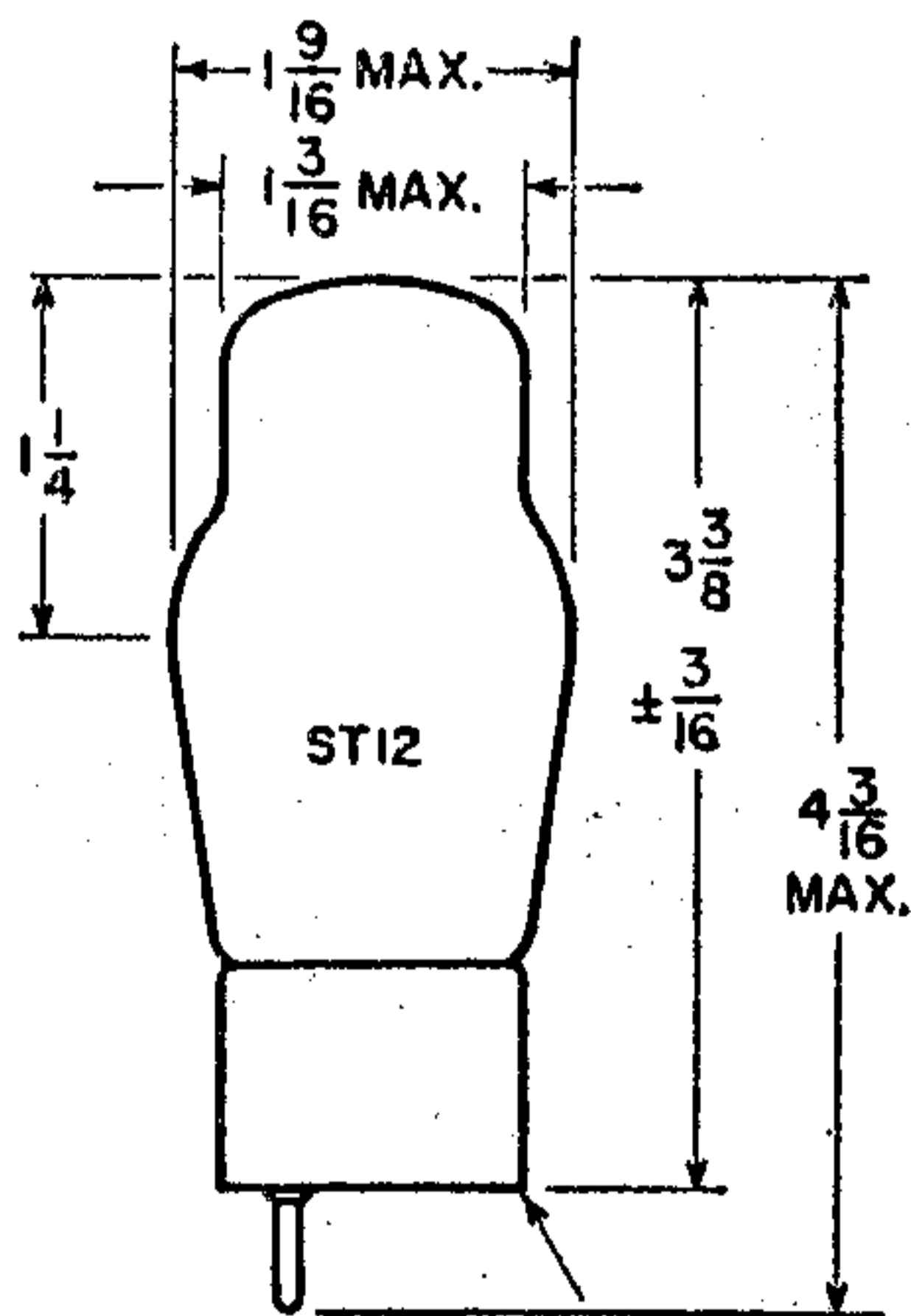
OCTAL OR SMALL-SHELL SMALL 4-, 5-, 6-, OR 7-PIN
