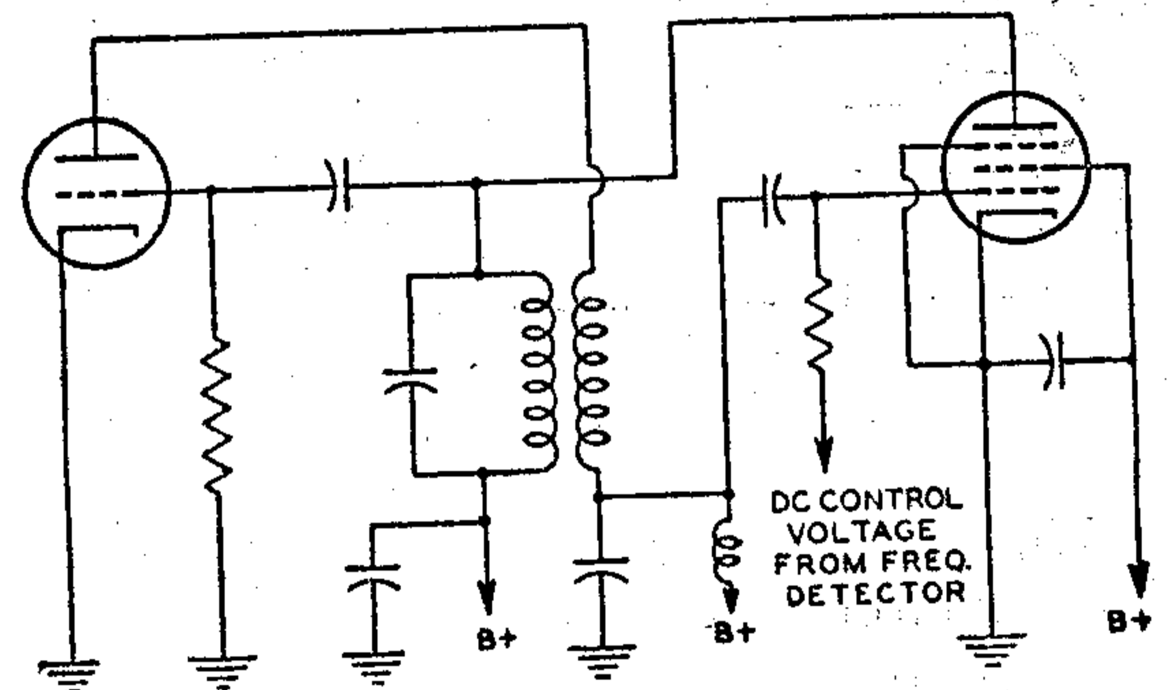
Fig. 104—Automatic-frequency-control (afc) circuit.
