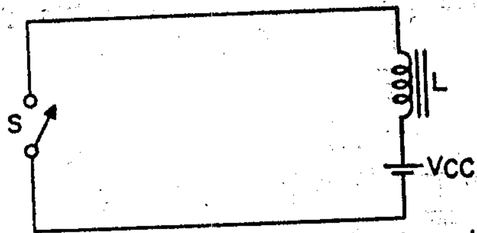
Fig. 85—Simplest form of deflection circuit.
