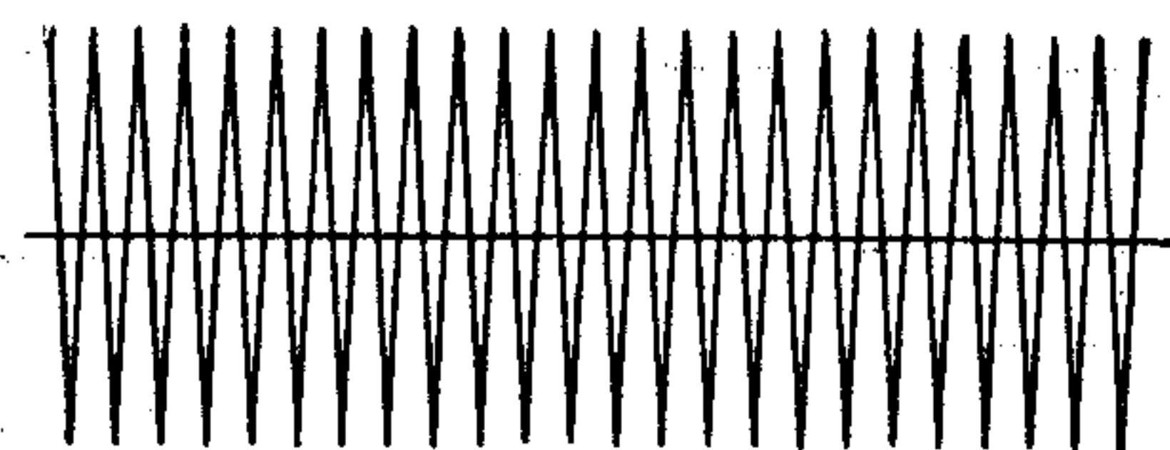
UNMODULATED RF CARRIER
