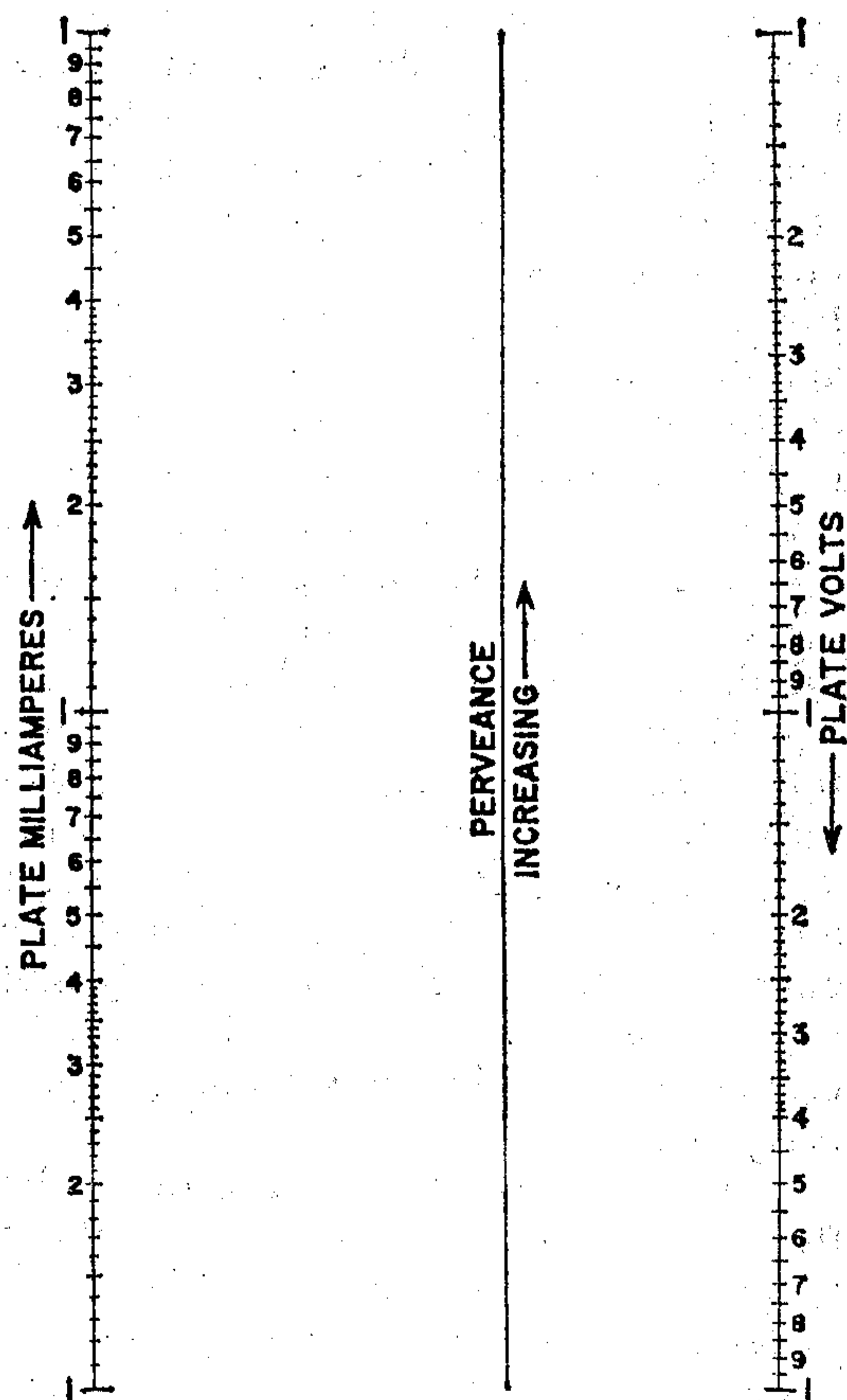
Fig. 125—Diode perveance nomograph.
