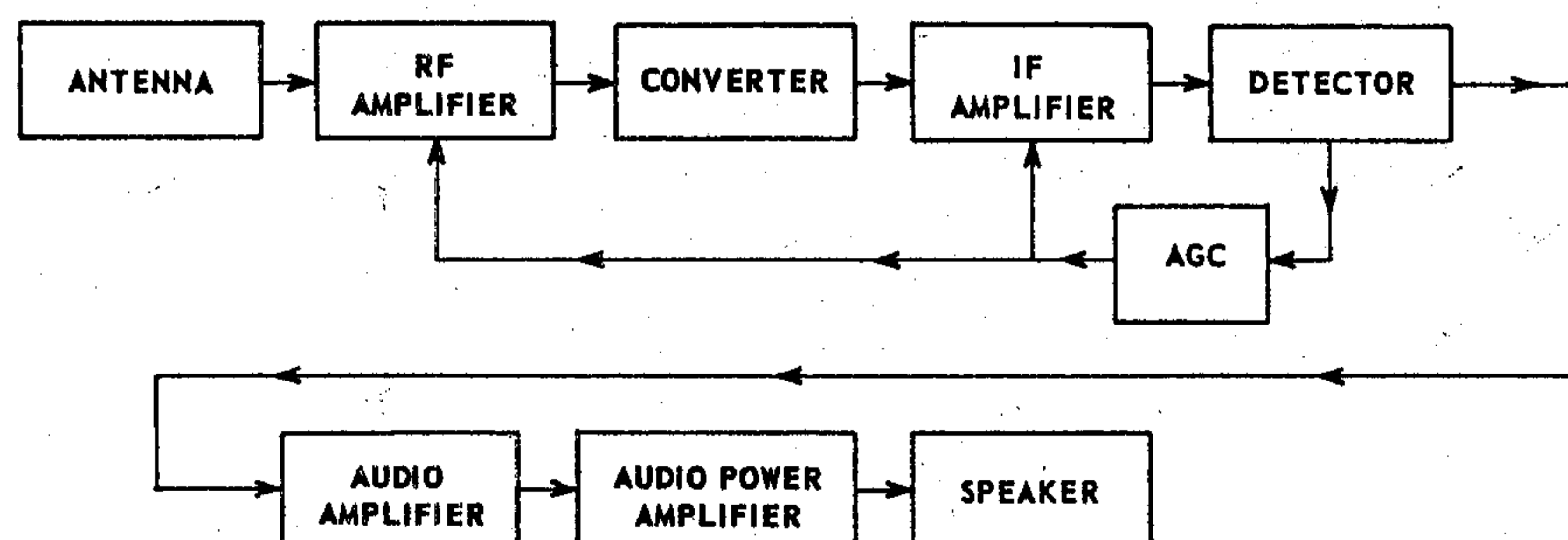
Fig. 14—Simplified block diagram for a broadcast-band receiver.
