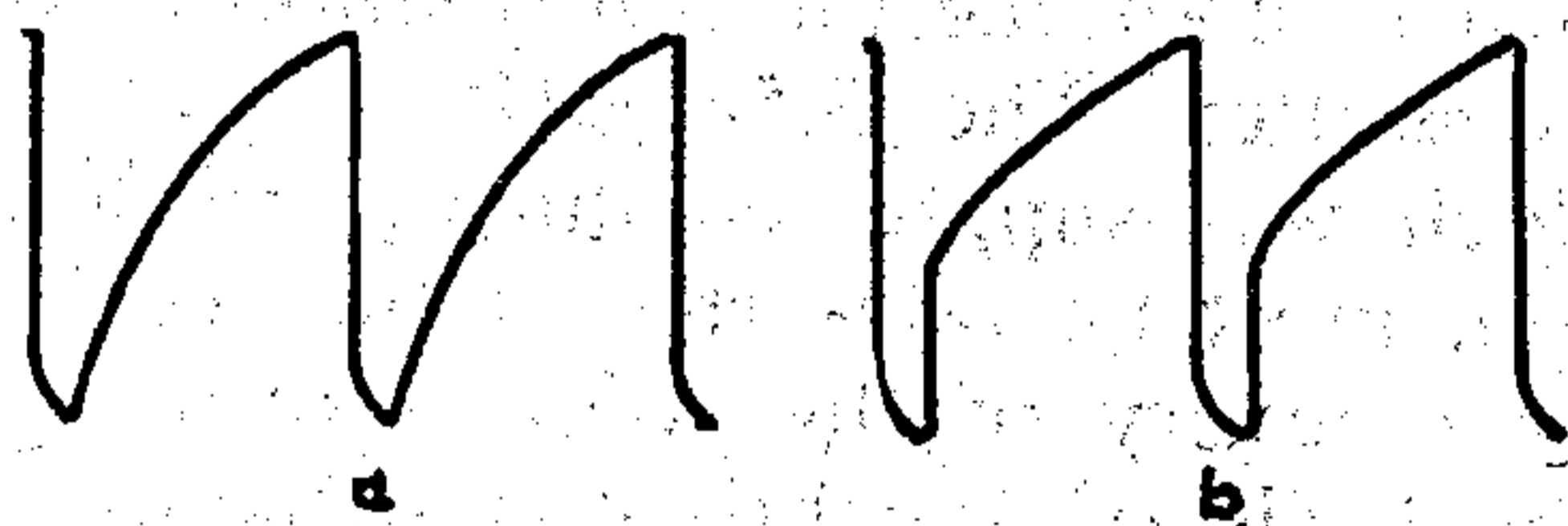
Fig. 91—Waveforms showing effect of R_2 in Fig. 90.
