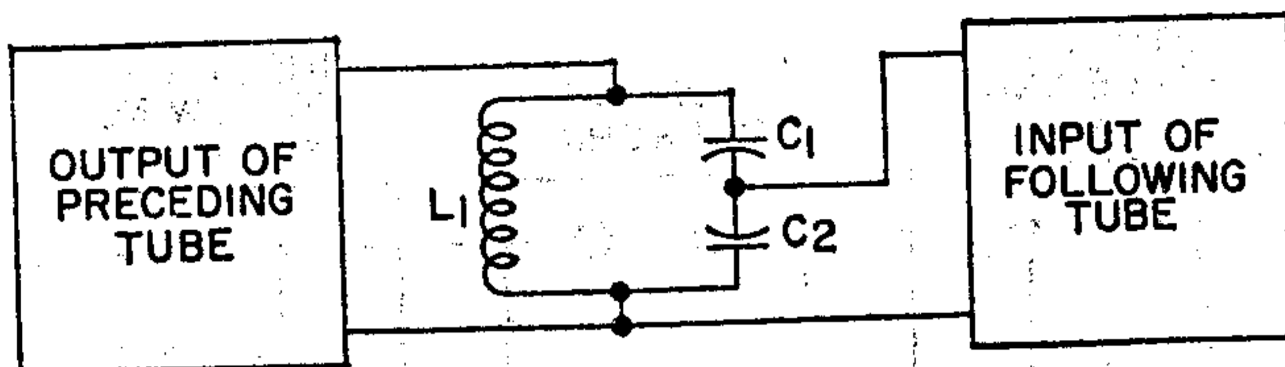
Fig. 71—Single-tuned coupling network using capacitive division.
