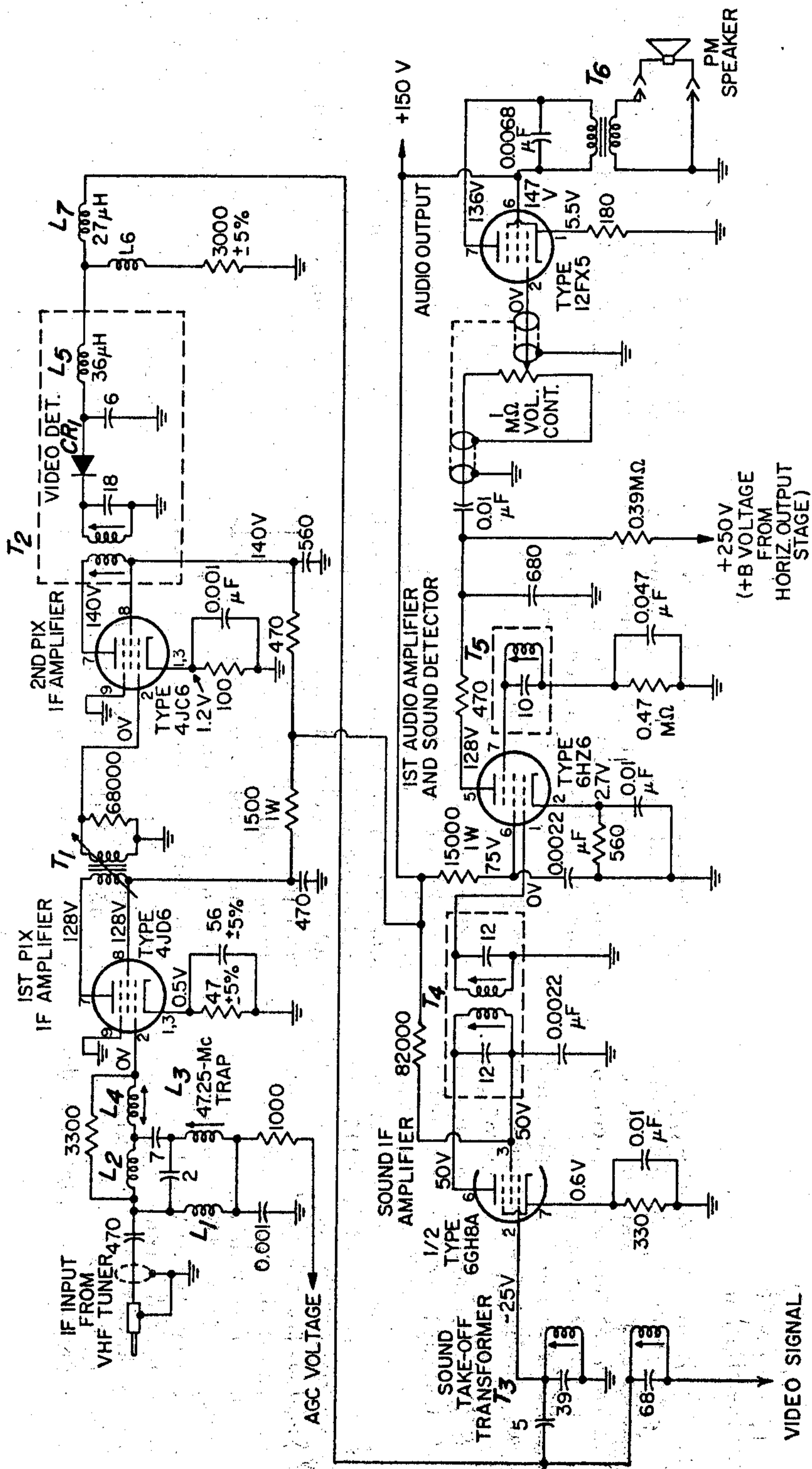
FIG. 25-27 VIDEO-IF AMPLIFIERS AND SOUND-CHANNEL CIRCUITS
