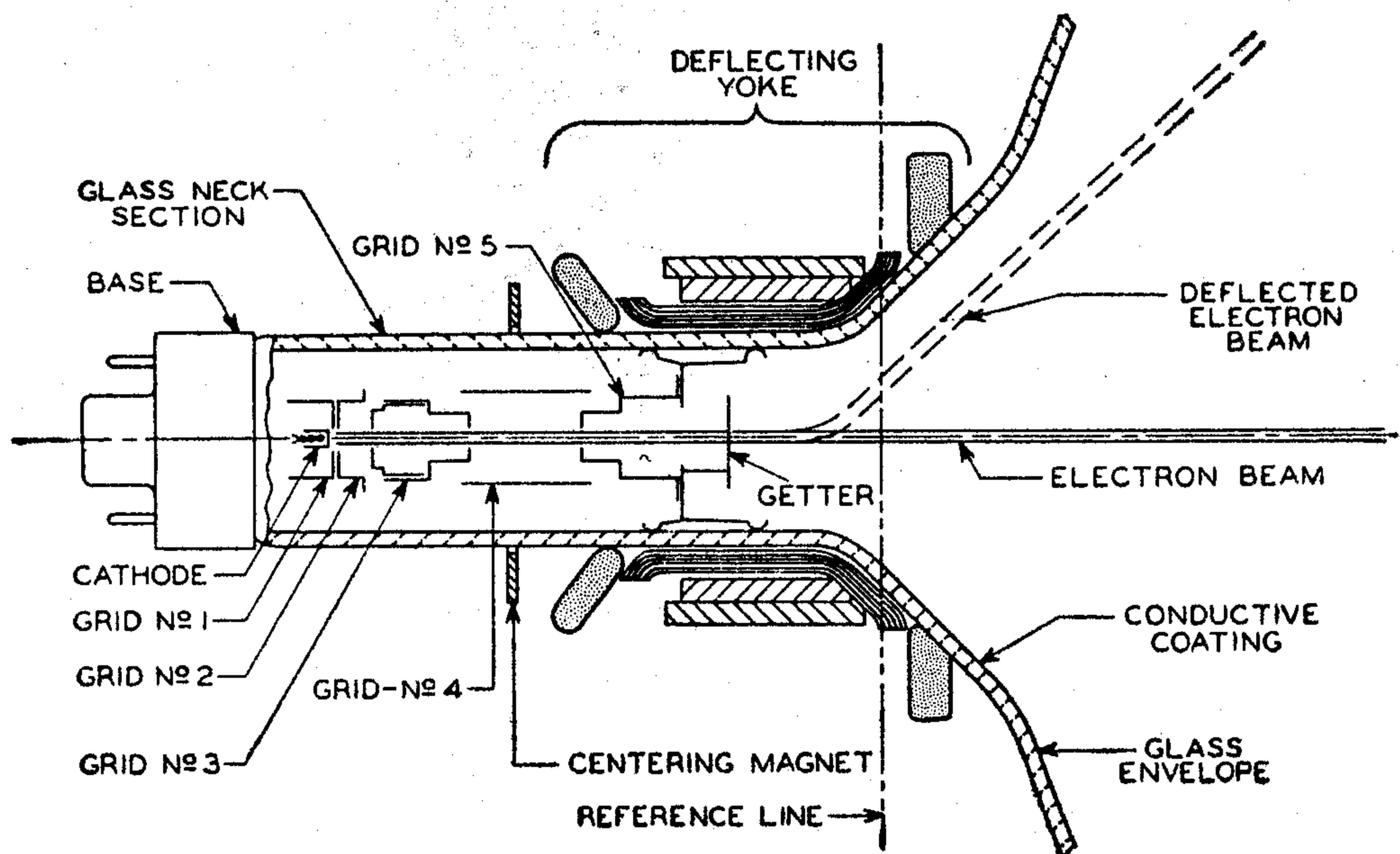
Fig. 10—Structure of television-picture-tube electron gun.
