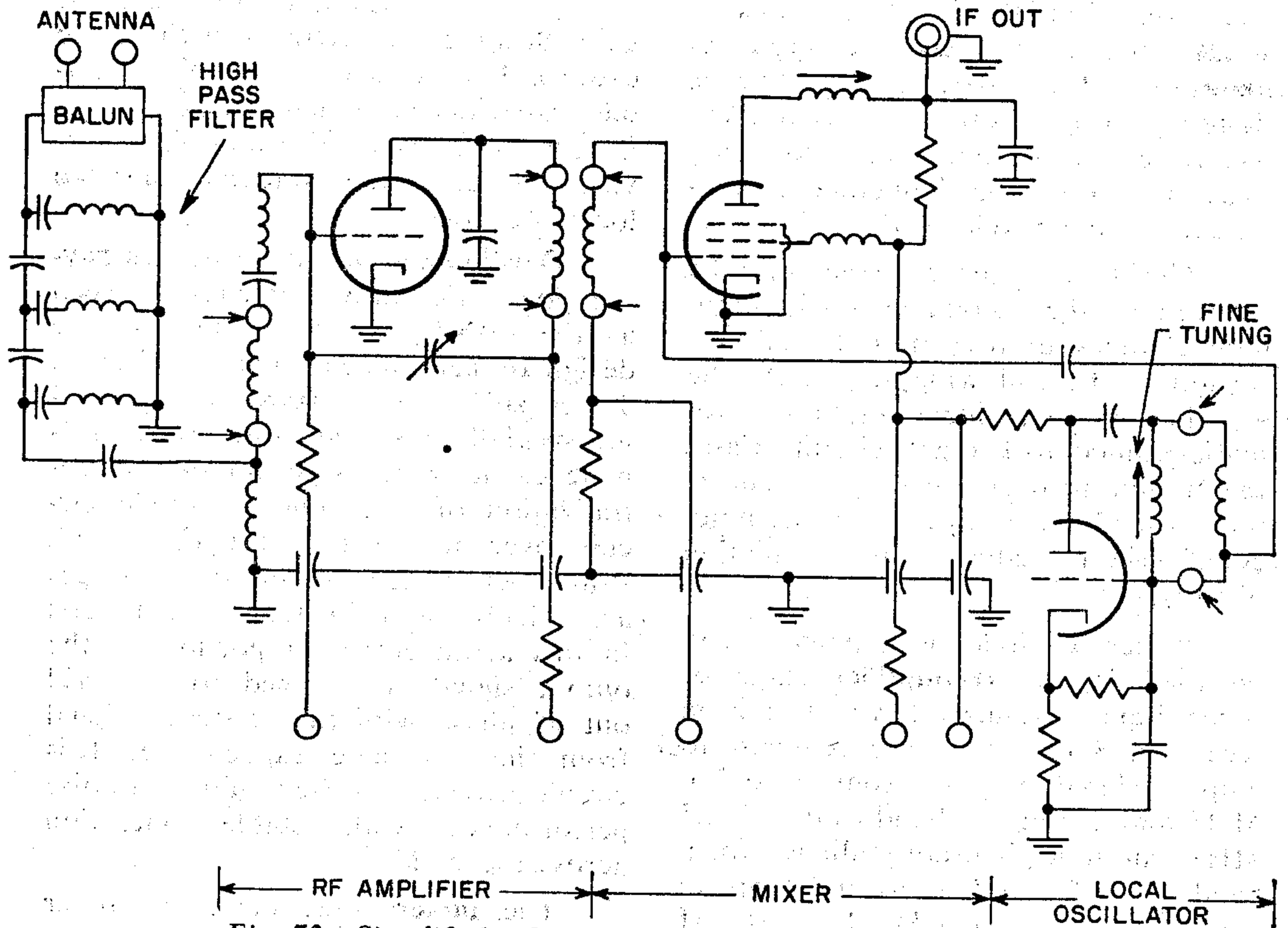
Fig. 72—Simplified schematic of typical vhf television tuner.
