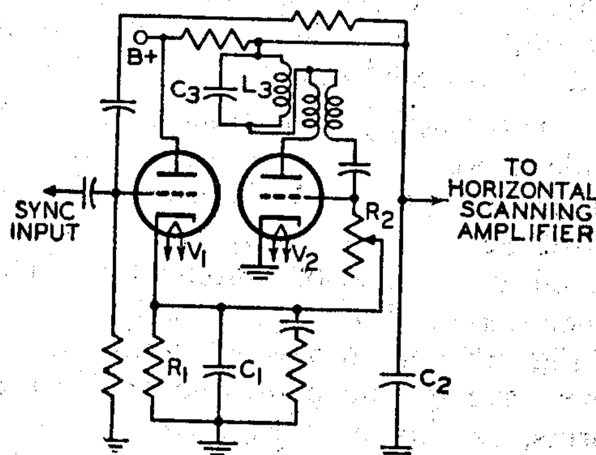
Fig. 101—Simplified synchroguide circuit.
