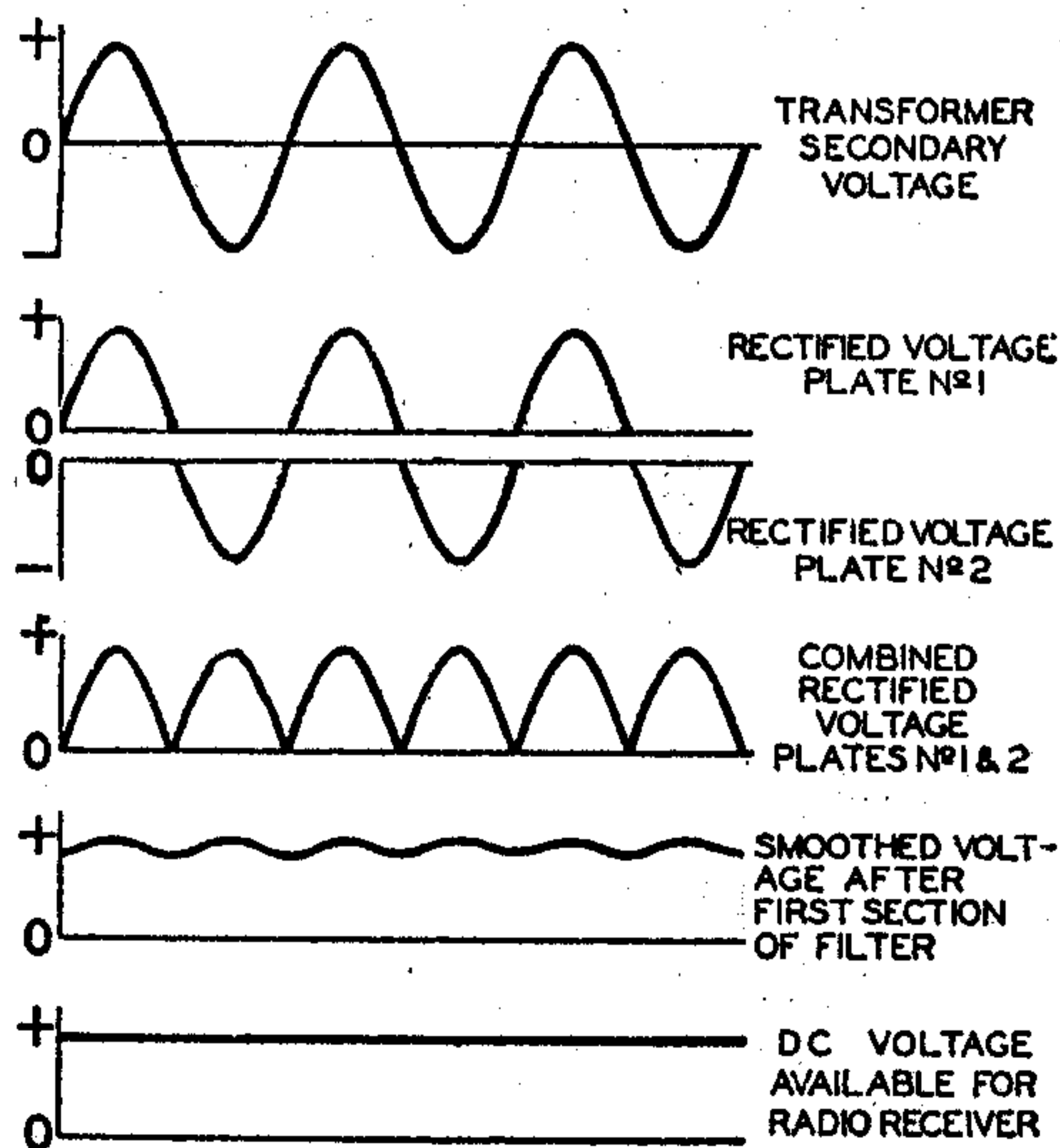
Fig. 17—Voltage waveforms of full-wave rectifier circuit.
