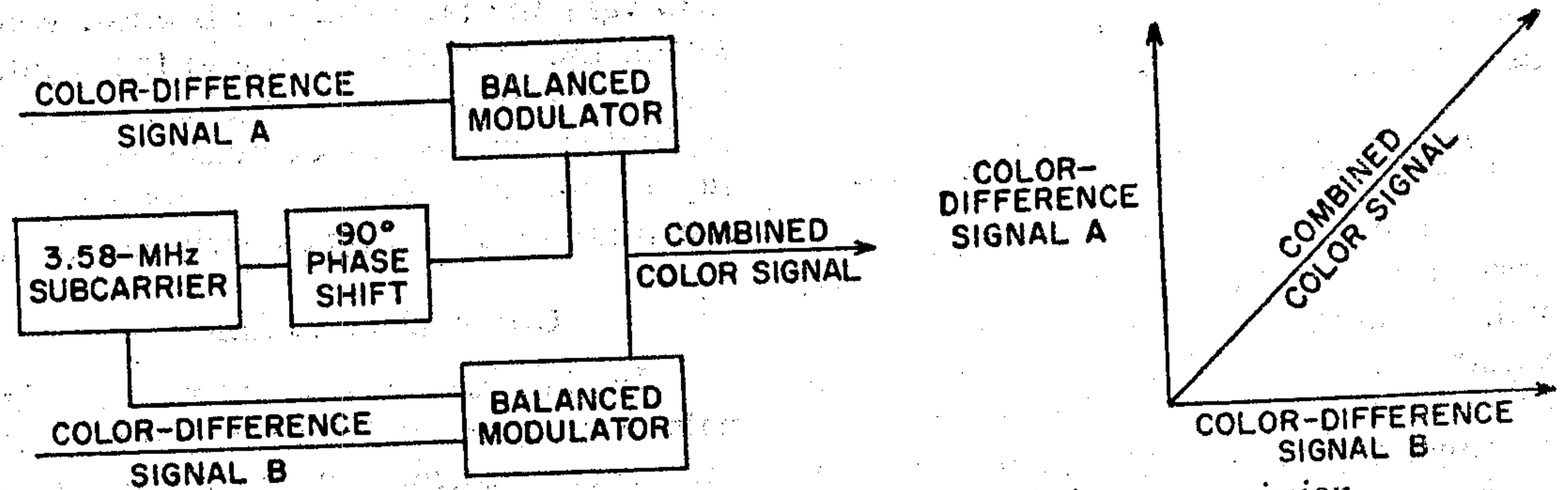
Fig. 93—Formation of combined color signal for transmission.
