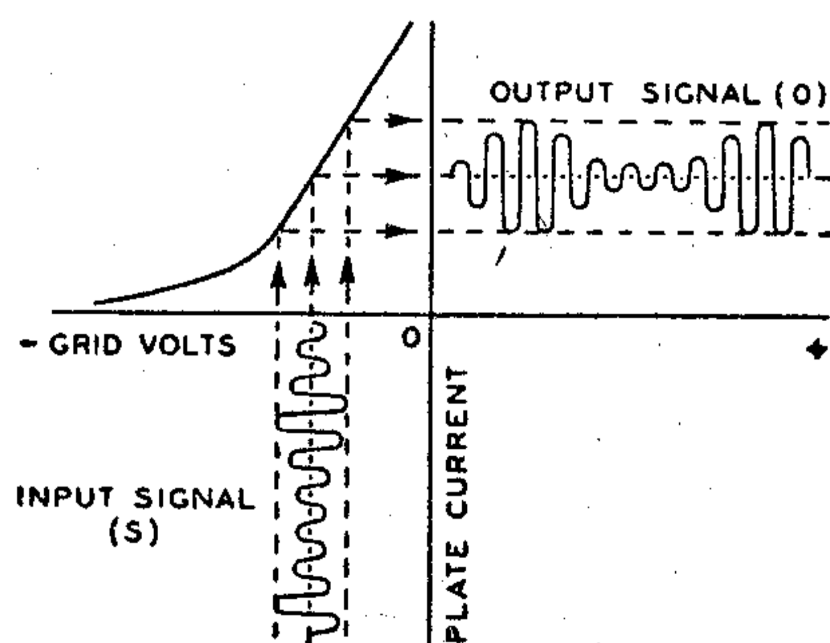
Fig. 34—Current characteristics of class A amplifier.
