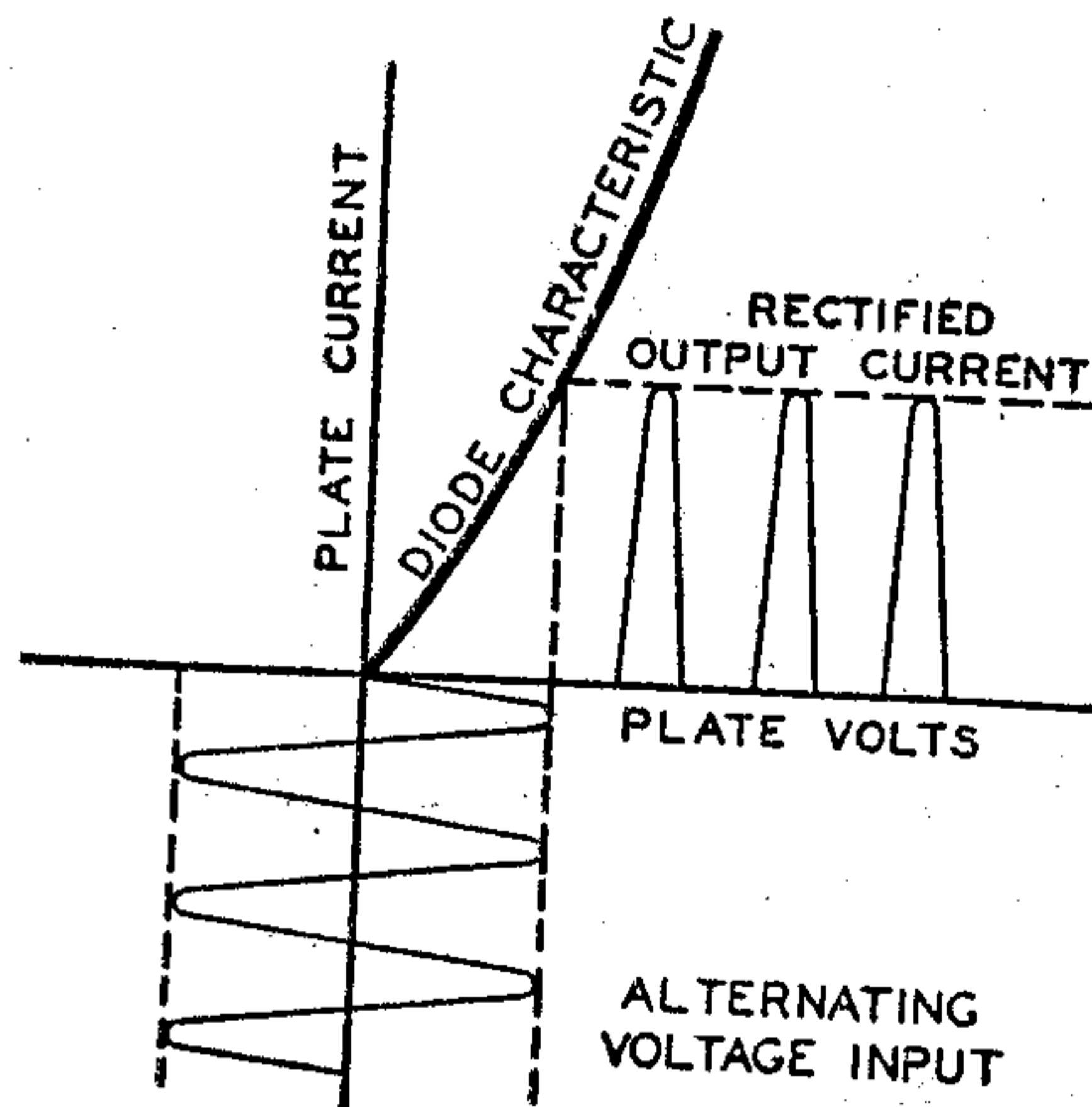
Fig. 4—Current characteristics of rectifier circuit.
