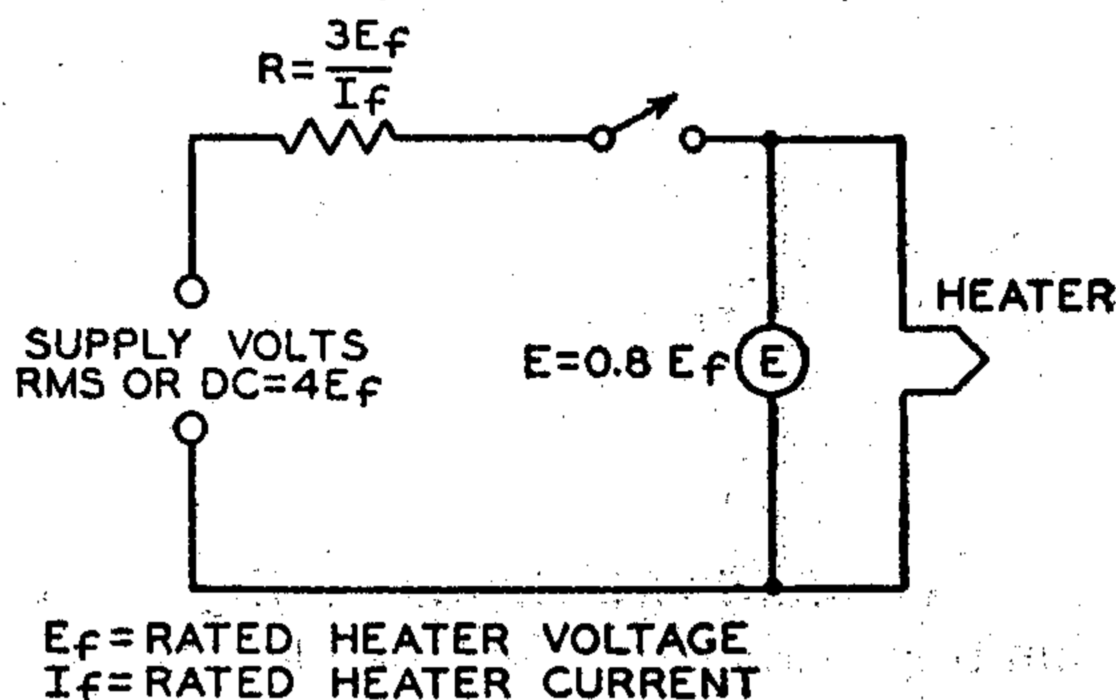
Fig. 124—Test circuit for measuring heater warm-up time.
