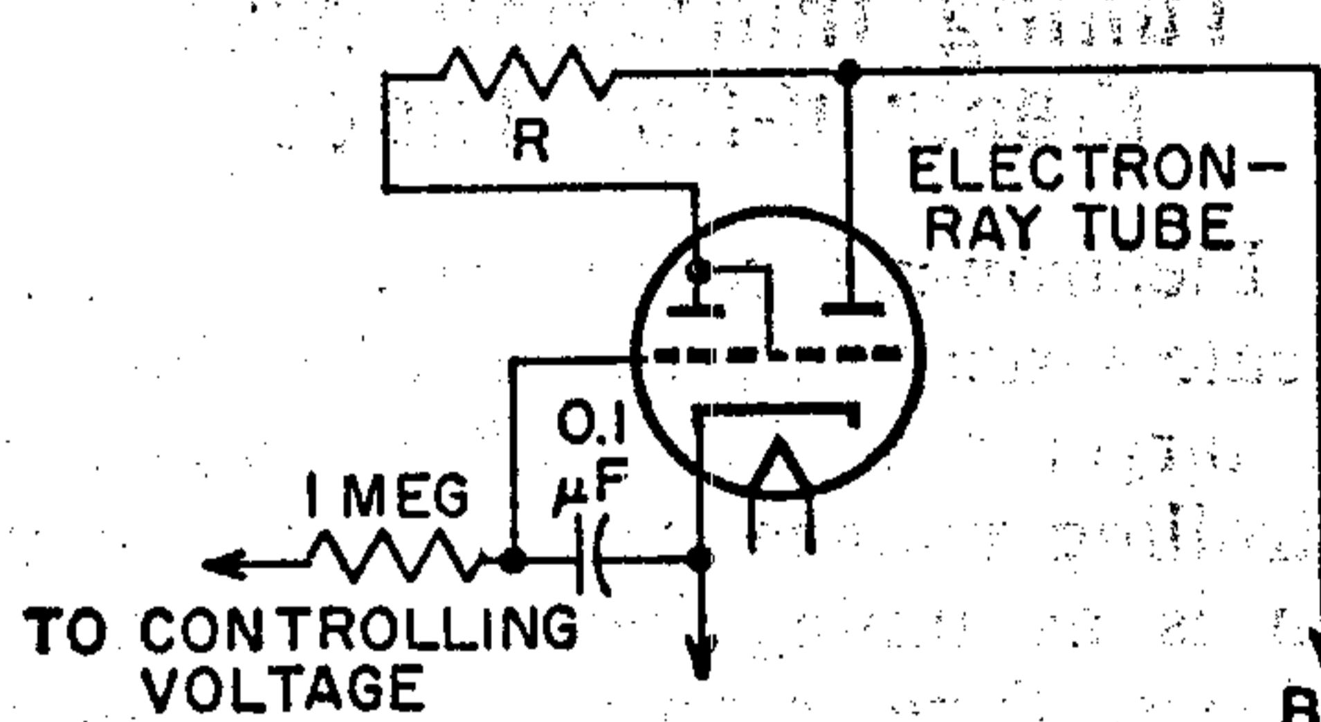
Fig. 110—Indicating circuit using an electron-ray tube.
