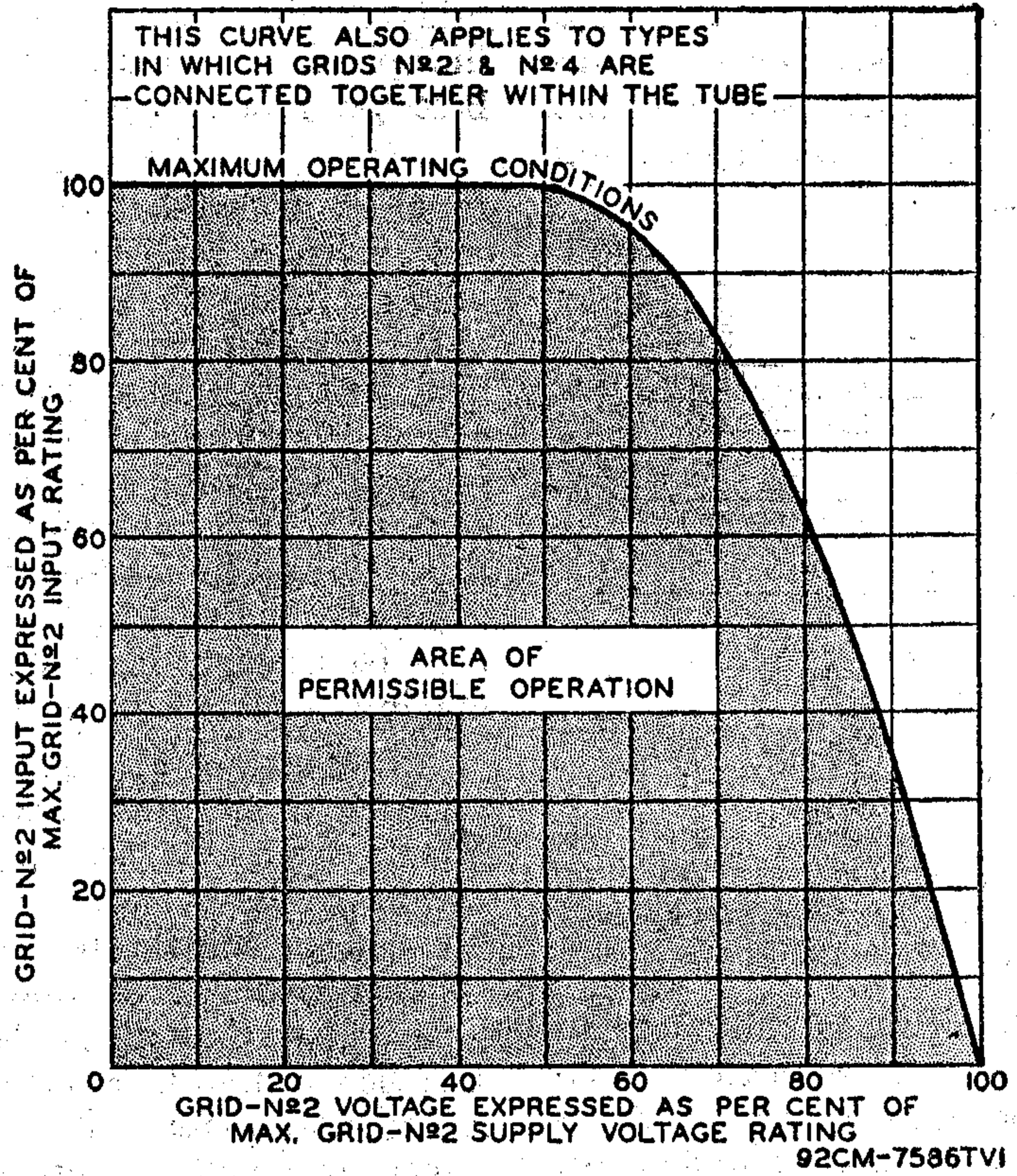
Fig. 128—Grid-No. 2 input rating curve.
