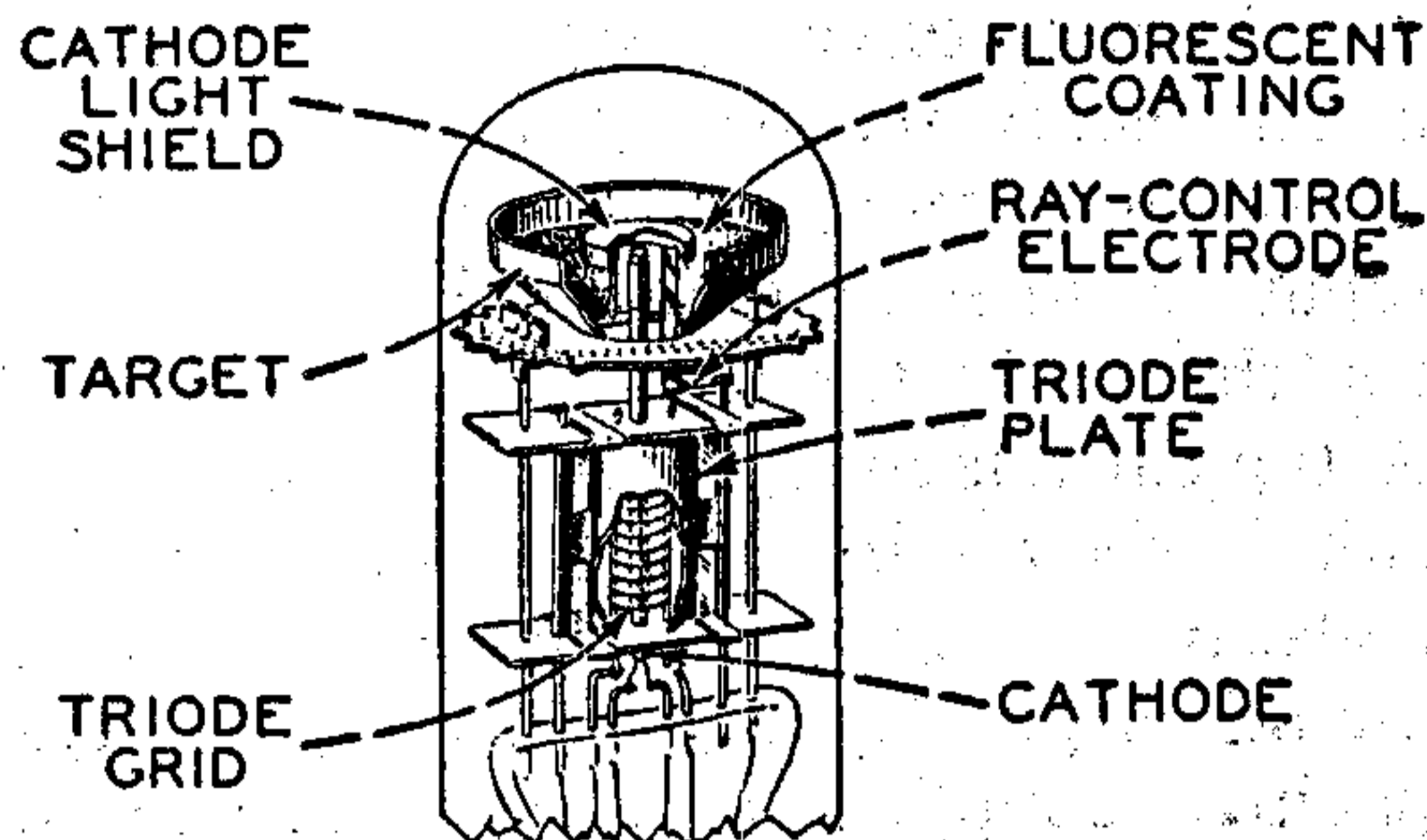
Fig. 109—Structure of electron-ray tube.
