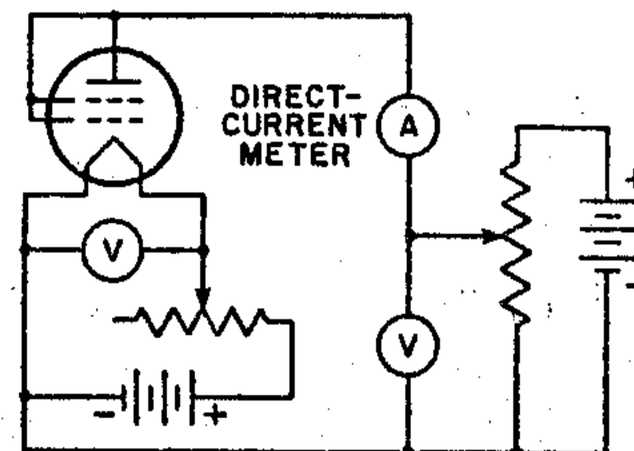
Fig. 130—Fundamental circuit of an emission tester
