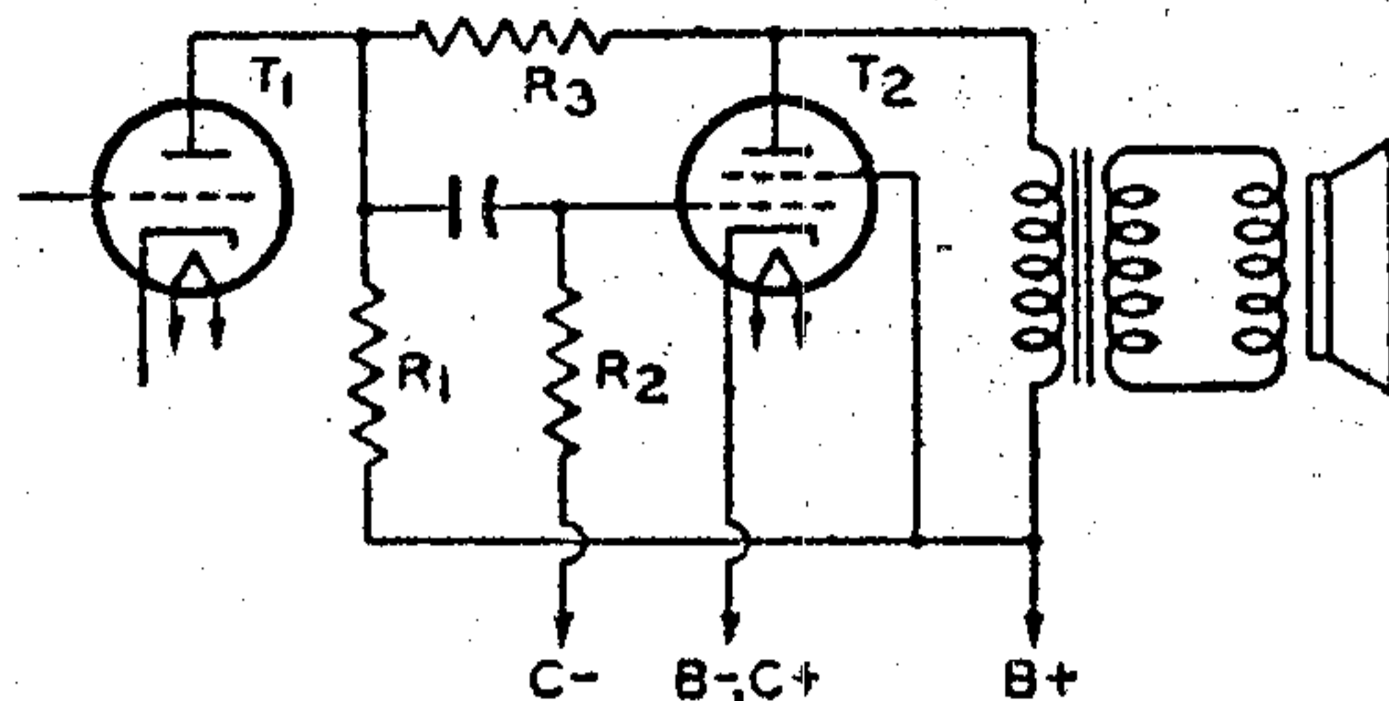
Fig. 50—Resistance-coupled stages using feedback resistor.
