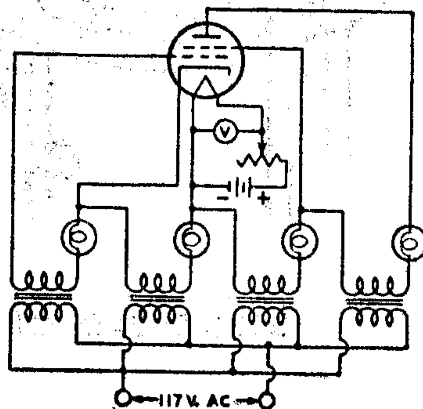
Fig. 129—Fundamental circuit of a short-circuit tester.
