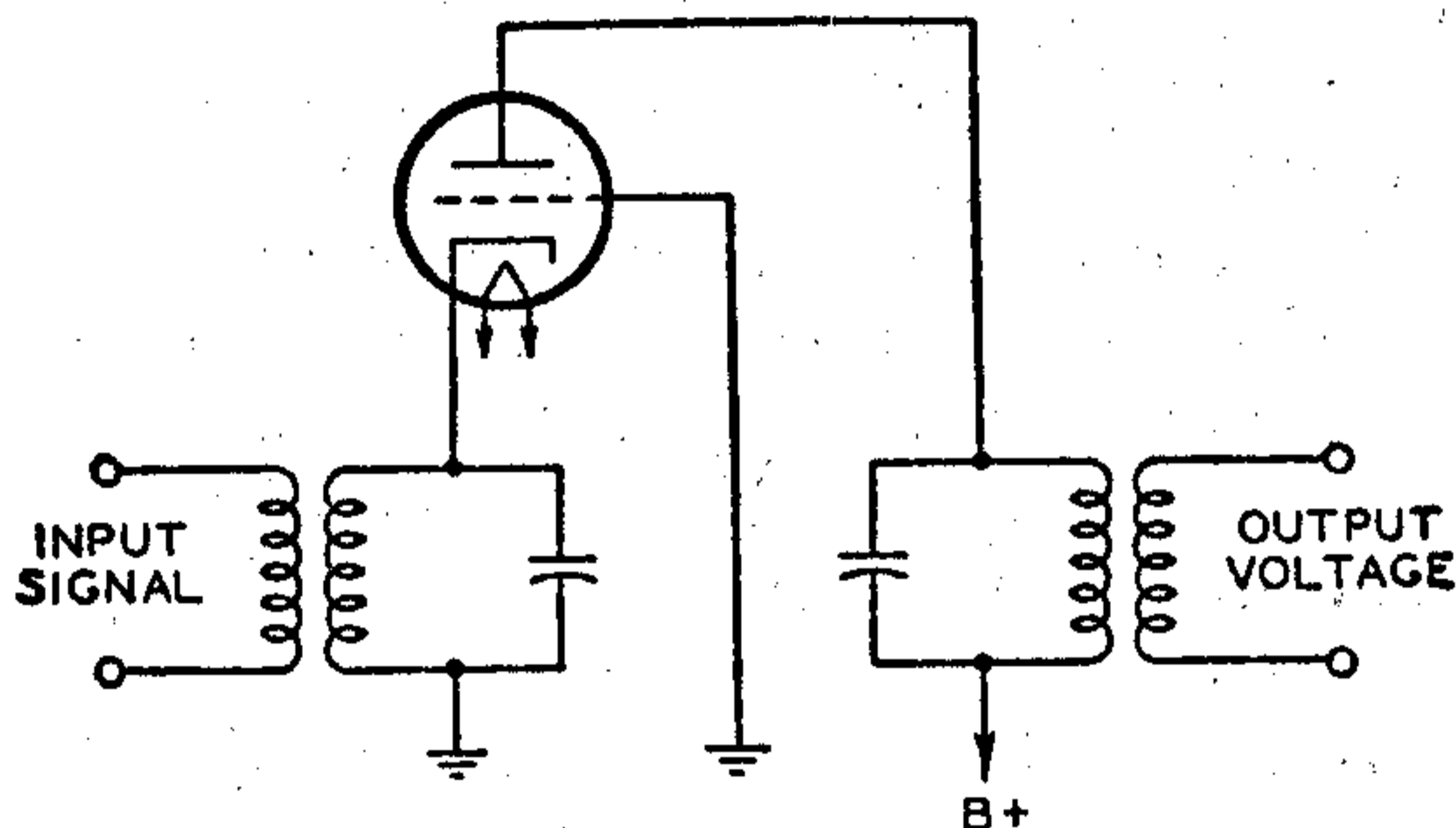
Fig. 47—Cathode-drive circuit.
