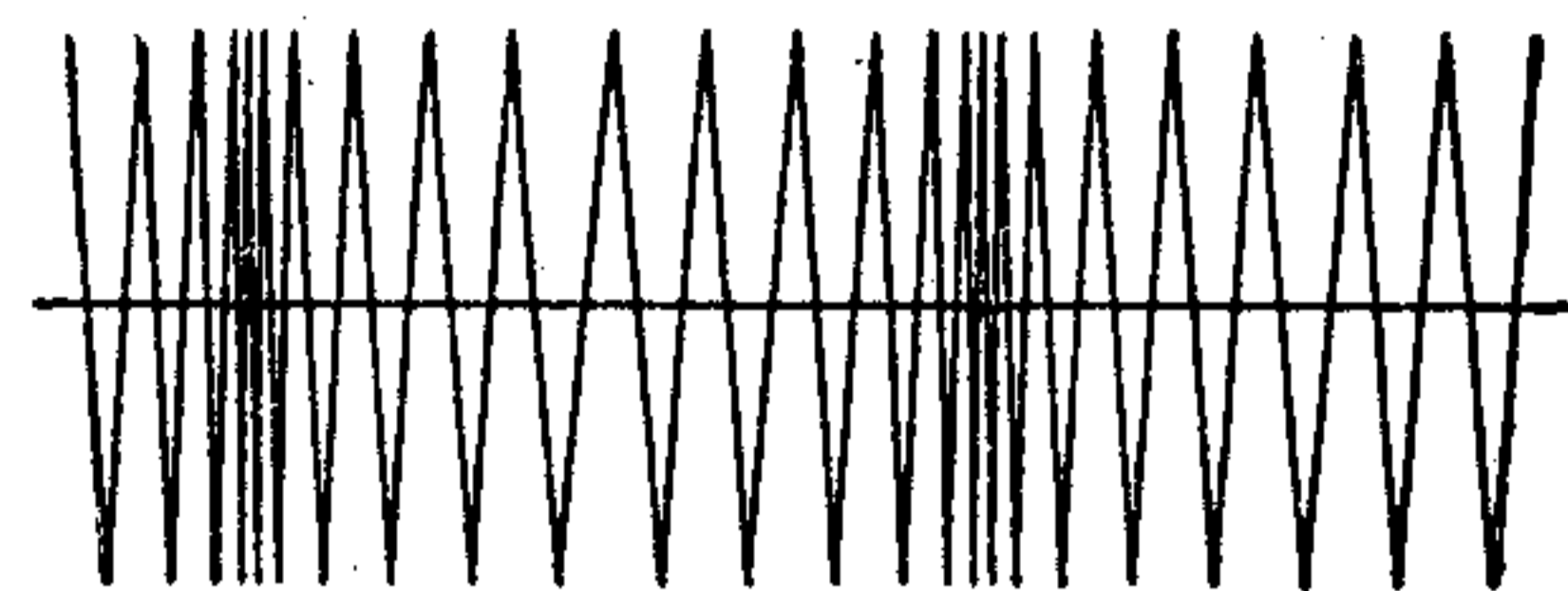
FREQUENCY-MODULATED RF WAVE
