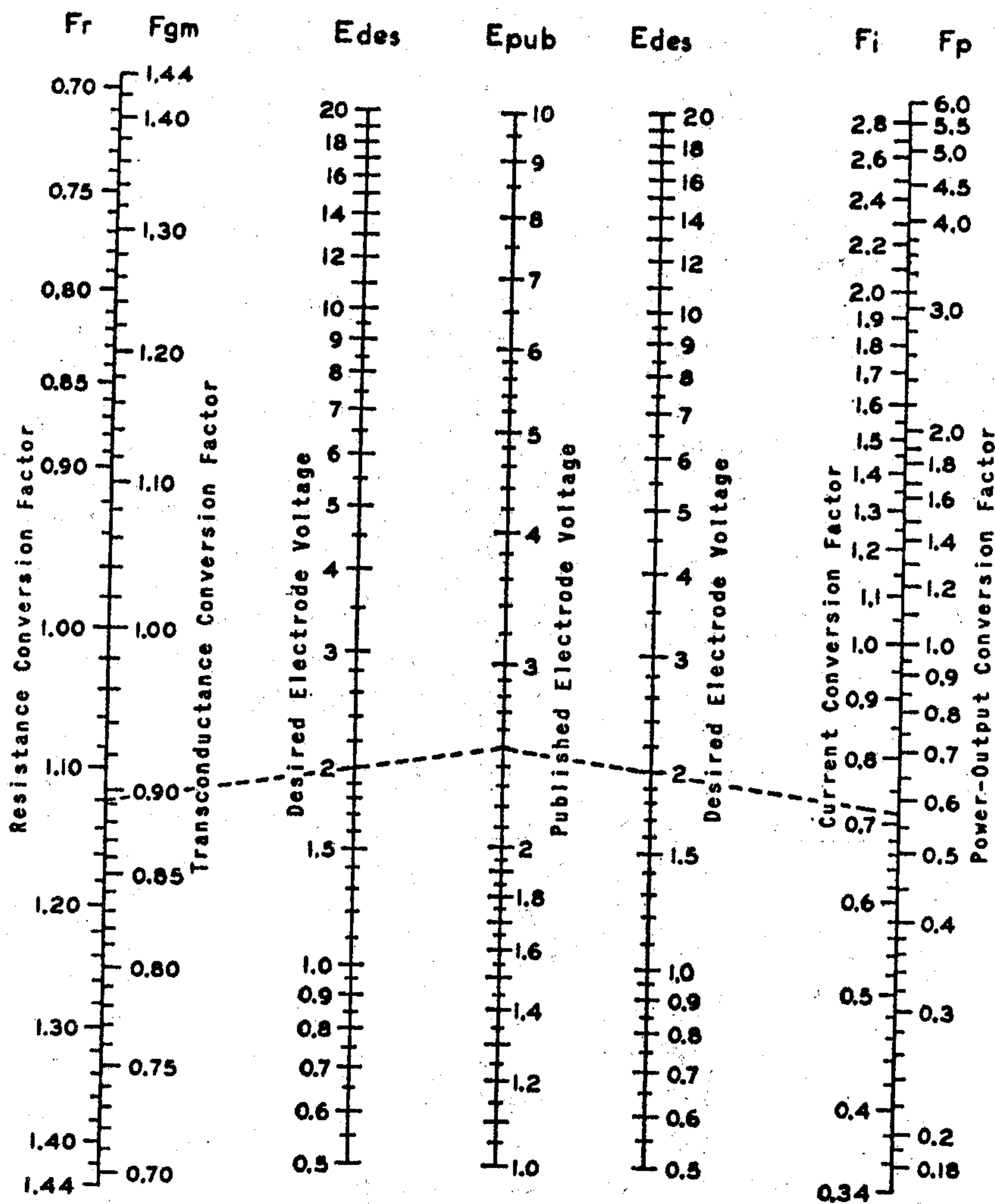
Fig. 44—Nomograph of tube conversion factors.
