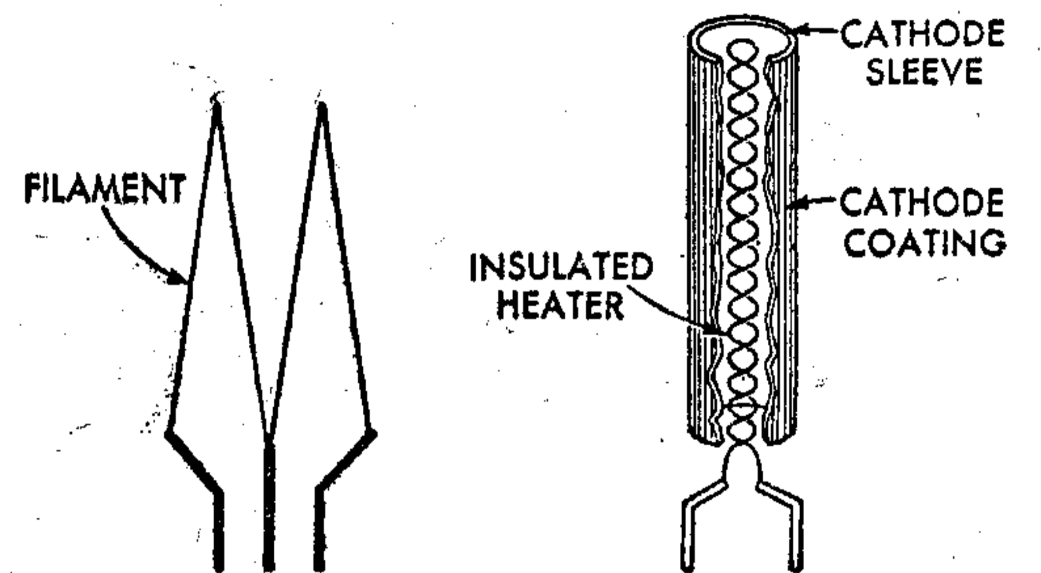
Fig. 1—Filament or directly heated cathode.
