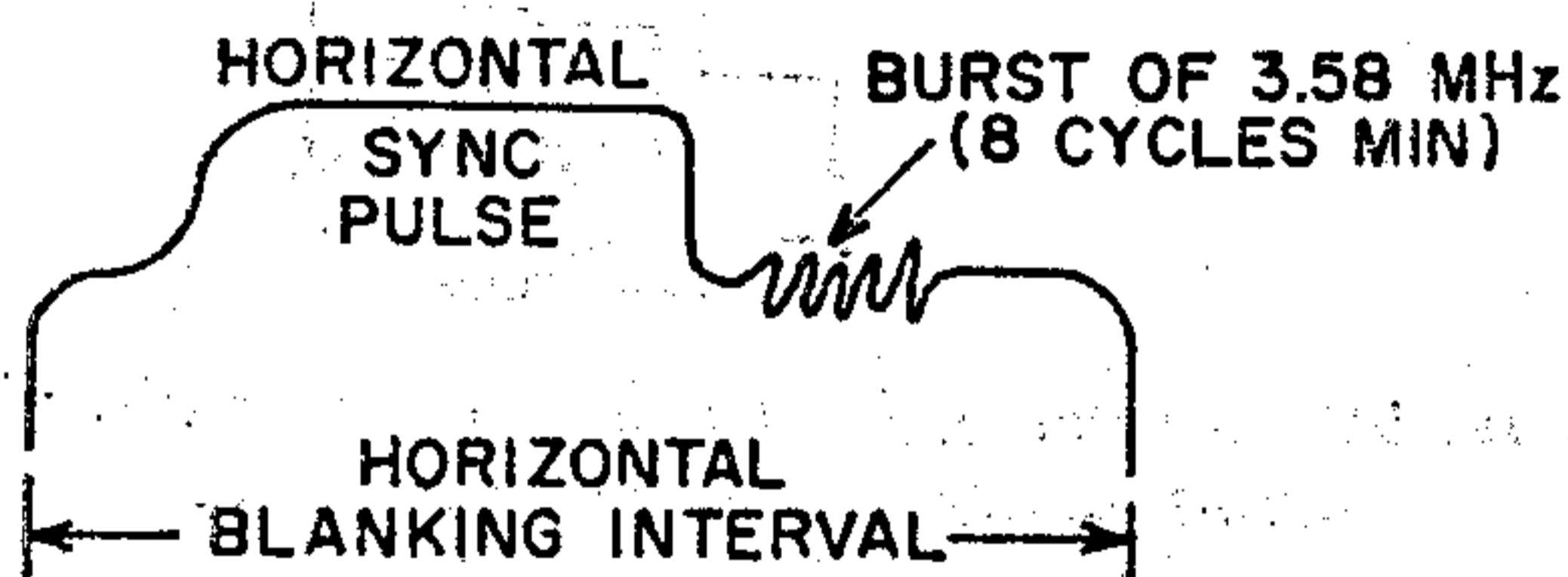
Fig. 95—Waveform for synchronizing signal.
