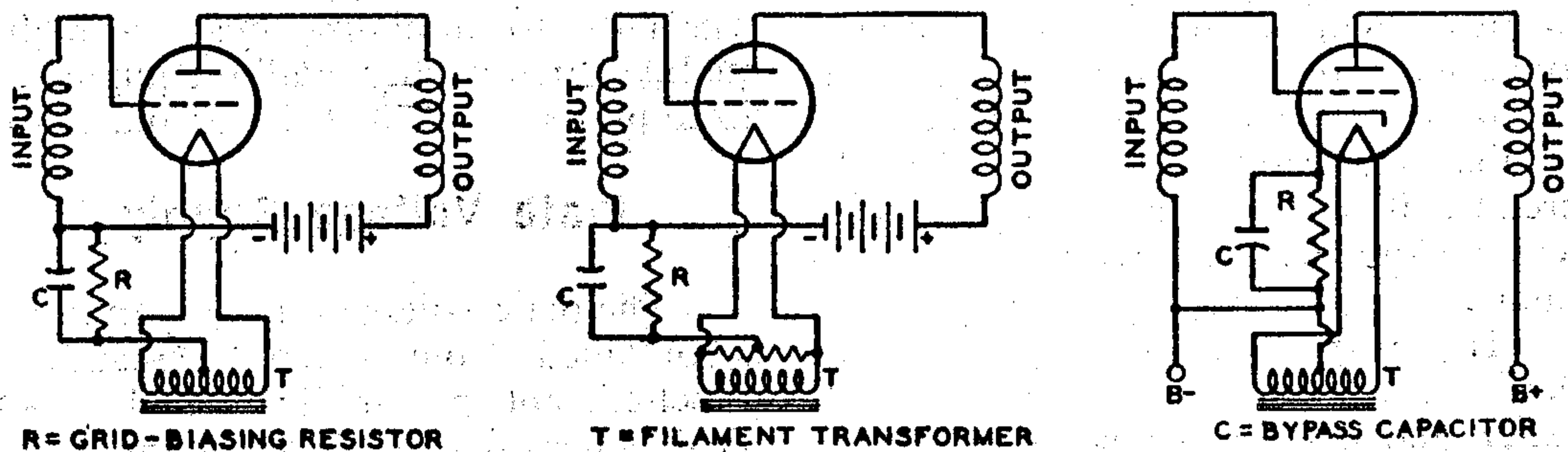
Fig. 113—Typical grid-voltage supply circuits.
