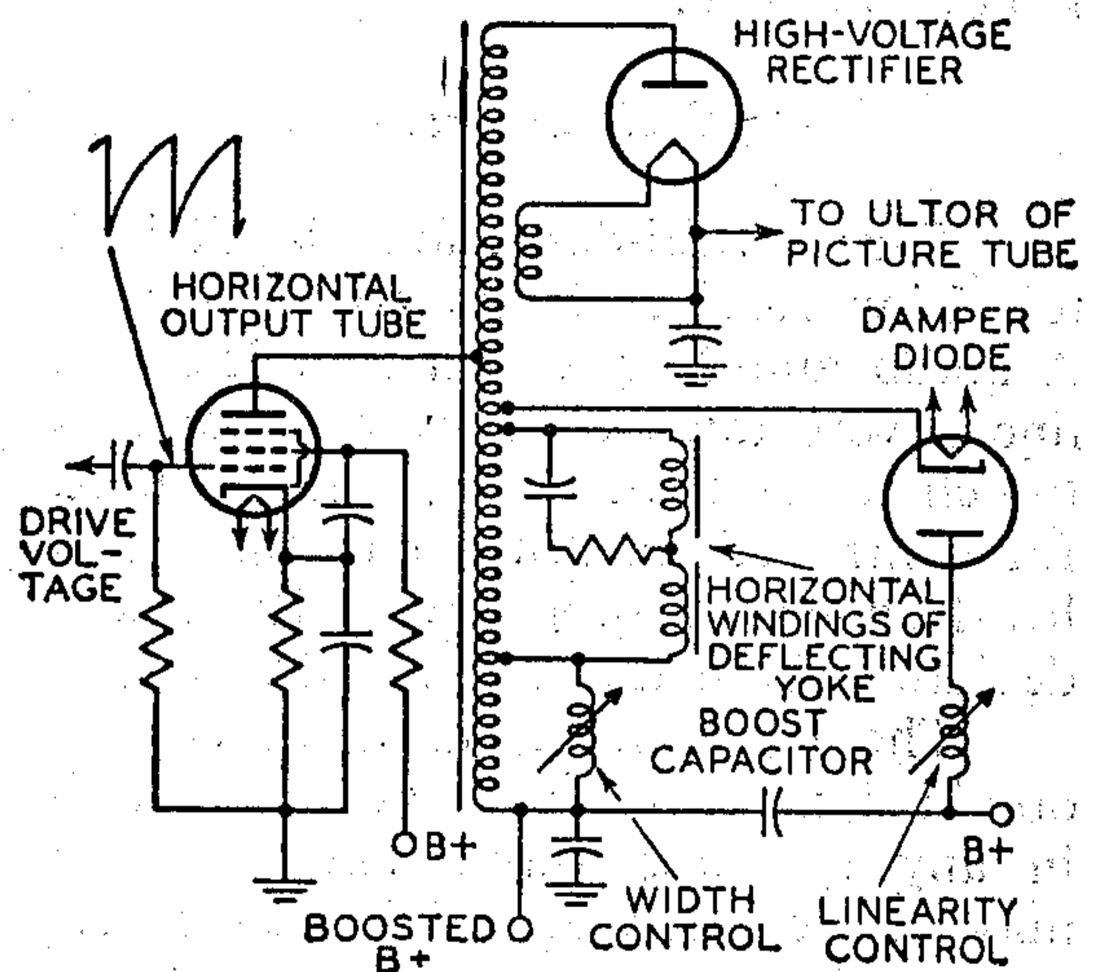
Fig. 89—Typical horizontal-deflection and high-voltage circuit.
