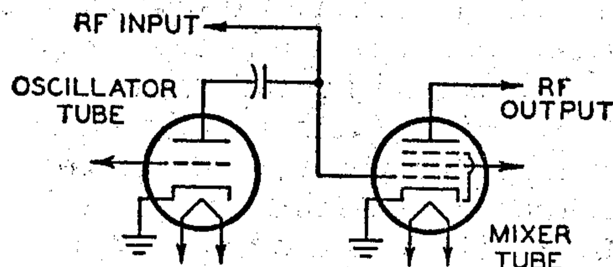
Fig. 108—Typical television mixer-oscillator circuit.
