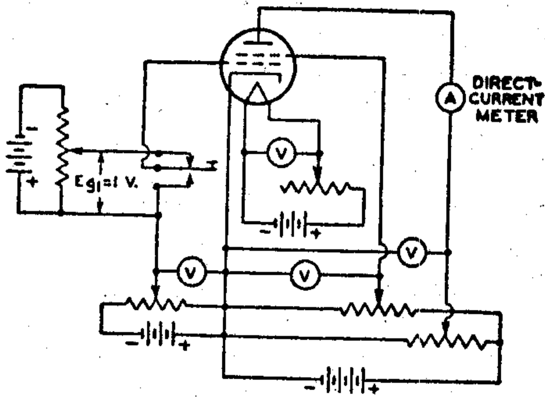
Fig. 131—Fundamental circuit of a transconductance tester using the "grid-shift" method.
