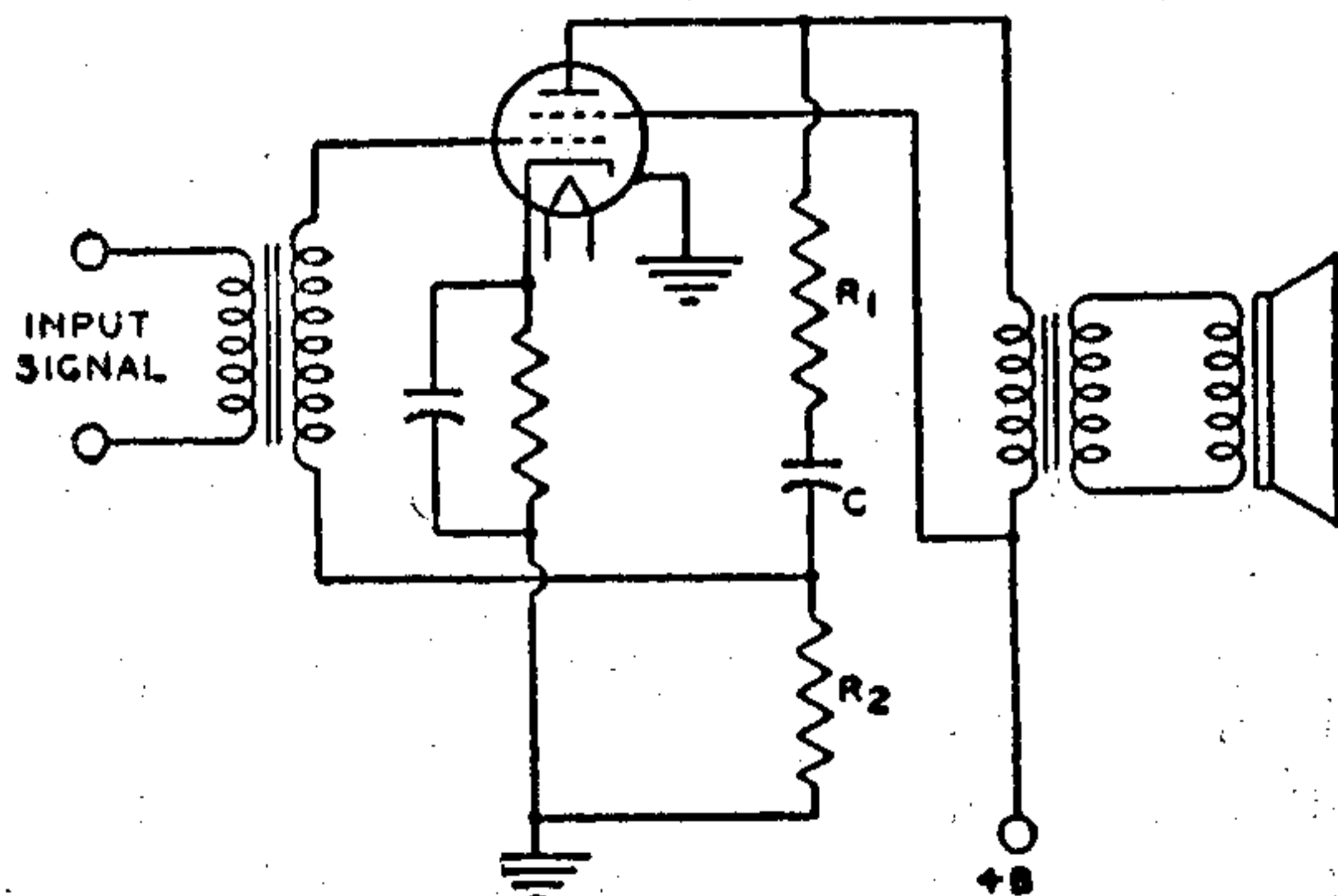
Fig. 48—Power-output stage using constant-voltage inverse feedback.
