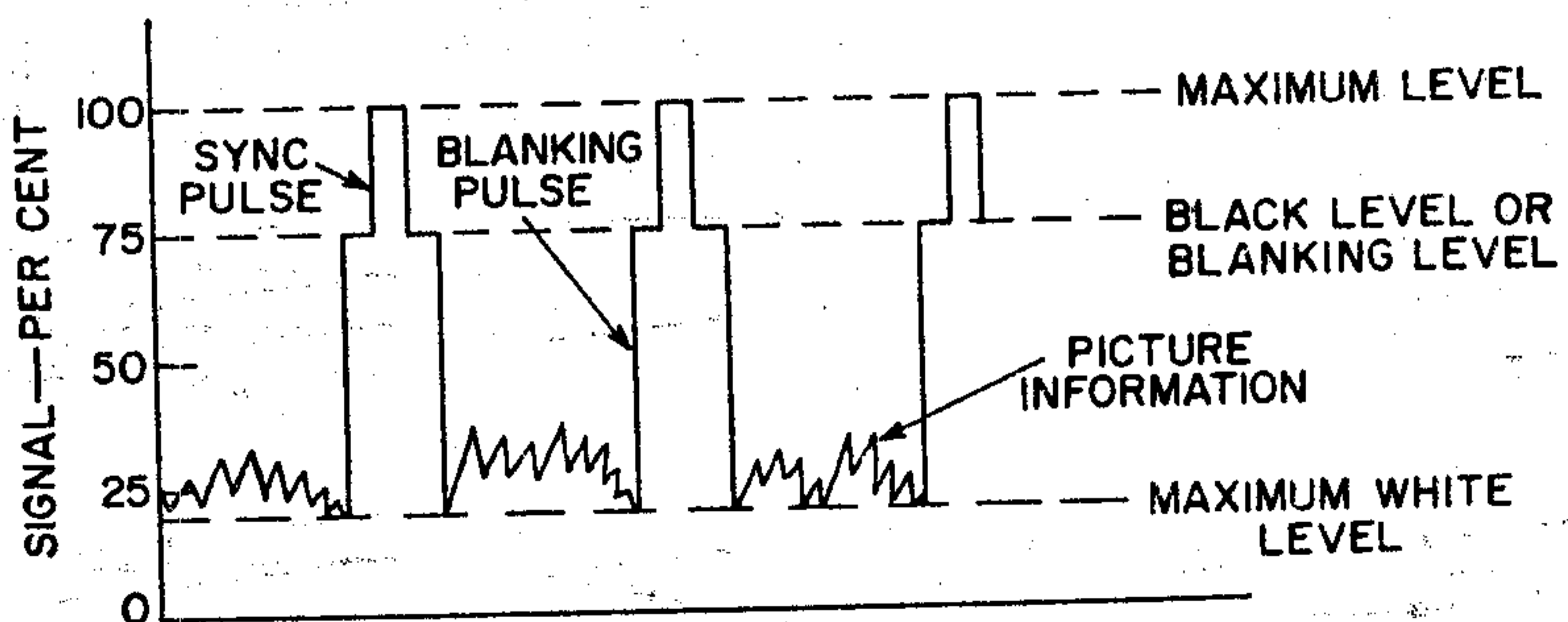
Fig. 79—Detected video signal.
