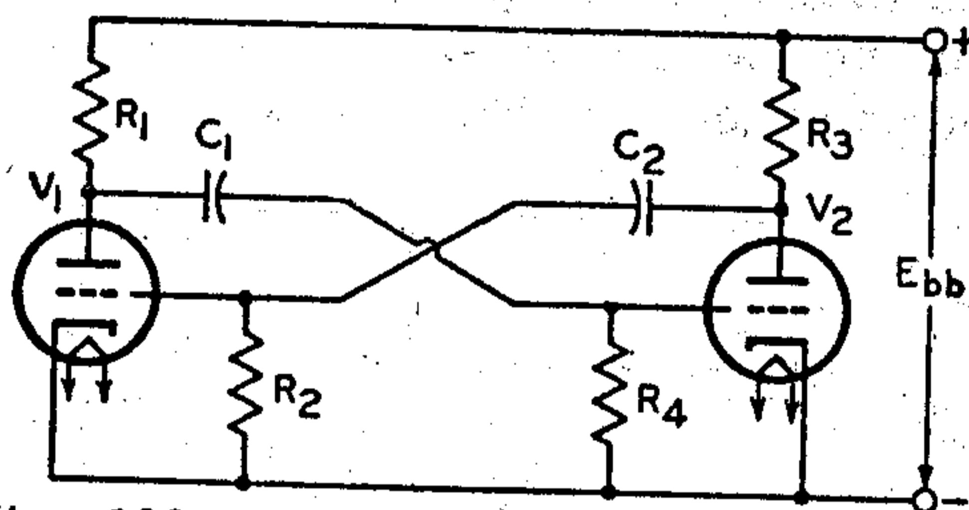
Fig. 100—Basic multivibrator circuit of the free-running type.
