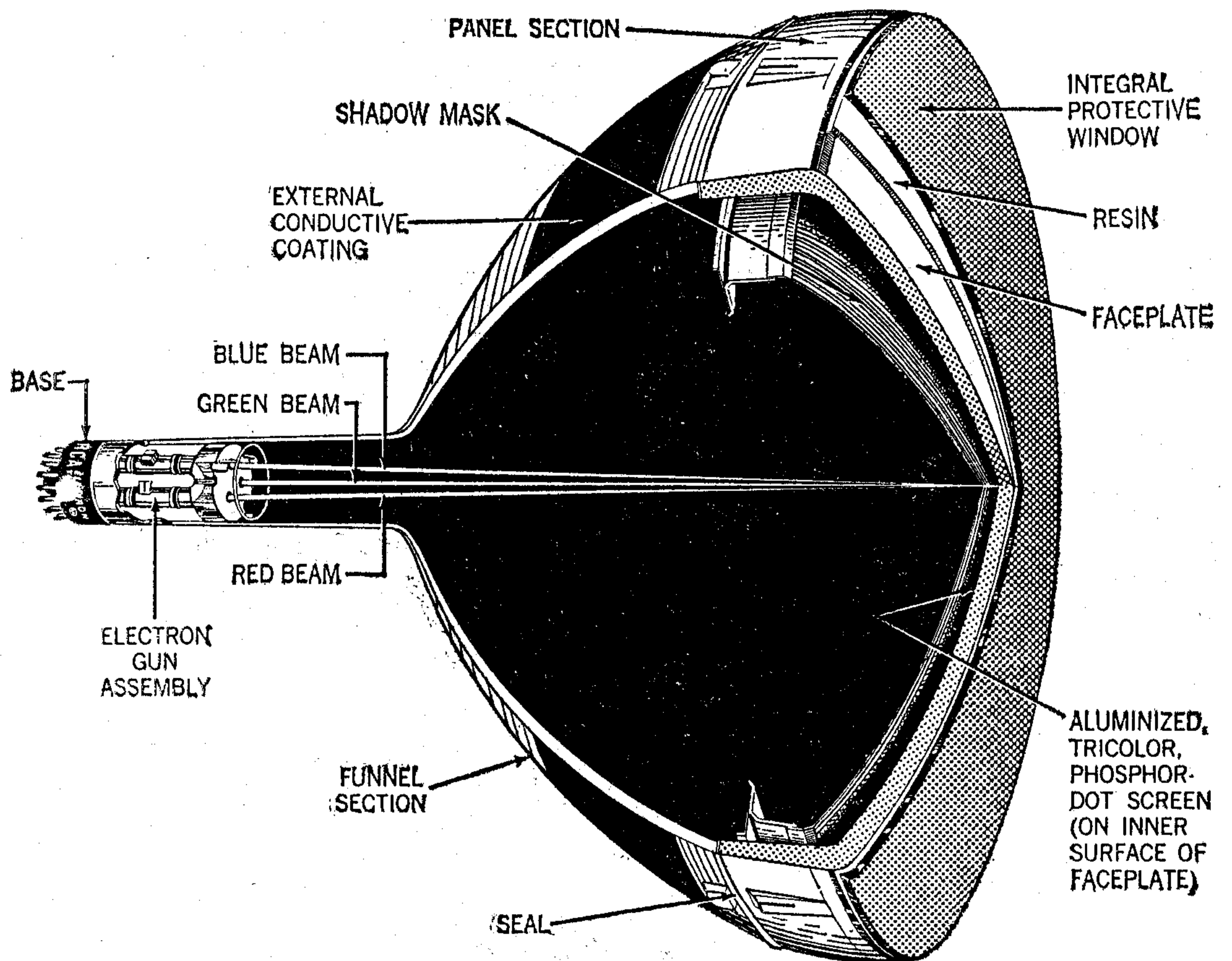
Fig. 11—Cutaway view of color television picture tube.
