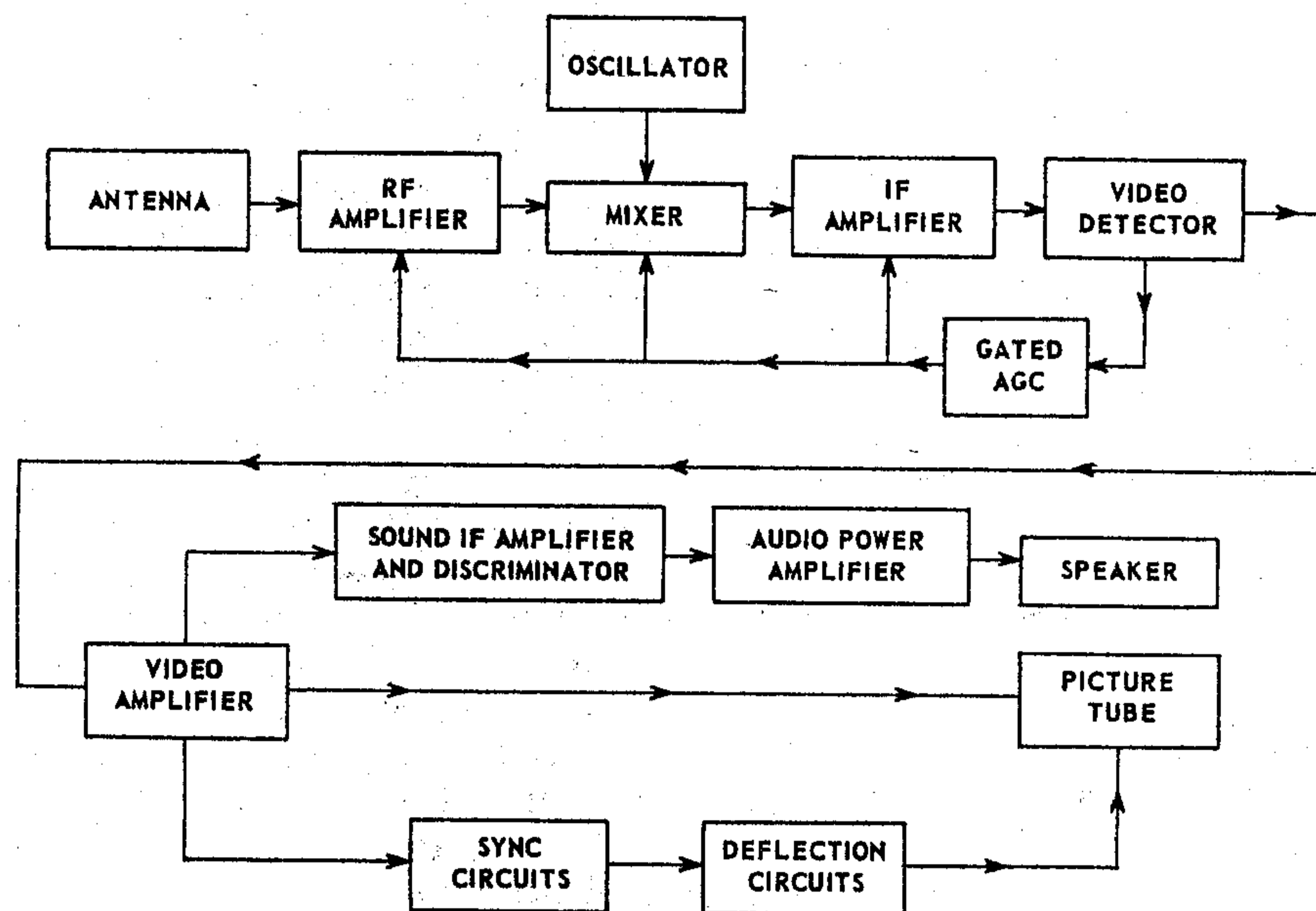
Fig. 15—Simplified block diagram for a television receiver.
