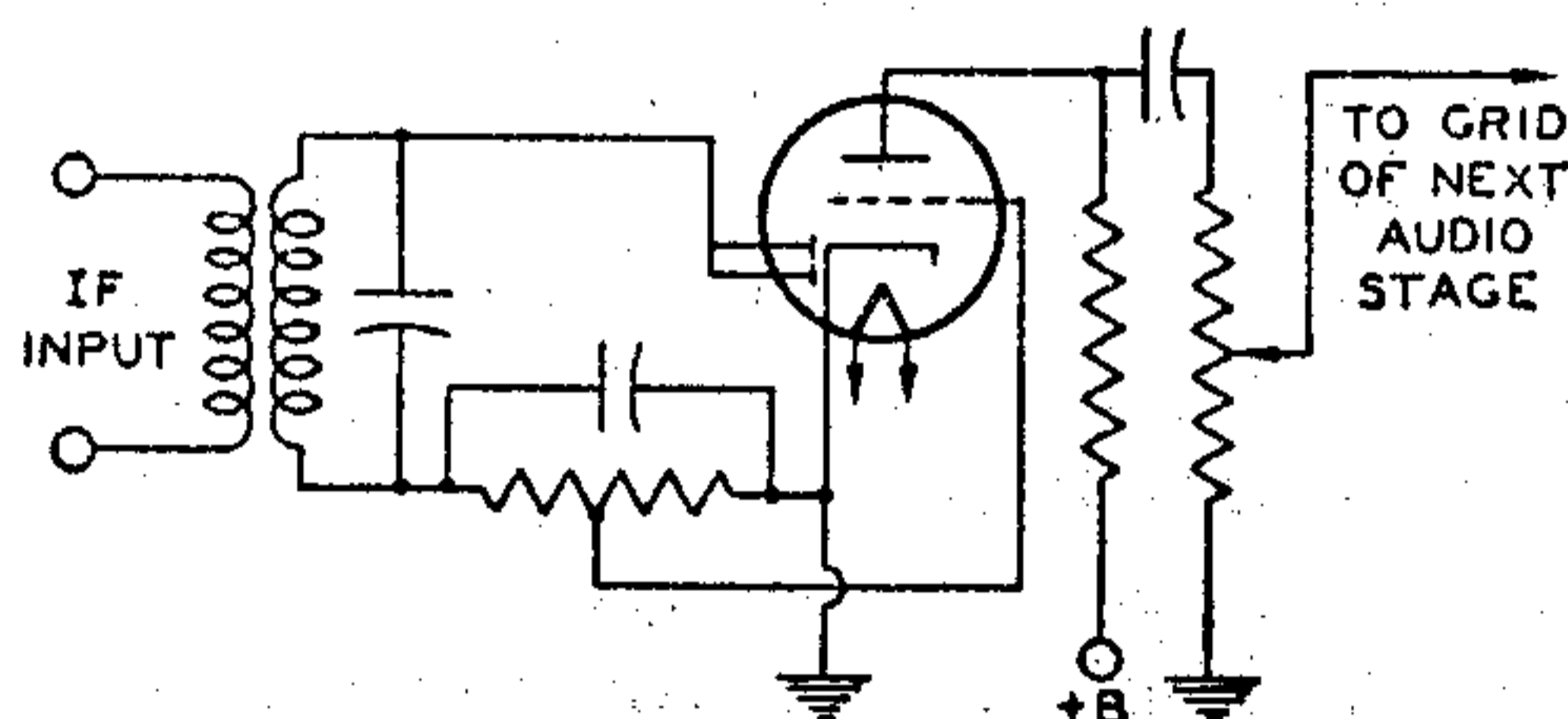
Fig. 25—Diode-biased detector circuit.
