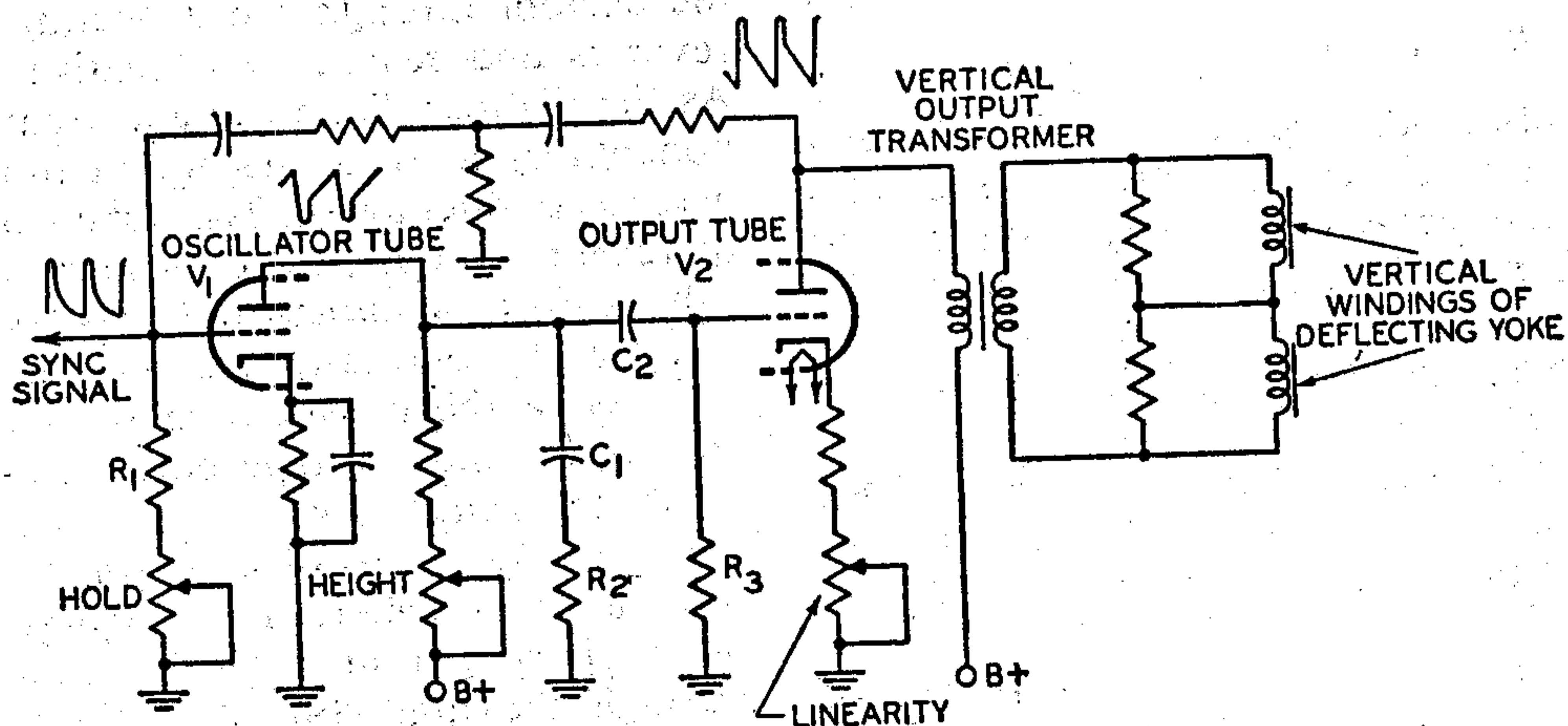
Fig. 90—Simplified combined vertical-oscillator-and-output stage.
