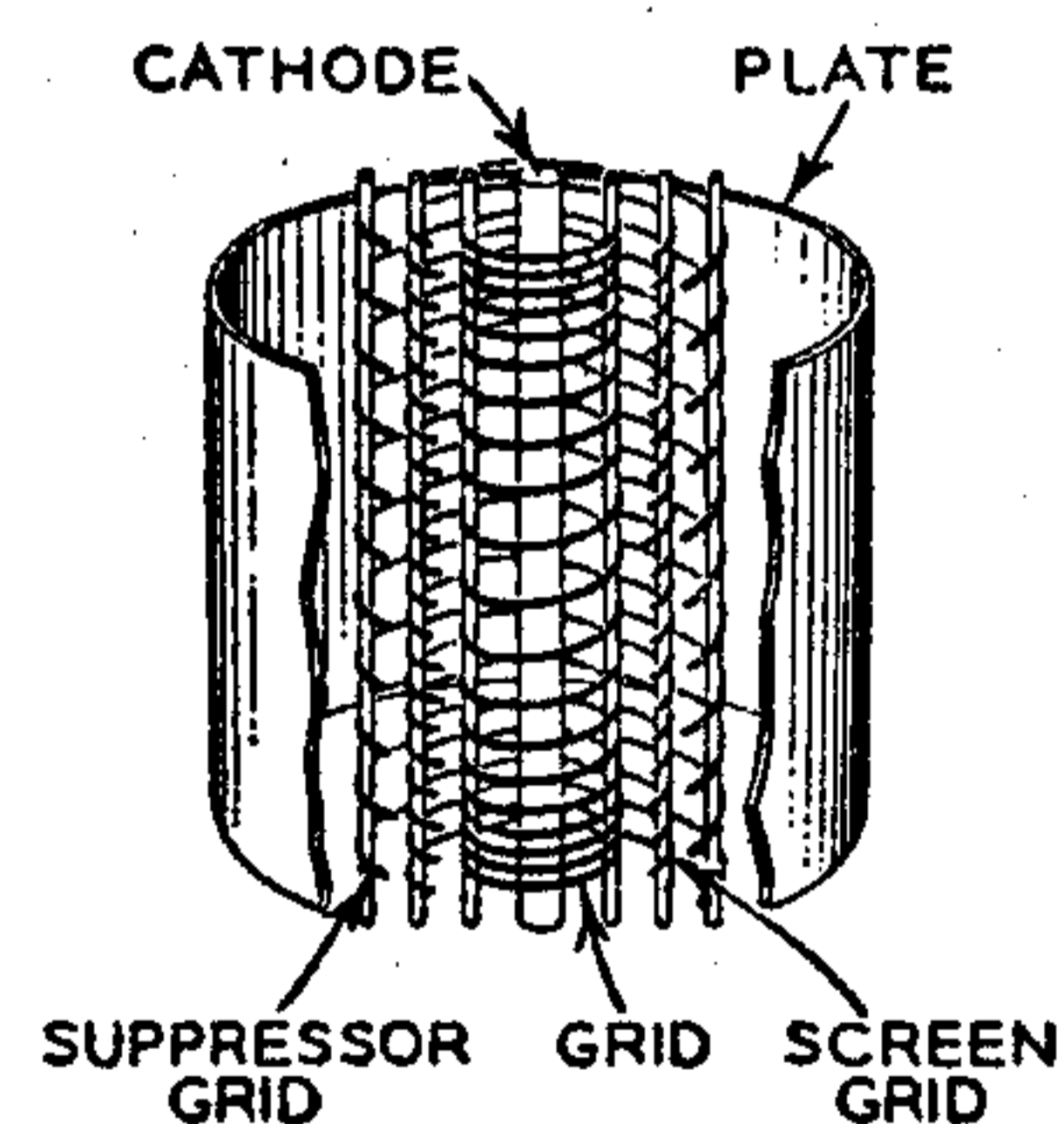
Fig. 37—Structure of remote-cutoff grid.
