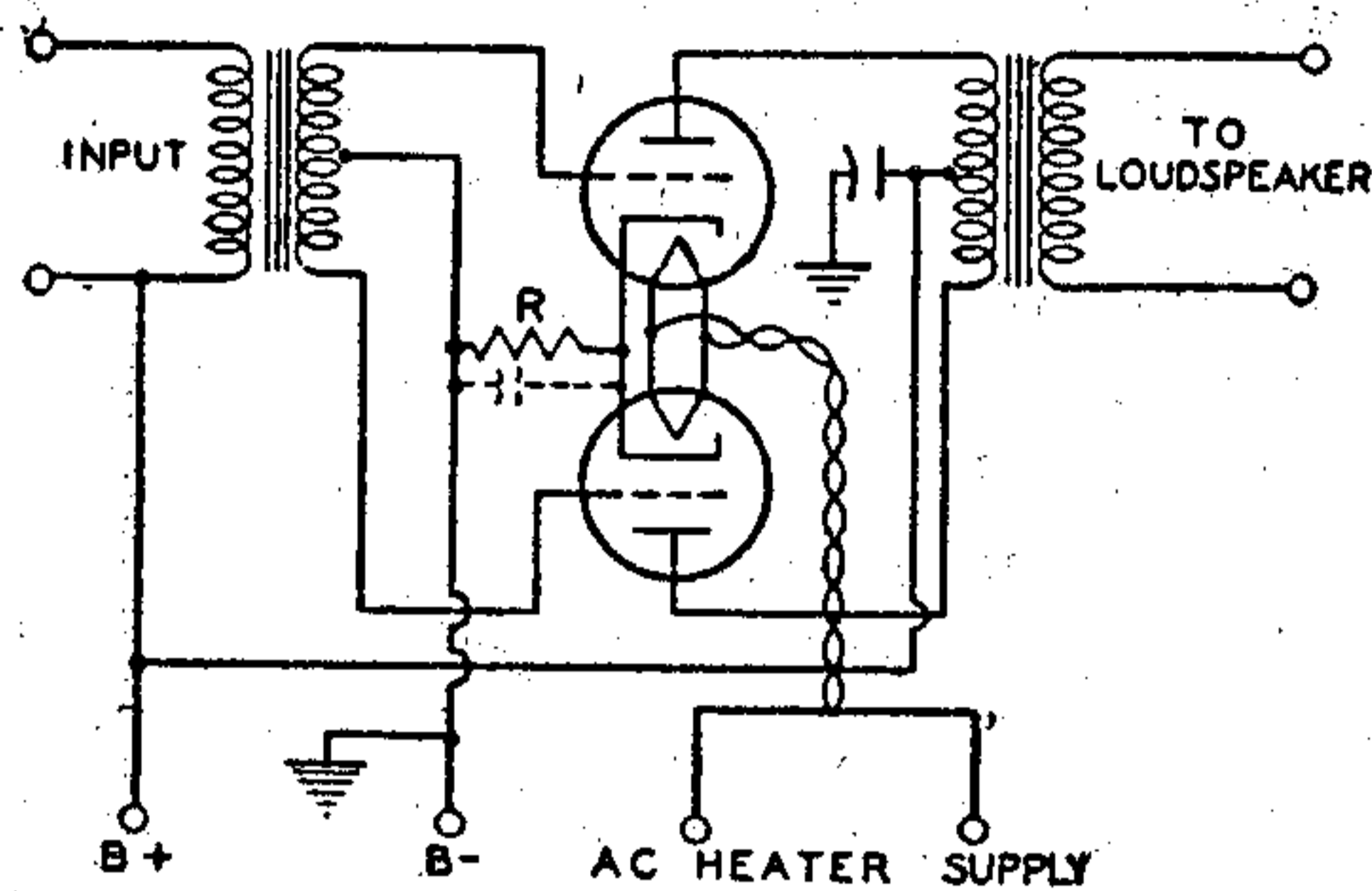
Fig. 40—Power amplifier with tubes connected in push-pull.
