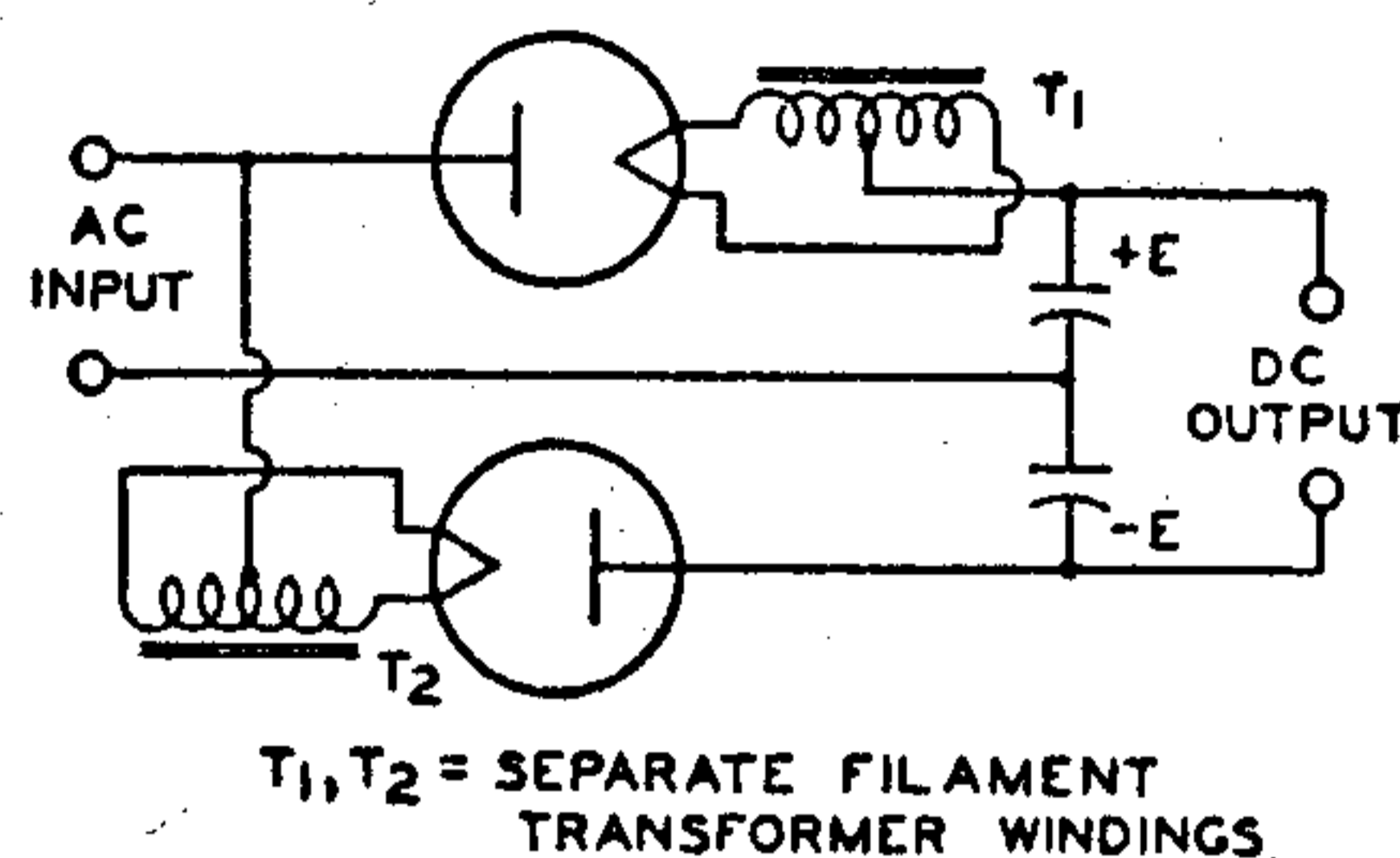
Fig. 19—Full-wave voltage-doubler circuit.
