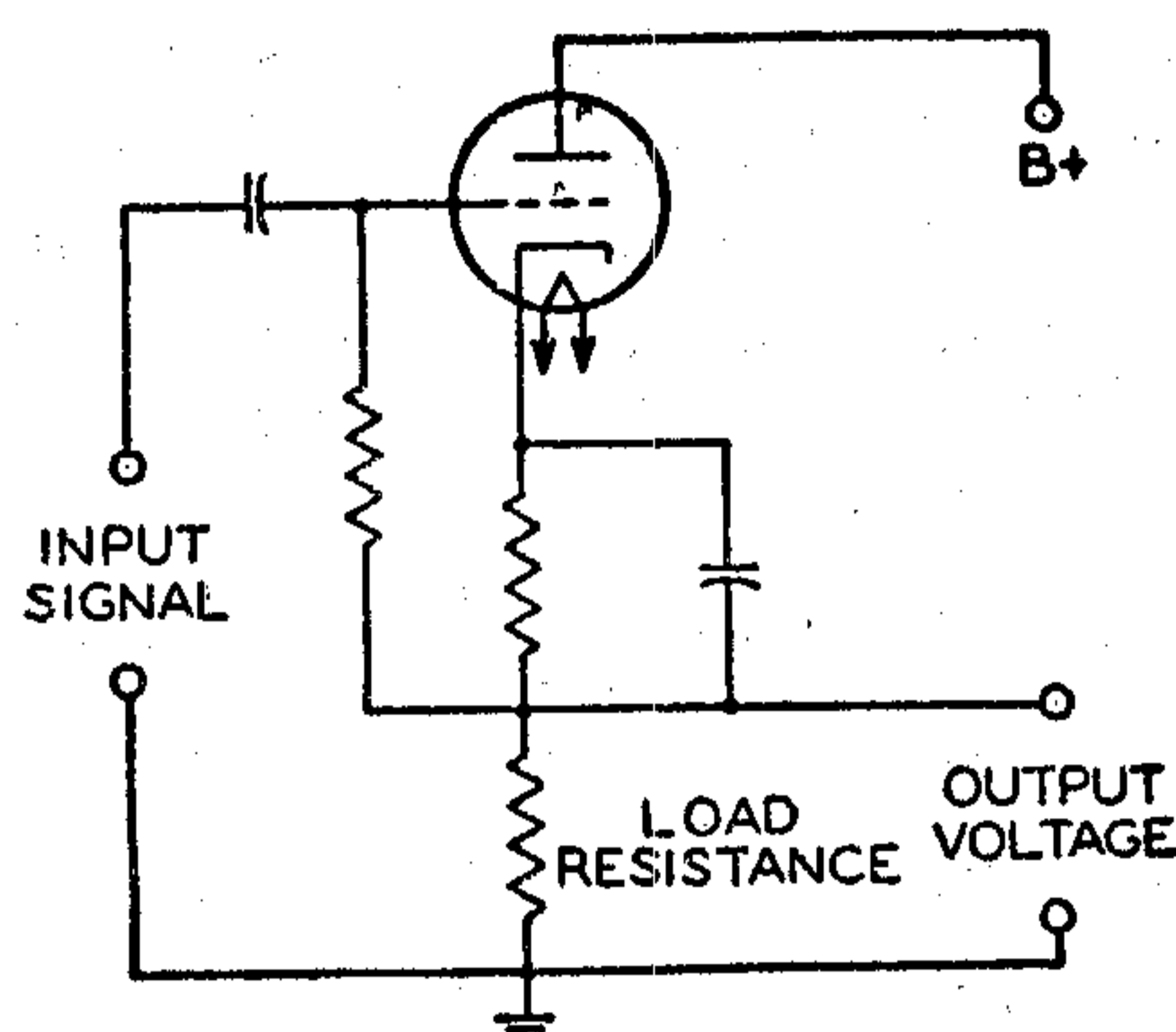
Fig. 53—Cathode-follower circuit modified for reduced bias.
