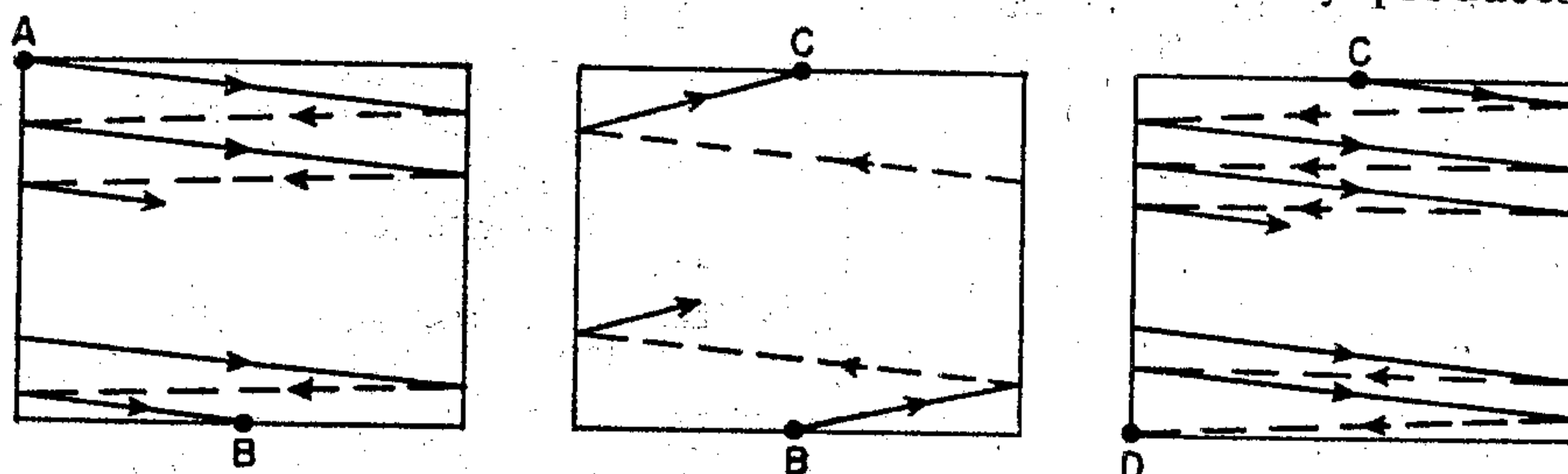
Fig. 78—The odd-line interlaced scanning procedure.
