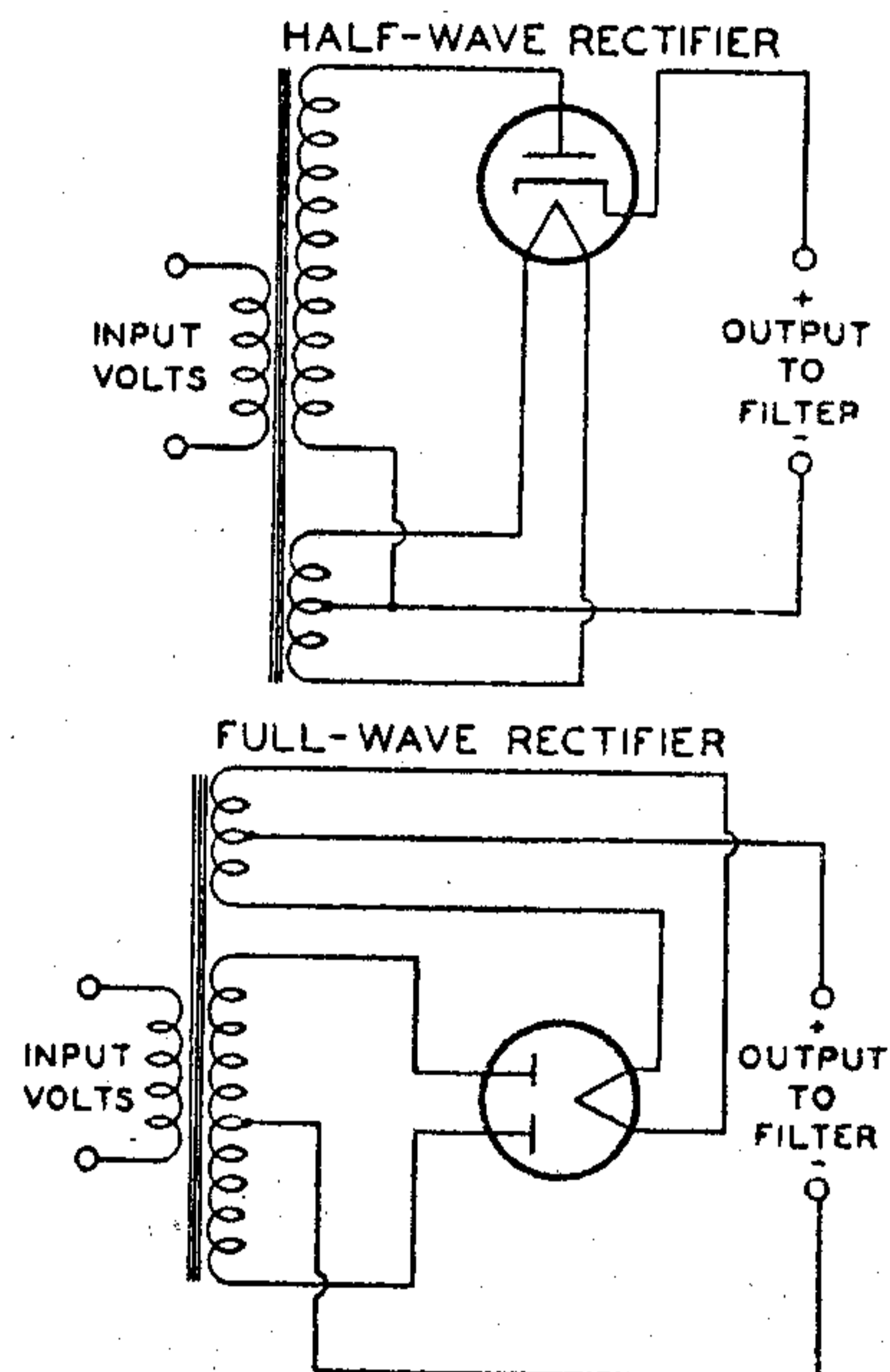
Fig. 18—Half-wave and full-wave rectifier circuits.
