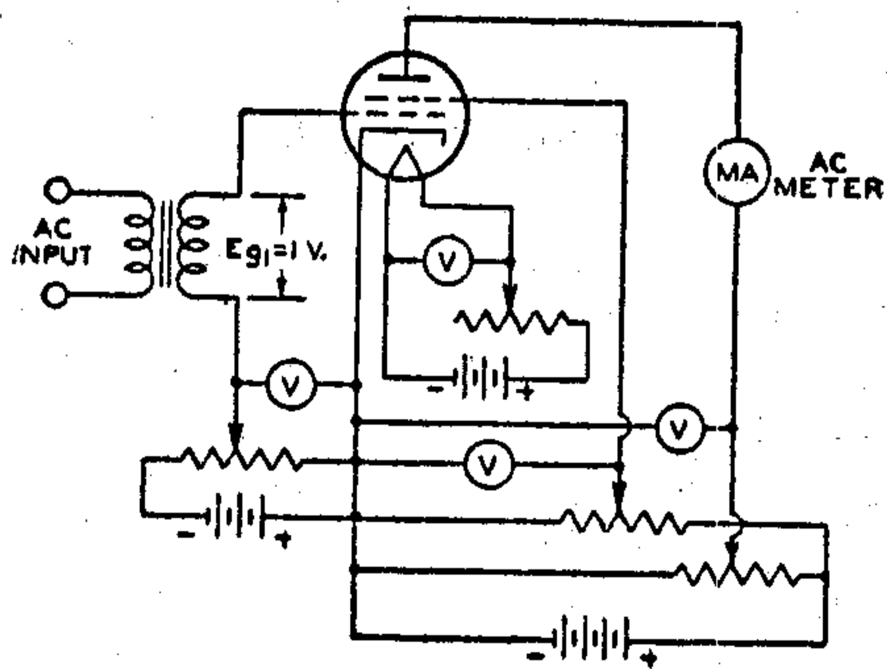
Fig. 132—Fundamental circuit of a dynamic transconductance tester.
