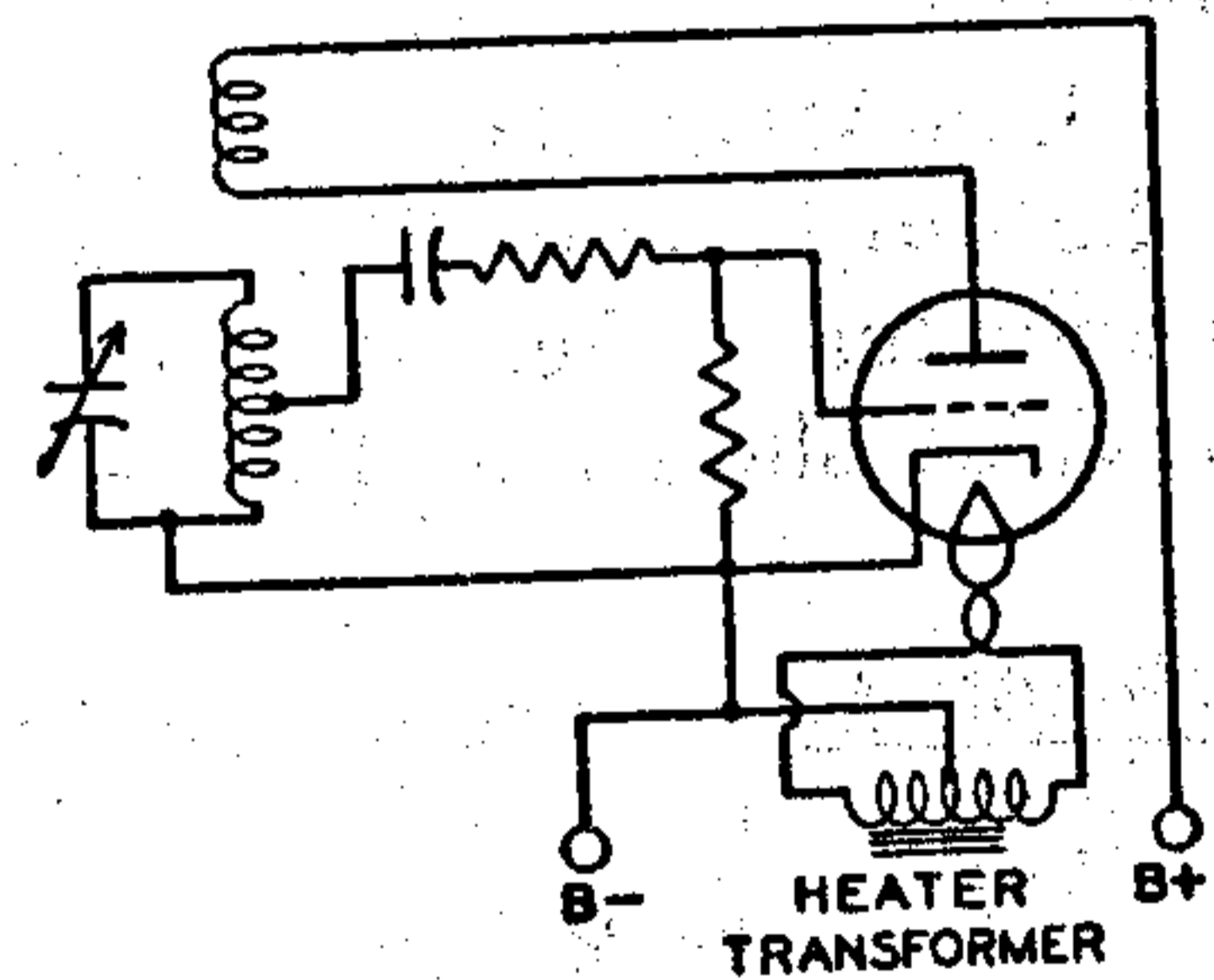
Fig. 99—Tuned-grid triode oscillator circuit using heater-cathode-type tube.
