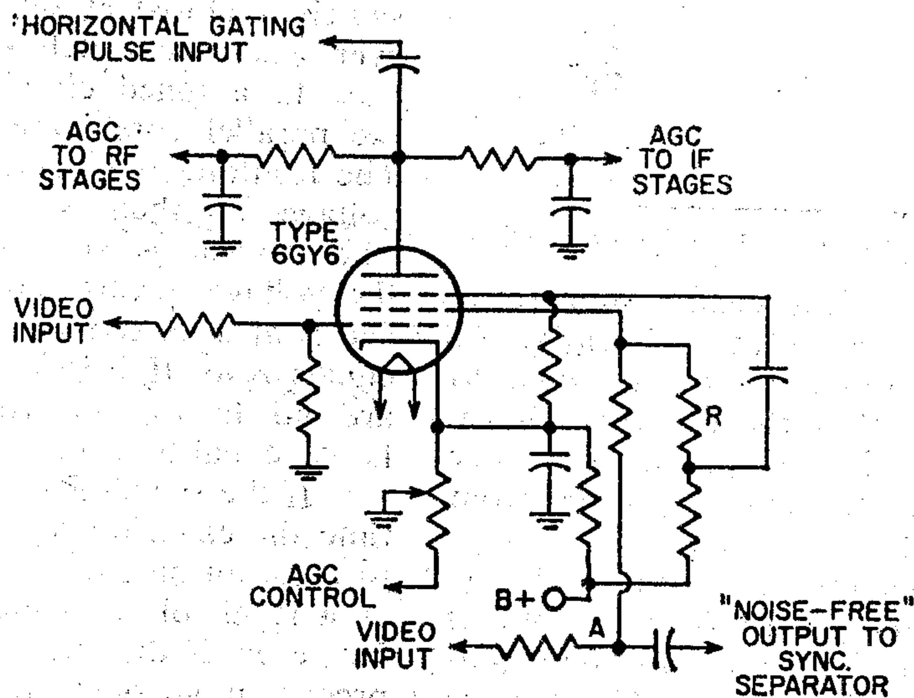
Fig. 84—Typical noise-cancellation circuit.
