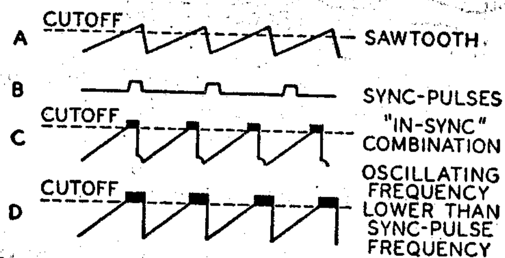
Fig. 102—Sawtooth and sync pulses in synchroguide circuit.
