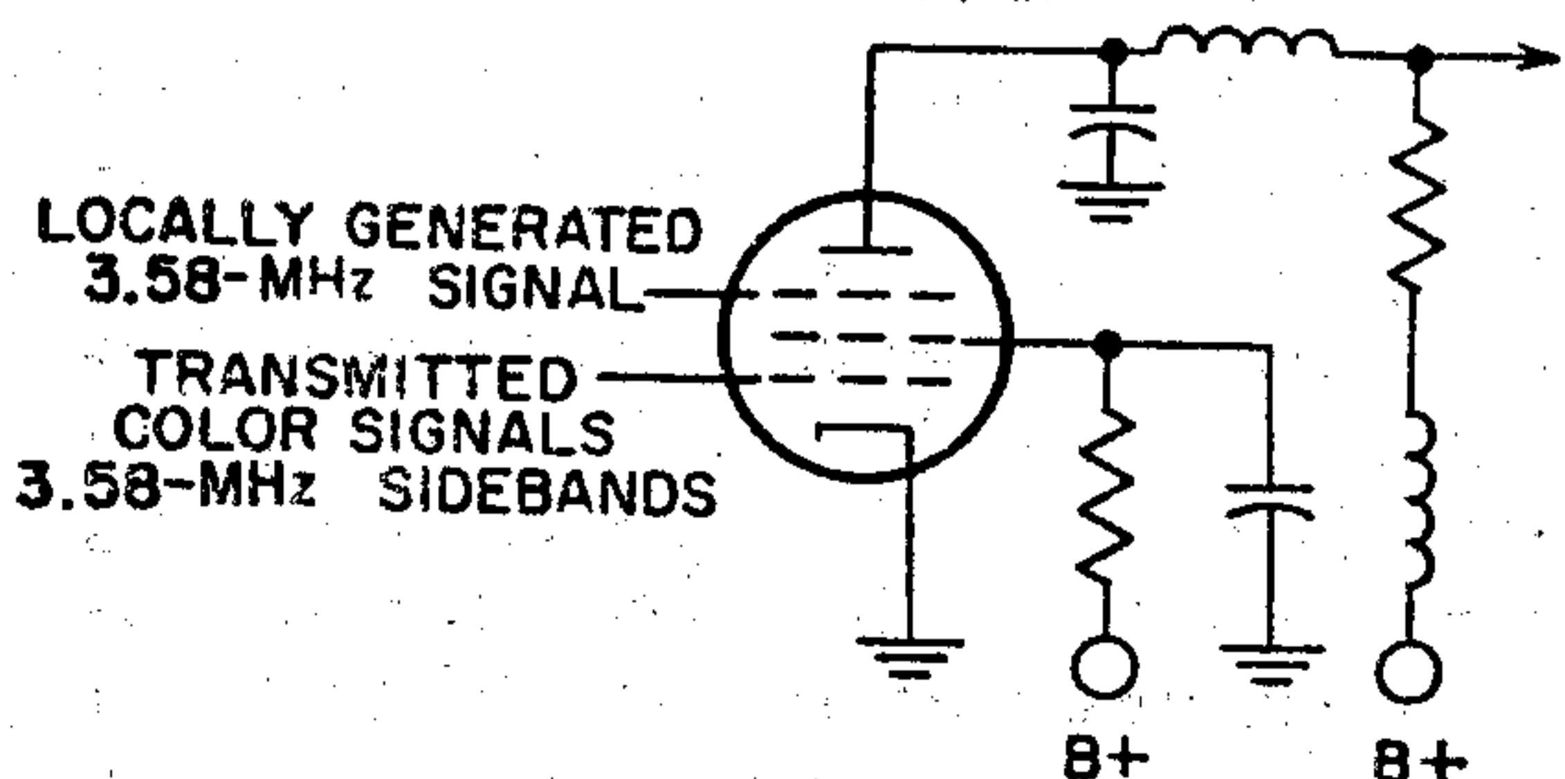
Fig. 96—Low-level color demodulator.
