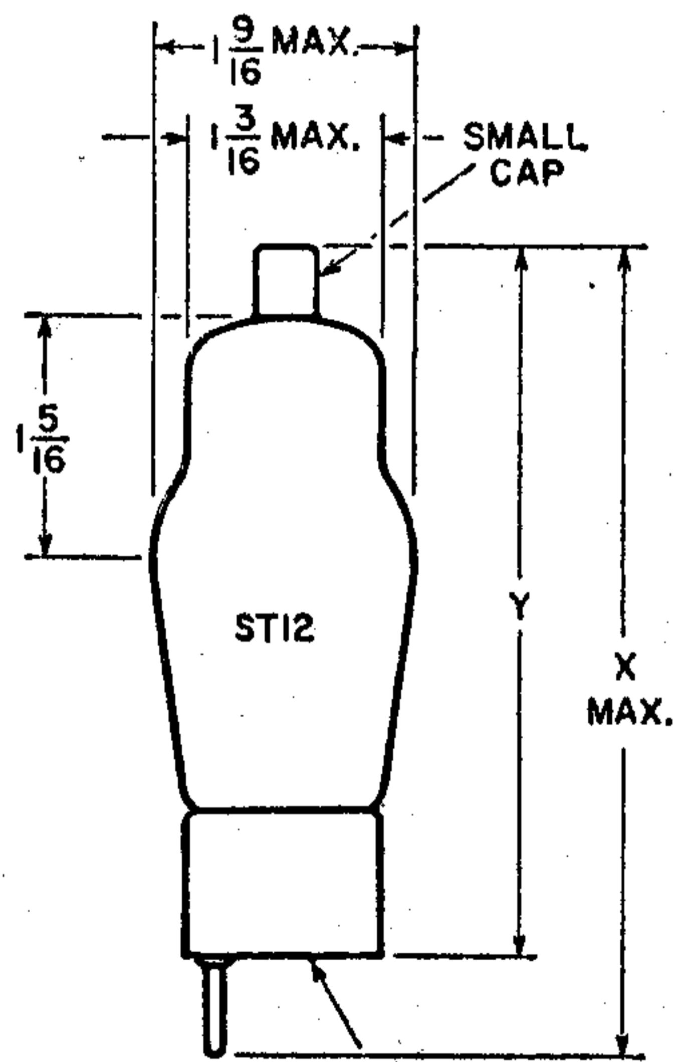
SMALL-SHELL SMALL 4-, 5-, 6-, OR 7-PIN
