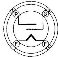
BOTTOM VIEW MEDIUM 4-PIN BAYONET BASE
