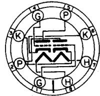
BOTTOM VIEW INTERMEDIATE SHELL 8-PIN OCTAL MICANOL
