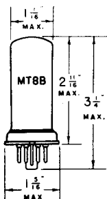
SMALL 7 PIN OCTAL BASE
