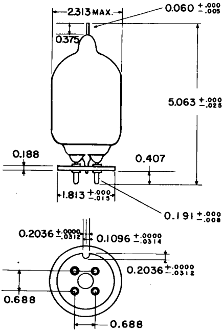
TUBE DIMENSIONS
