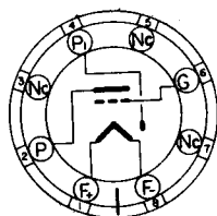
BOTTOM VIEW LOCKING-IN 8-PIN
