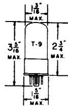
GLASS BULB 6 PIN OCTAL BASE WITH METAL SHELL 6C5GT
