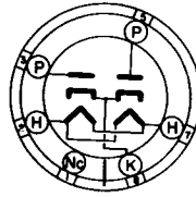
G-6S BOTTOM VIEW 6X5GT/G
