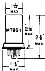
METAL SHELL 6SK7
