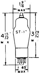
GLASS BULB SMALL 7 PIN OCTAL BASE 6R7G
