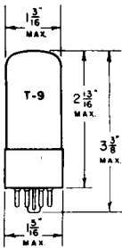
5Y3GT/G - MEDIUM 5 PIN OCTAL BASE
