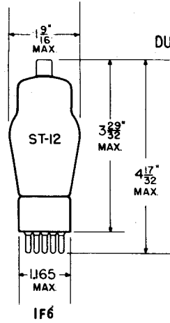
SMALL METAL CAP
