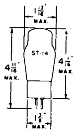
80 - MEDIUM 4 PIN BASE
