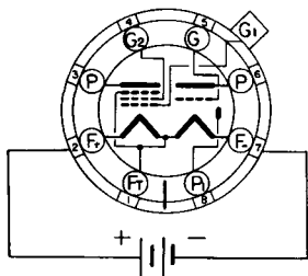
FILAMENTS CONNECTED IN SERIES
