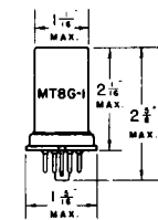
METAL TUBE SMALL WAFER 8 PIN OCTAL BASE 12SA7
