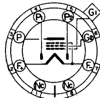
BOTTOM VIEW SMALL SHELL 8-PIN OCTAL
