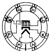
BOTTOM VIEW LOCK-IN 8 PIN BASE
