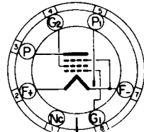
BOTTOM VIEW INTERMEDIATE SHELL OCTAL 7 PIN BASE
