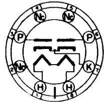
BOTTOM VIEW LOCK-IN 8 PIN BASE
