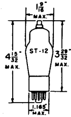
SMALL 8 PIN OCTAL BASE 1C7G
