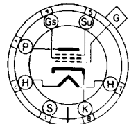
7R BOTTOM VIEW 6K7 6K7GT
