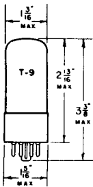
5Y3GT/G - MEDIUM 5 PIN OCTAL BASE
