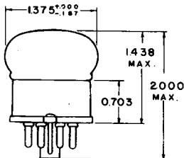
TUBE DIMENSIONS
