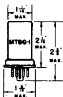
METAL TUBE SMALL WAFER 8 PIN OCTAL BASE 6SA7
