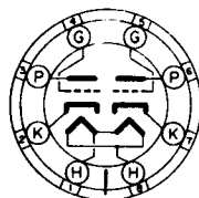
8AC BOTTOM VIEW
