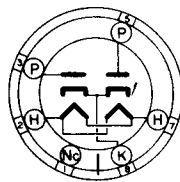
G-6S BOTTOM VIEW
