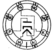
BOTTOM VIEW 8 PIN LOCK-IN
