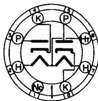
BOTTOM VIEW INTERMEDIATE SHELL 8 PIN OCTAL
