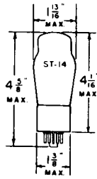
5Y4G - MEDIUM 8 PIN OCTAL BASE
