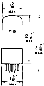
GLASS BULB 6F6GT/G
