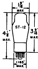
SMALL 7 PIN OCTAL BASE 6K6G
