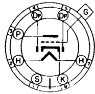
7 V BOTTOM VIEW
