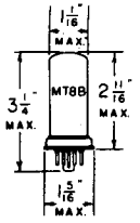
METAL SHELL 5 PIN OCTAL BASE 5W4
