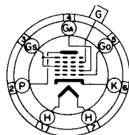
7C BOTTOM VIEW
