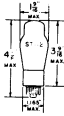
GLASS BULB SMALL 6 PIN OCTAL BASE 6C5G
