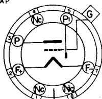
BOTTOM VIEW 7-PIN OCTAL BASE WITH METAL SHELL
