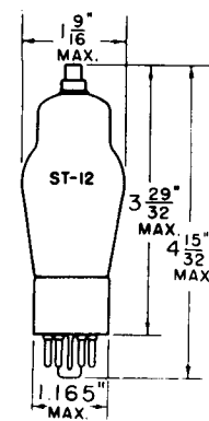
6V7G SMALL 7 PIN OCTAL BASE
