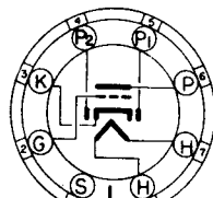
BOTTOM VIEW SMALL WAFER 8-PIN OCTAL METAL SLEEVE
