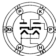
6J BOTTOM VIEW
