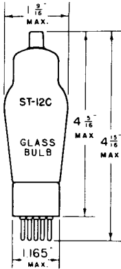
SMALL 6 PIN BASE
