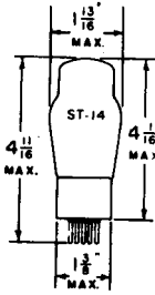
MEDIUM 5 PIN BASE 1F4
