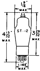
GLASS BULB SMALL 7 PIN OCTAL BASE 6K7G
