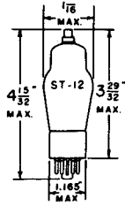
GLASS BULB SMALL 7 PIN OCTAL BASE 6K7G
