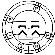
6S BOTTOM VIEW 6X5
