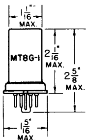
METAL SHELL SMALL WAFER OCTAL 8 PIN BASE
