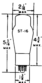
5U4G - MEDIUM 9 PIN OCTAL BASE
