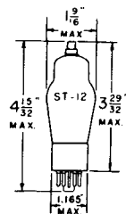
GLASS BULB SMALL 7 PIN OCTAL BASE 6L7G
