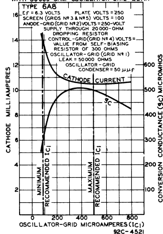
OPERATION CHARACTERISTICS WITH 50000-OHM OSCILLATOR-GRID LEAK
