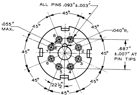
BOTTOM VIEW OF BASE
