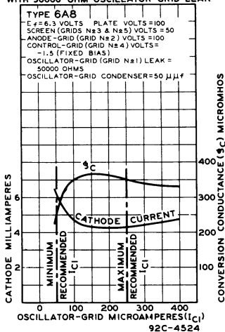
OPERATION CHARACTERISTICS WITH 50000-OHM OSCILLATOR-GRID LEAK
