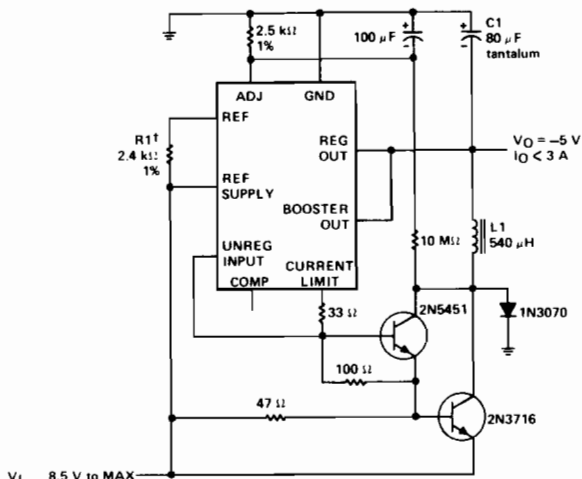
FIGURE 3—SWITCHING REGULATOR
