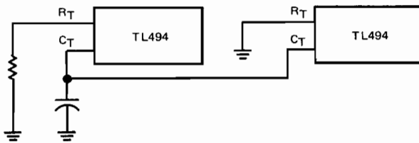
FIGURE 1—MASTER-SLAVE OSCILLATOR CONNECTION
