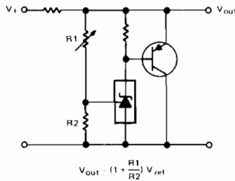
FIGURE 12—HIGHER-CURRENT APPLICATIONS
