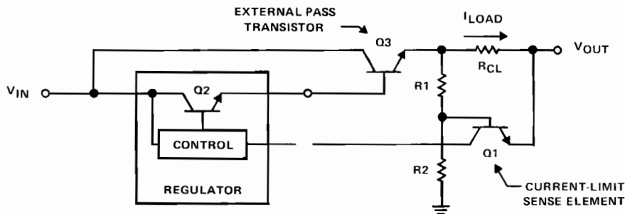
Figure 4.9. Fold-Back Current Limit Configuration
