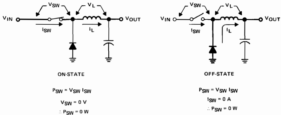
Figure 3.10. Switching Voltage Regulator Modes
