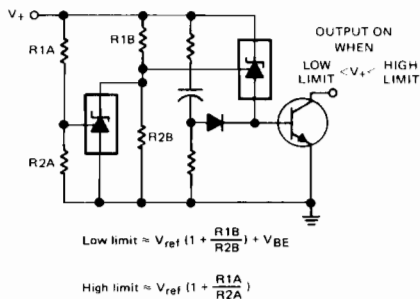
FIGURE 14—OVER-VOLTAGE/UNDER-VOLTAGE PROTECTION CIRCUIT
