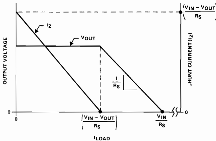
Figure 3.9. Output Voltage vs Load Current vs Shunt Current of a Shunt Regulator
