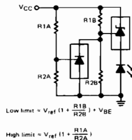
FIGURE 15— V_{CC} MONITOR
