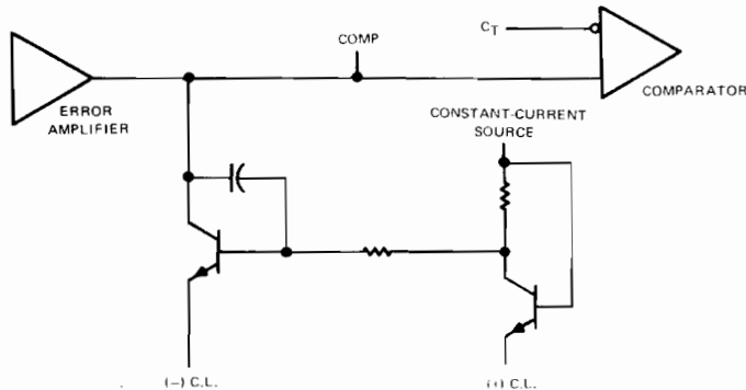
FIGURE 8—CURRENT-LIMIT SCHEMATIC
