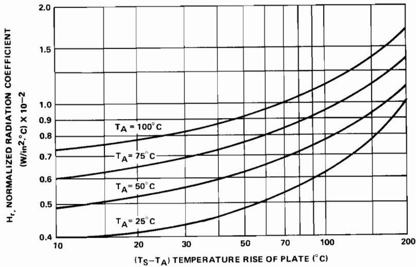
Figure 5.7. Normalized Heat Transfer Coefficient H_r
