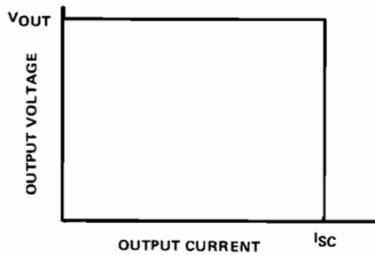
Figure 4.7. Constant-Current Limiting
