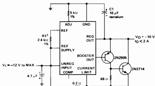
FIGURE 2—HIGH-CURRENT REGULATOR
