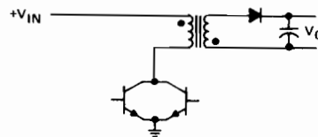
FLYBACK
