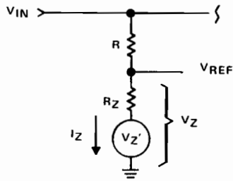
Figure 2.2. Zener Reference Model
