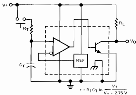
FIGURE 3—BASIC TIMER
