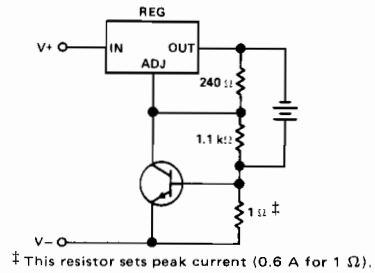
FIGURE 12—CURRENT-LIMITED 6-V CHARGER
