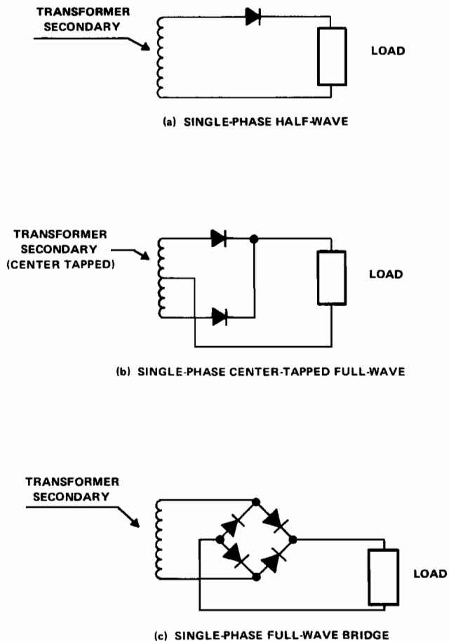
Figure 7.2. Input Supply Transformer/Rectifier Configurations
