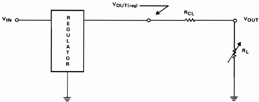
Figure 4.3. Series Resistance Current Limiter
