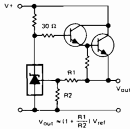
FIGURE 9—SERIES REGULATOR
