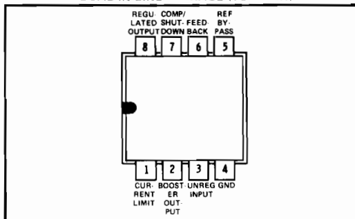
LM105 . . . JG LM205, LM305, LM305A, LM376 . . . JG OR P DUAL-IN-LINE PACKAGE (TOP VIEW)
