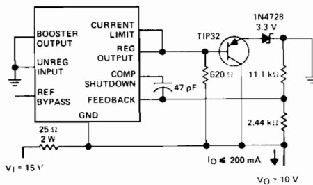
FIGURE 6—SHUNT REGULATOR
