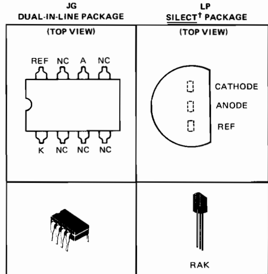
NC—No internal connection
