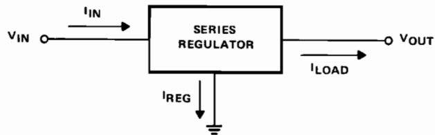
Figure 3.5. Series Regulator
