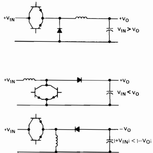
FIGURE 10—SINGLE-ENDED INDUCTOR CIRCUIT
