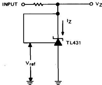
FIGURE 1—TEST CIRCUIT FOR V_Z = V_{ref}
