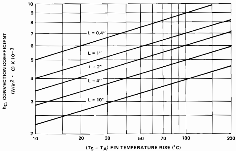
Figure 5.6. Convection Coefficient h_C
