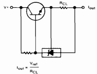
FIGURE 10—CURRENT LIMITER
