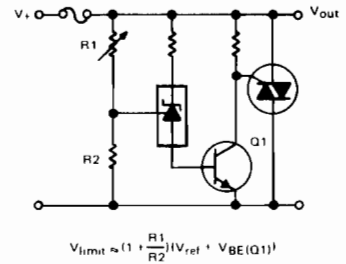
FIGURE 13—CROW BAR
