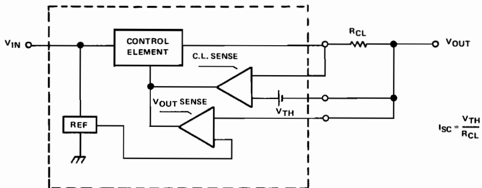
Figure 4.5. Constant Current Limit Configuration
