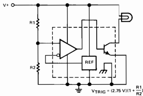
FIGURE 4—OVER-VOLTAGE DETECTOR
