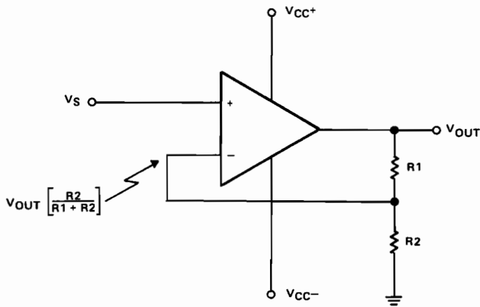
Figure 2.7. Comparator Model Showing Common-Mode Voltage
