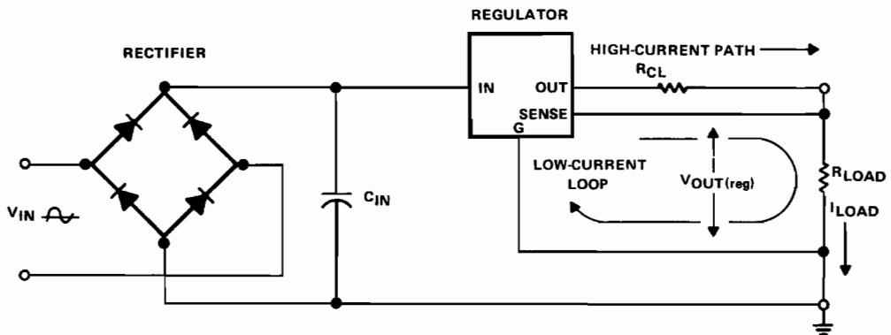
Figure 6.2. Proper Regulator Layout
