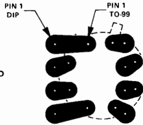
TYPICAL P.C. BOARD LAYOUT
