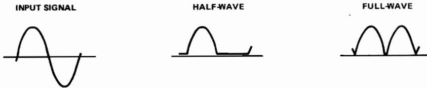
Figure 7.3. Rectifier Output-Voltage Waveforms
