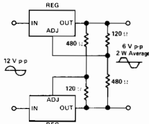
FIGURE 11—A-C VOLTAGE REGULATOR CIRCUIT
