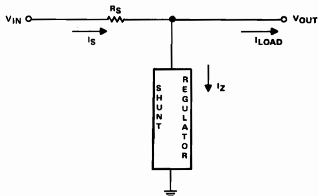
Figure 3.8. Shunt Regulator
