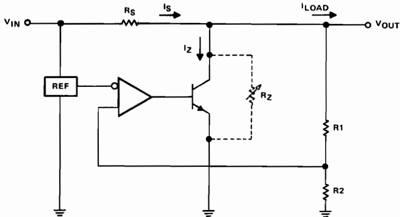
Figure 1.4. Basic Shunt Regulator
