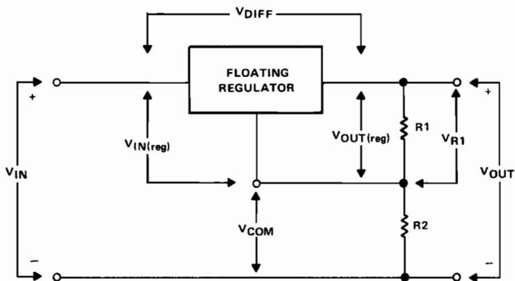
Figure 3.6. Floating Regulator
