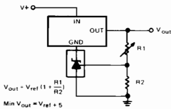
FIGURE 11—OUTPUT CONTROL OF A THREE-TERMINAL FIXED REGULATOR
