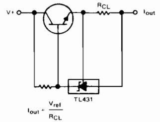
FIGURE 10—CURRENT LIMITER
