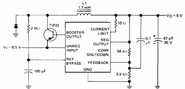
FIGURE 7—SWITCHING REGULATOR
