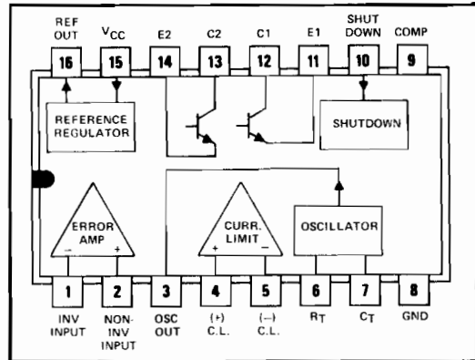
SG1524 . . . J SG2524, SG3524 . . . J OR N DUAL-IN-LINE PACKAGE (TOP VIEW)
