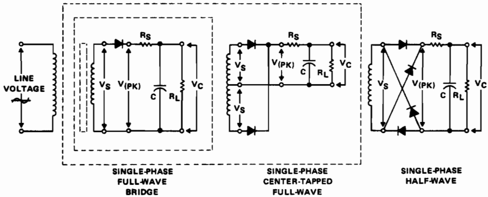
Figure 7.8. Input Filter Design
