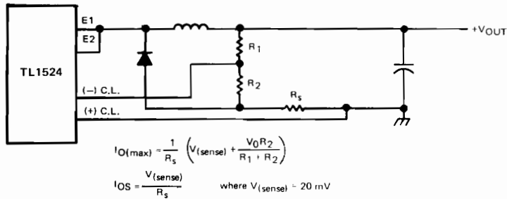
FIGURE 7—FOLDBACK CURRENT LIMITING FOR SHORTED OUTPUT CONDITIONS
