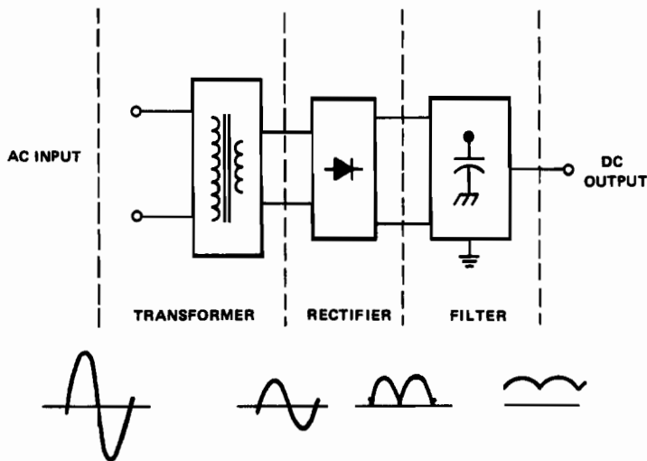
Figure 7.1. Input Supply
