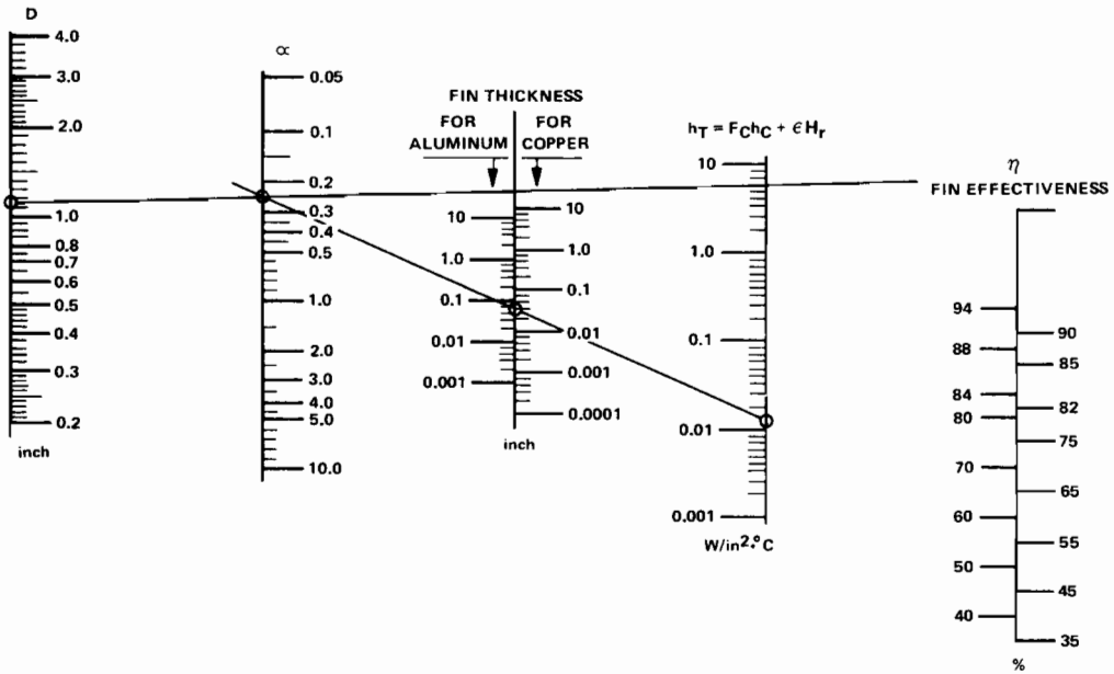
Figure 5.9. Nomograph B – Fin Effectiveness
