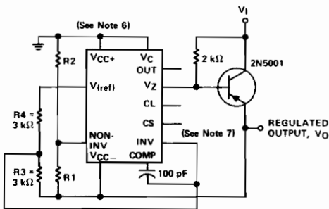
FIGURE 3—NEGATIVE-VOLTAGE REGULATOR
