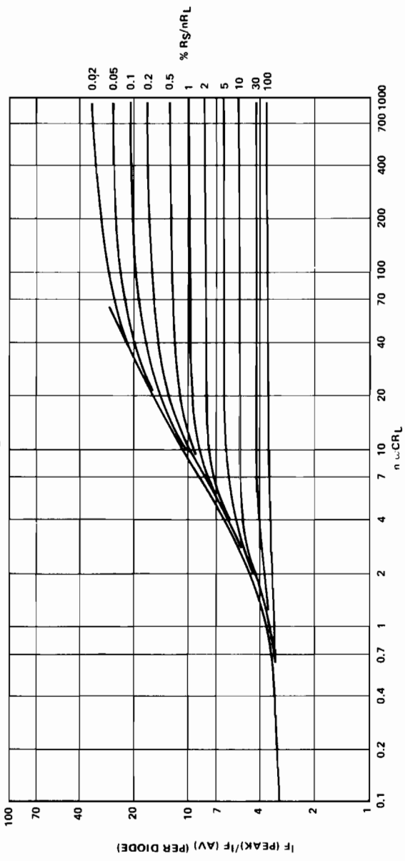
Figure 7.6. Relation of RMS and Peak to Average Diode Current in Capacitor Input Circuits (From O. H. Schade, Proc. IRE, Vol. 31, p. 345, 1943)
