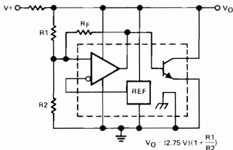
FIGURE 1—SHUNT REGULATOR
