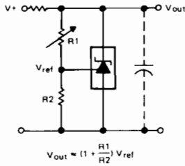
FIGURE 8—SHUNT REGULATOR
