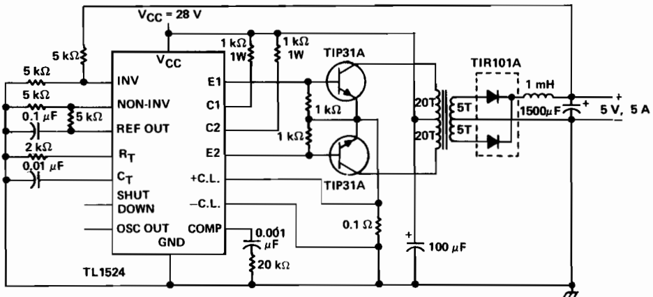
FIGURE 15—PUSH-FULL TRANSFORMER-COUPLED CIRCUIT
