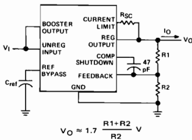
FIGURE 1—BASIC REGULATOR WITH CURRENT LIMITING
