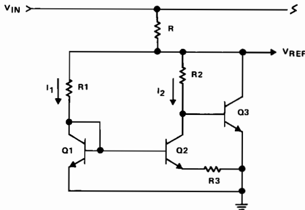
Figure 2.4. Band-Gap Reference
