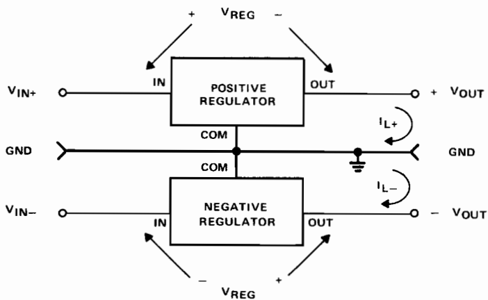
Figure 3.1. Conventional Positive/Negative Regulator
