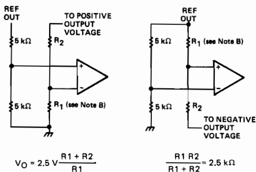
FIGURE 6—ERROR AMPLIFIER BIAS CIRCUITS
