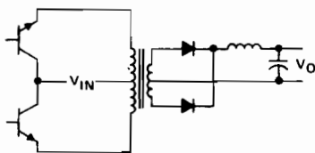
PUSH PULL
