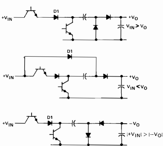
FIGURE 9—CAPACITOR-DIODE-COUPLED VOLTAGE-MULTIPLIER OUTPUT STAGES
