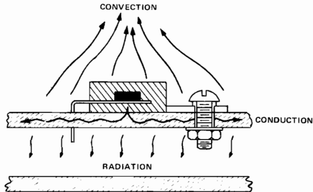
Figure 5.3. Heat Flow Paths of Semiconductor Cooling
