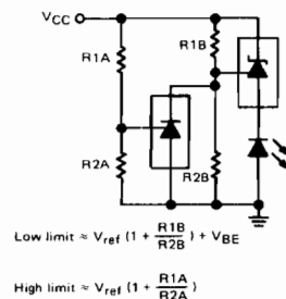
FIGURE 15—V CC MONITOR
