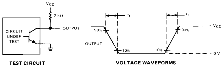
FIGURE 2—SWITCHING TIMES
