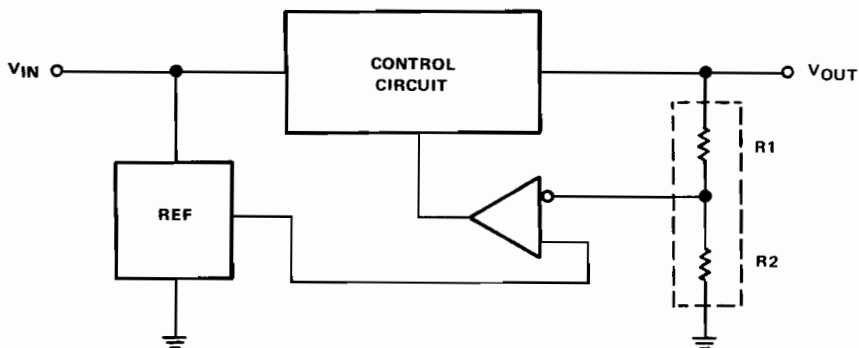
Figure 2.5. R_1/R_2 Ladder Network Sampling Element
