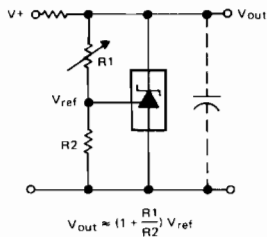
FIGURE 8—SHUNT REGULATOR
