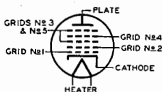
Pentagrid Converter
