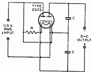
VOLTAGE-DOUBLER CIRCUIT
