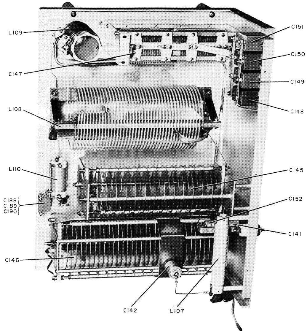
Figure 6-7. Output Network Parts Arrangement, Bottom View
