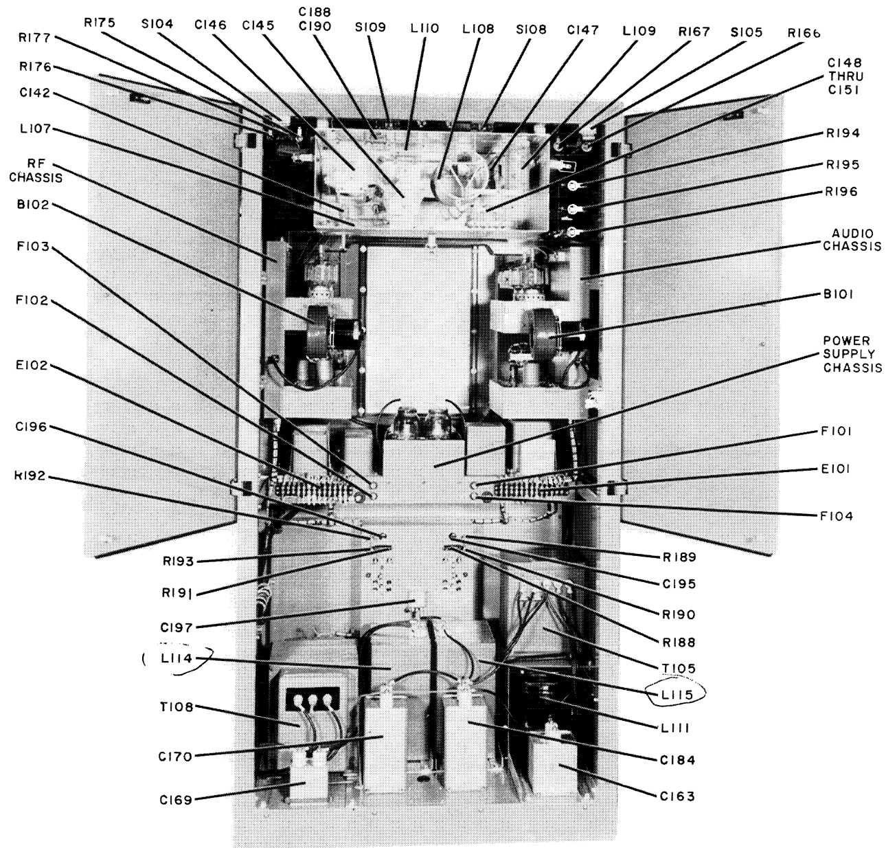
Figure 6-2. Transmitter Parts Arrangement, Rear View
