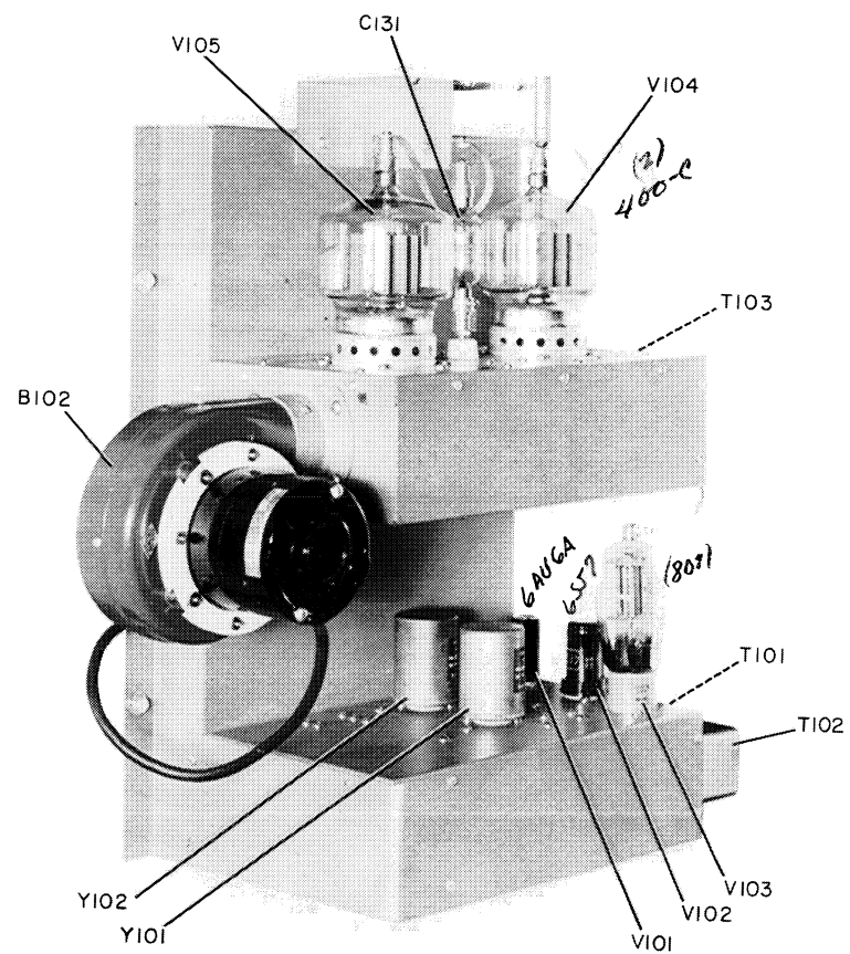
Figure 6-3. R-F Chassis Parts Arrangement
