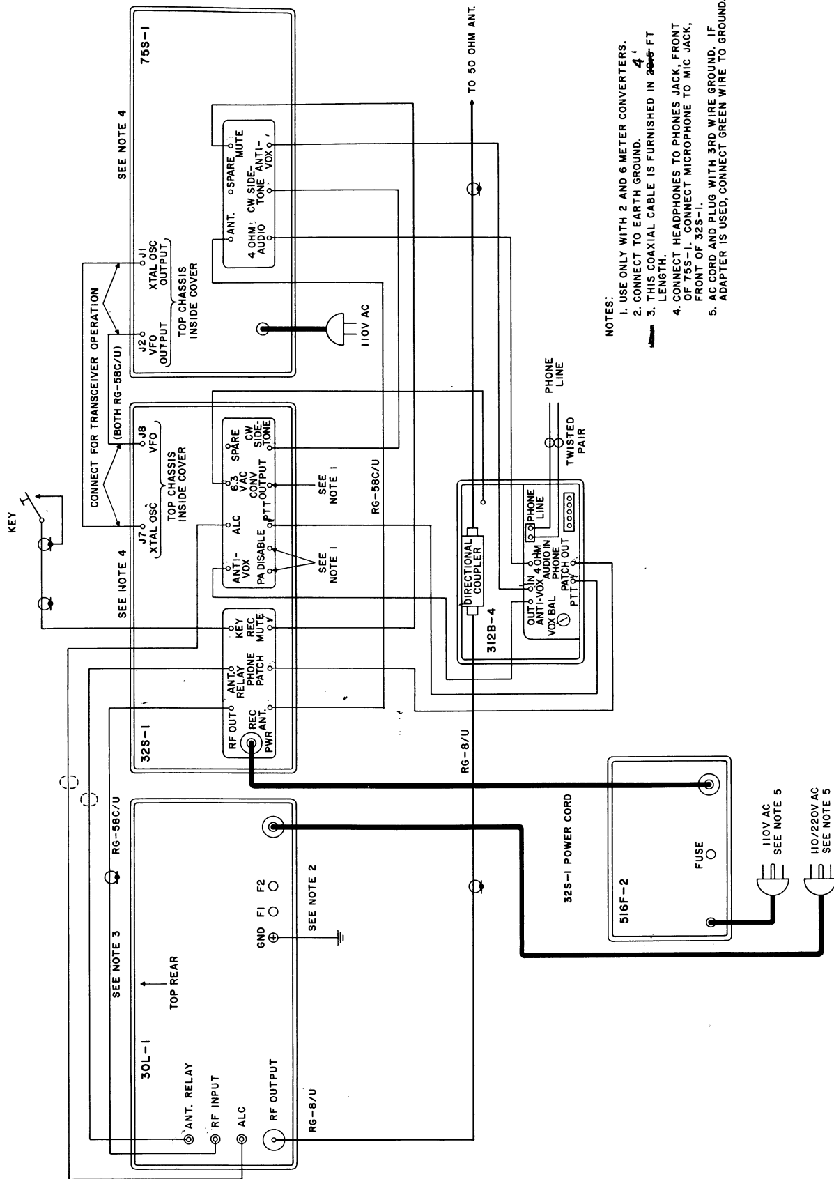
Figure 1-4. Interconnections with S-Line
