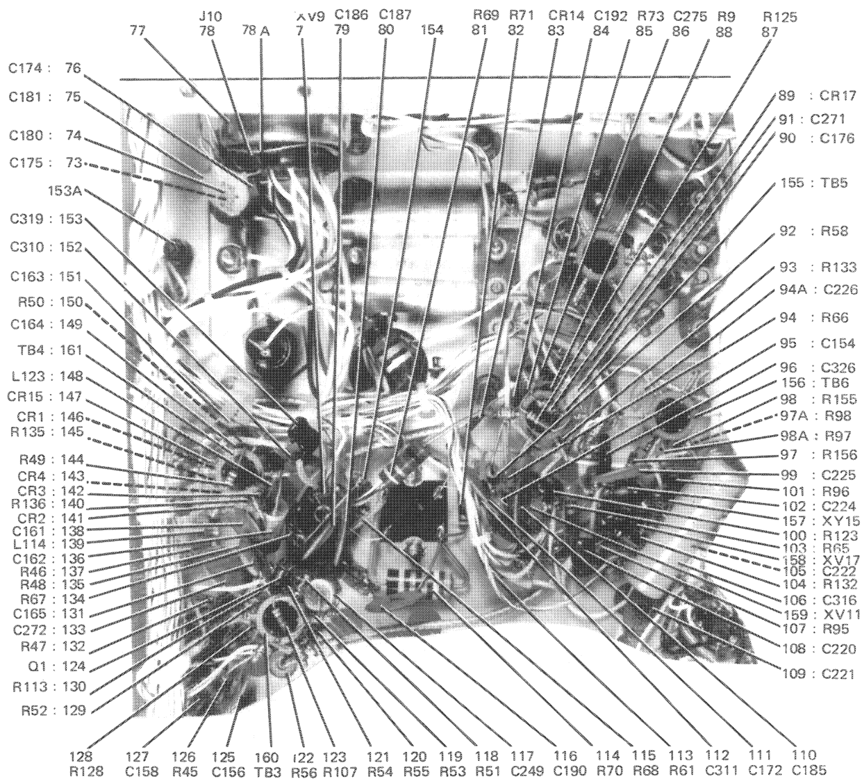
DETAIL B
