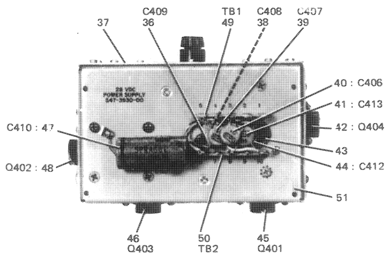
BOTTOM VIEW
