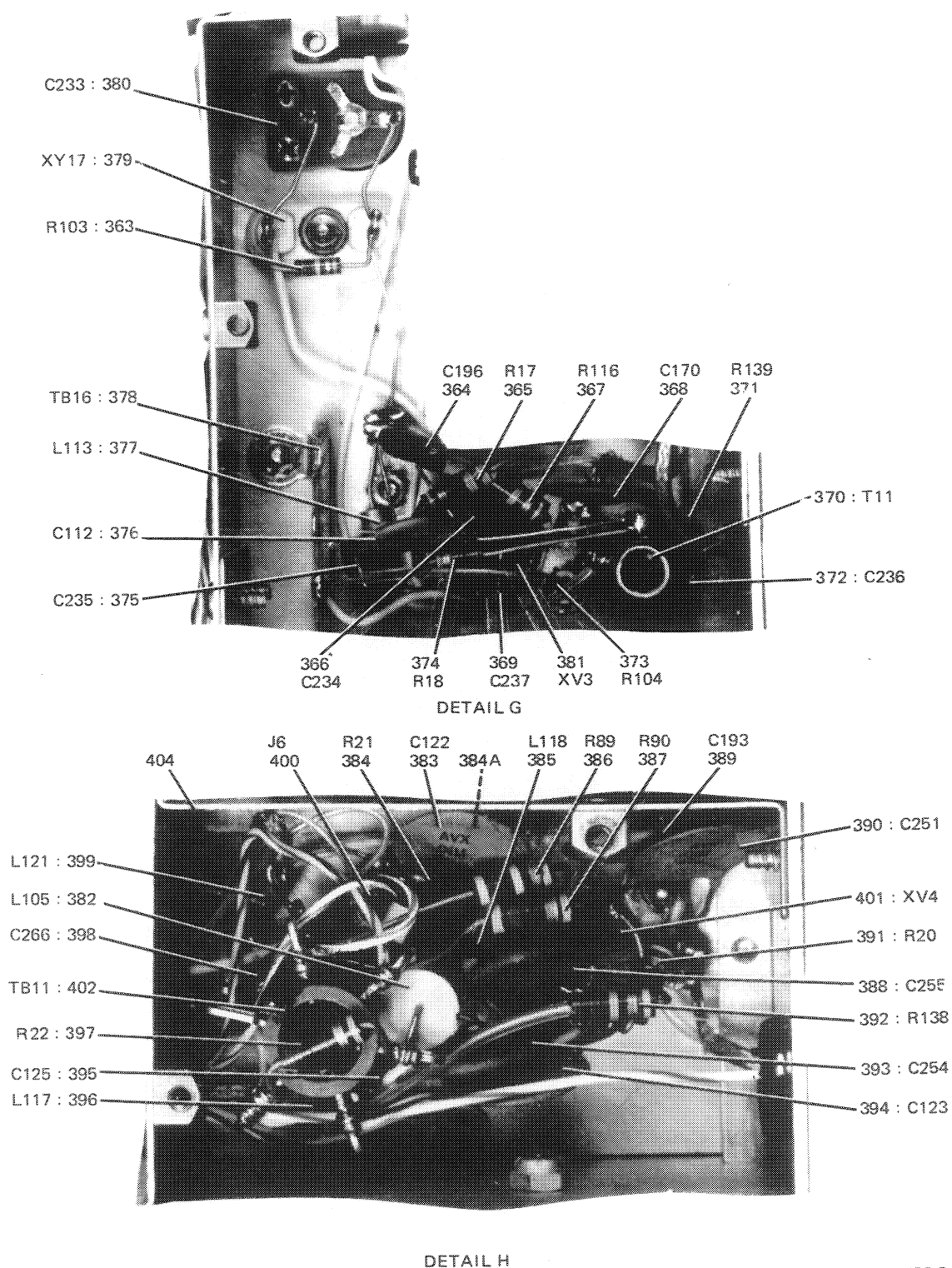
Receiver Subassembly Figure 6-3 (Sheet 8)
