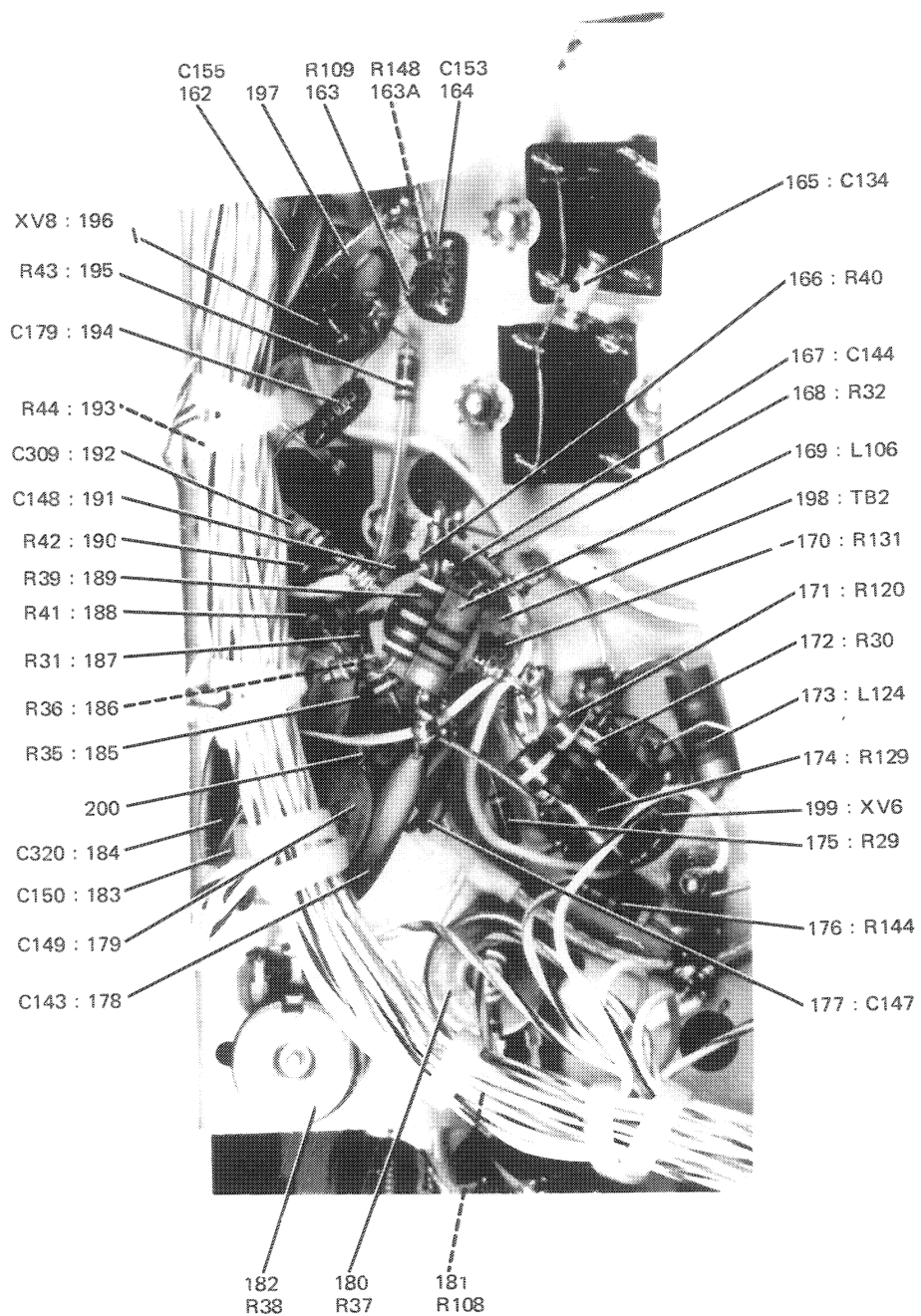
DETAIL C
