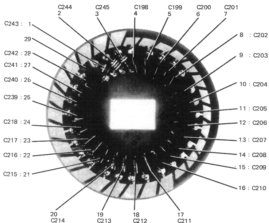
Crystal Oscillator Capacitor Assembly (A8) Figure 6-12
