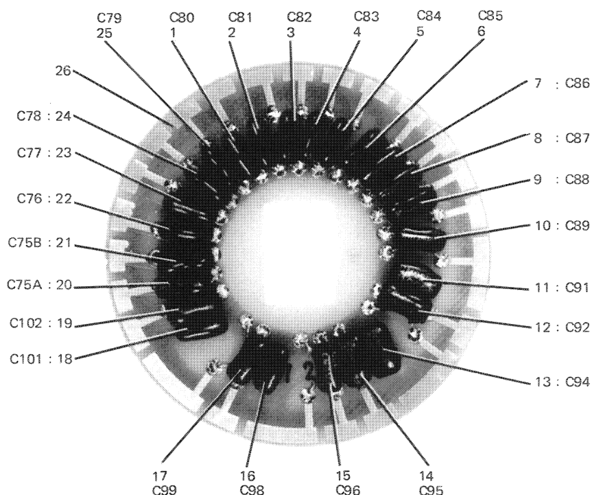
Capacitor Assembly (A7) Figure 6-11
