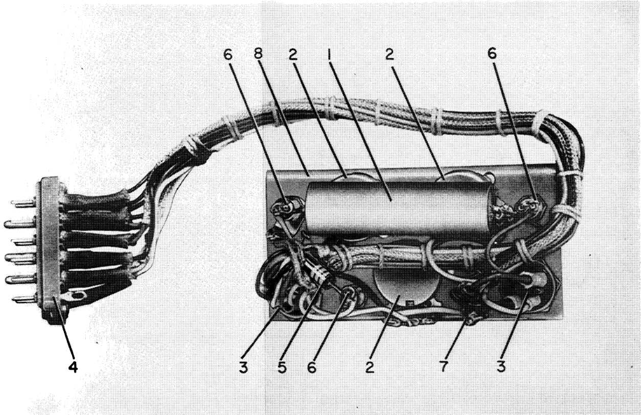
Figure 9. Sidetone Control
