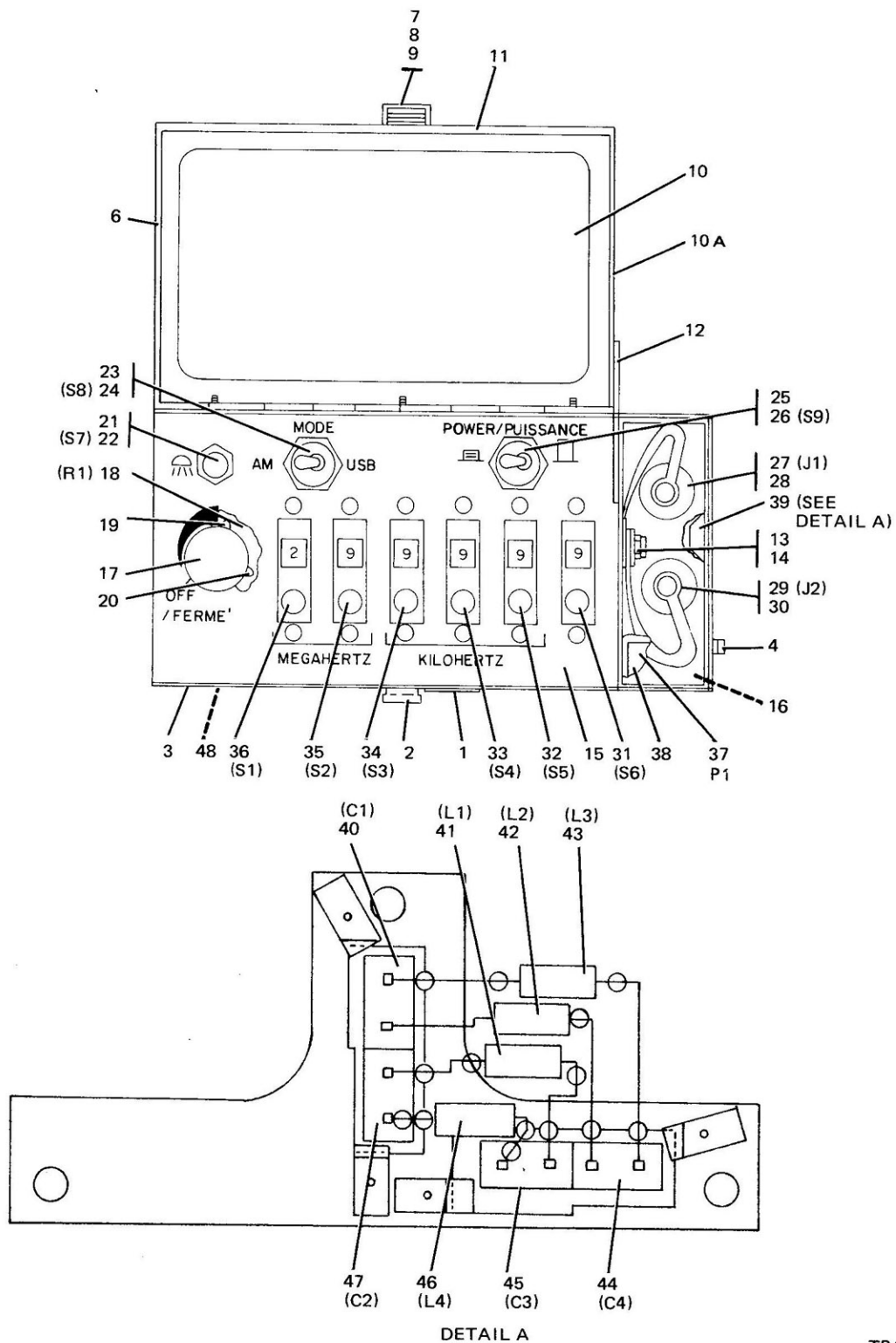
Figure 3-34. Receiver-Transmitter Control C-5310/URC A2
