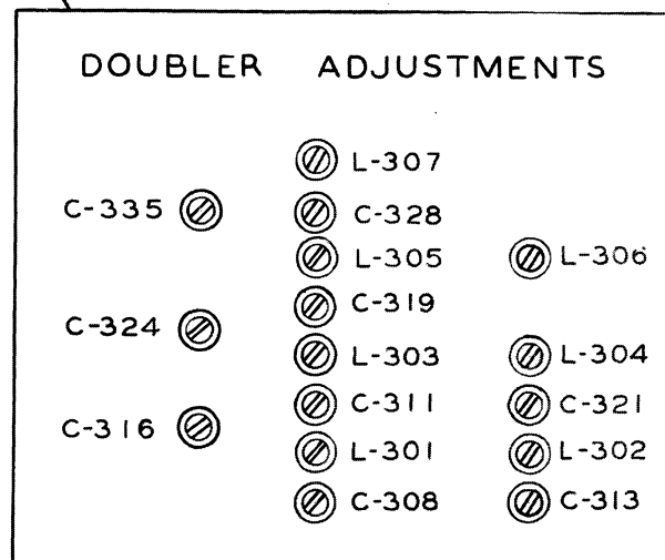
Figure 6-4. Location of RF Unit Adjustments
