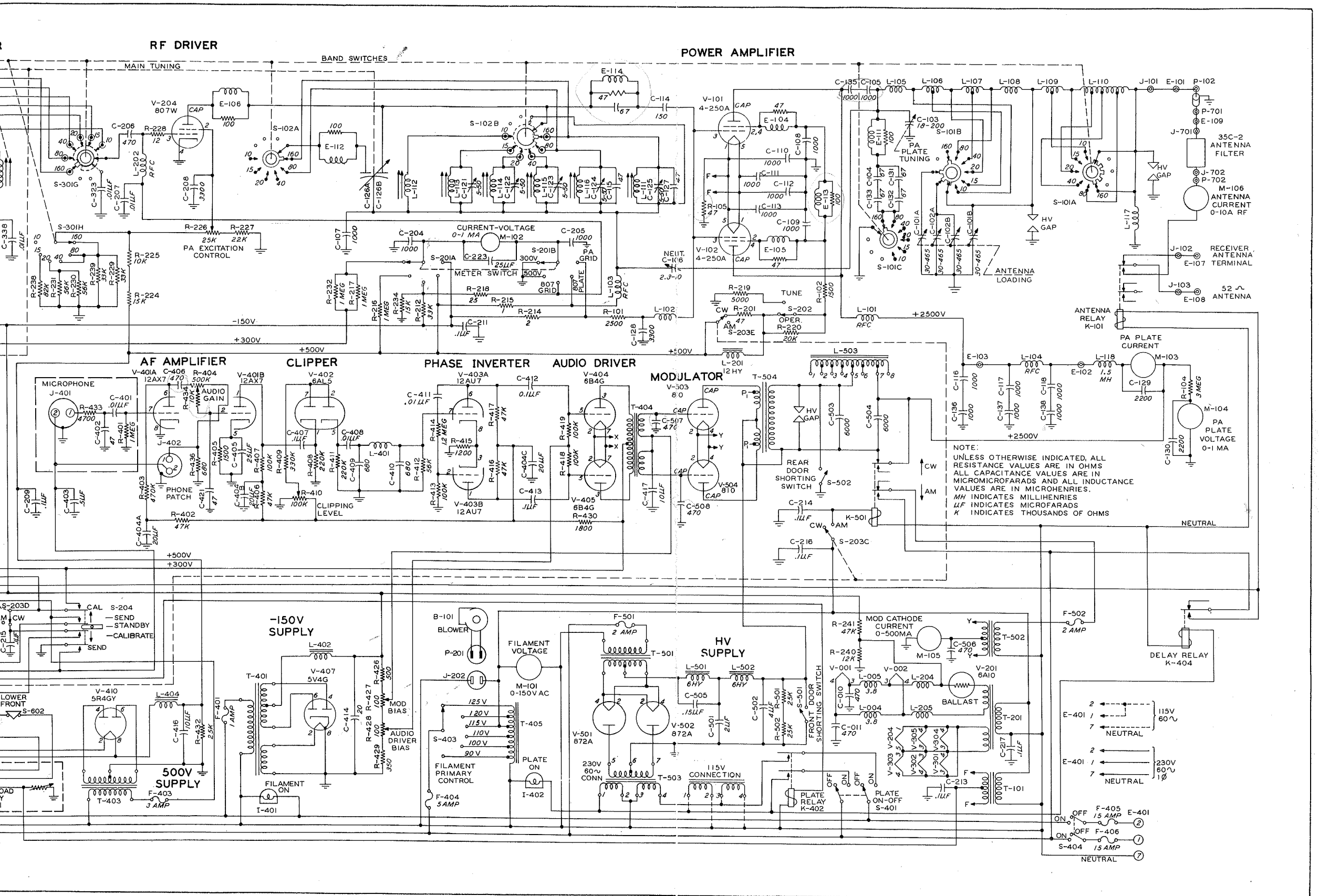
Figure 7-4. KW-1 Main Schematic
