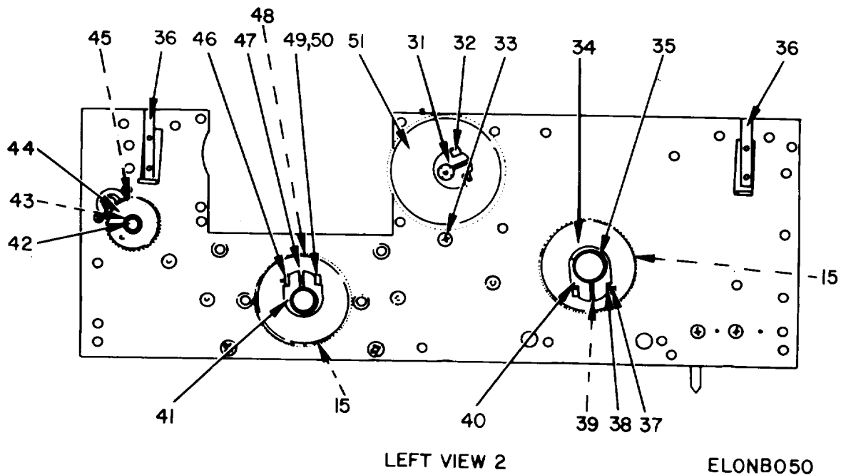
Figure 50. Radio Frequency Translator, Top View 3, Left View 2.
