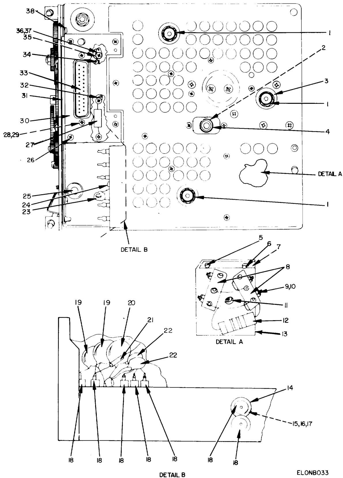
Figure 33. Amplifier Radio Frequency, Bottom View.
