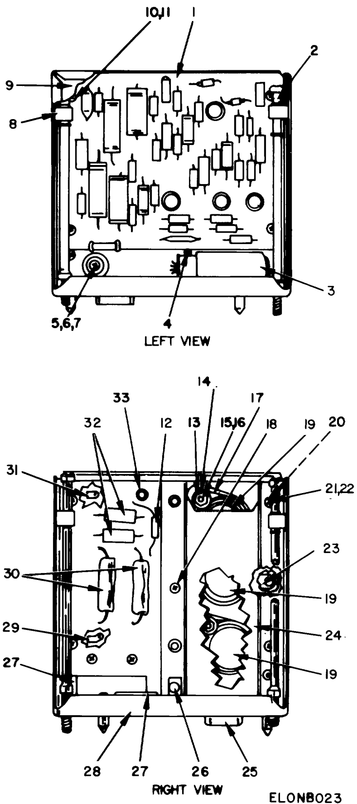
Figure 23. Amplifier.
