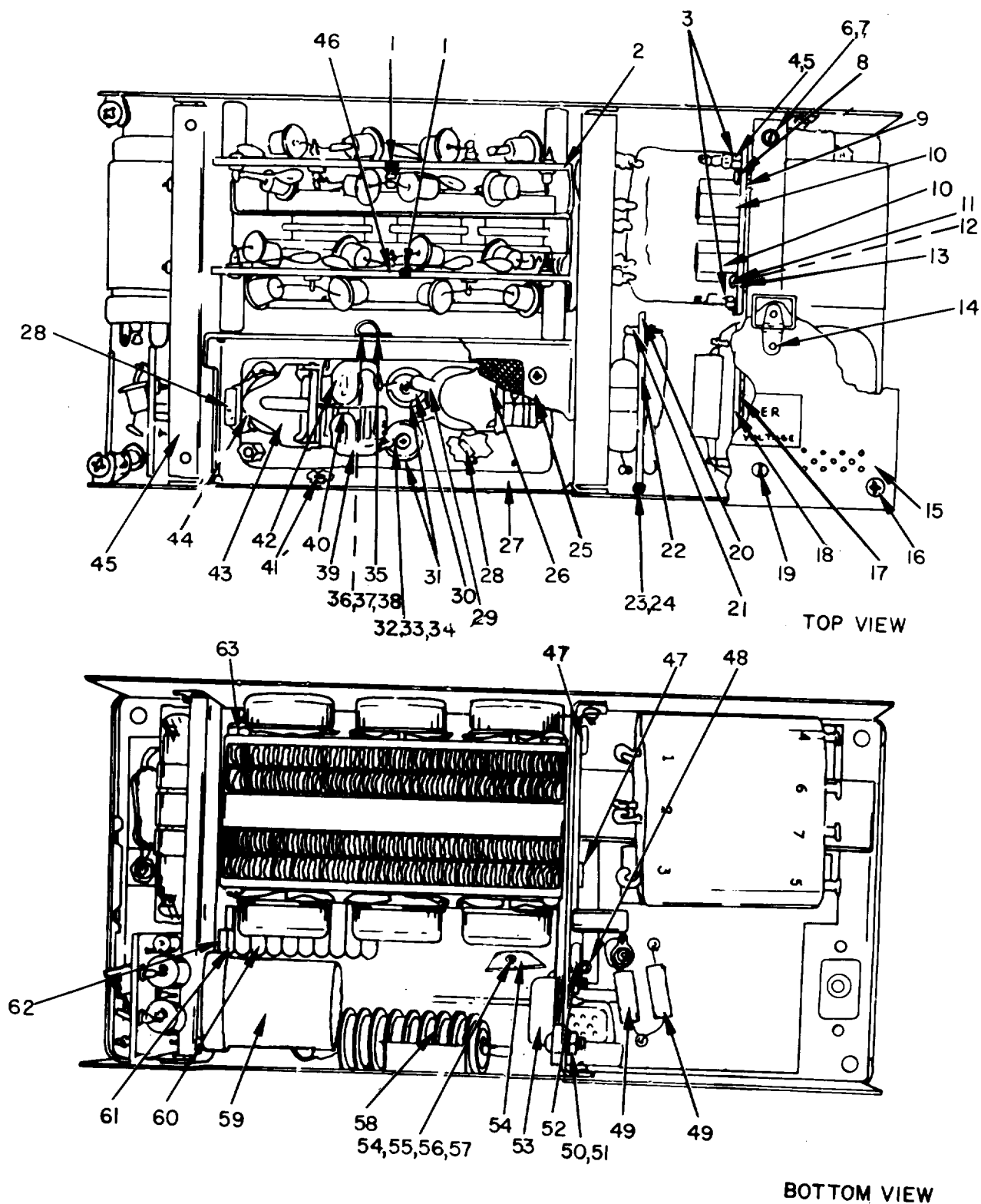
Figure 26. High Voltage Power Supply Module, Top and Bottom View.
