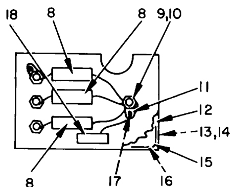
DETAIL A, BOTTOM VIEW ELONB051
