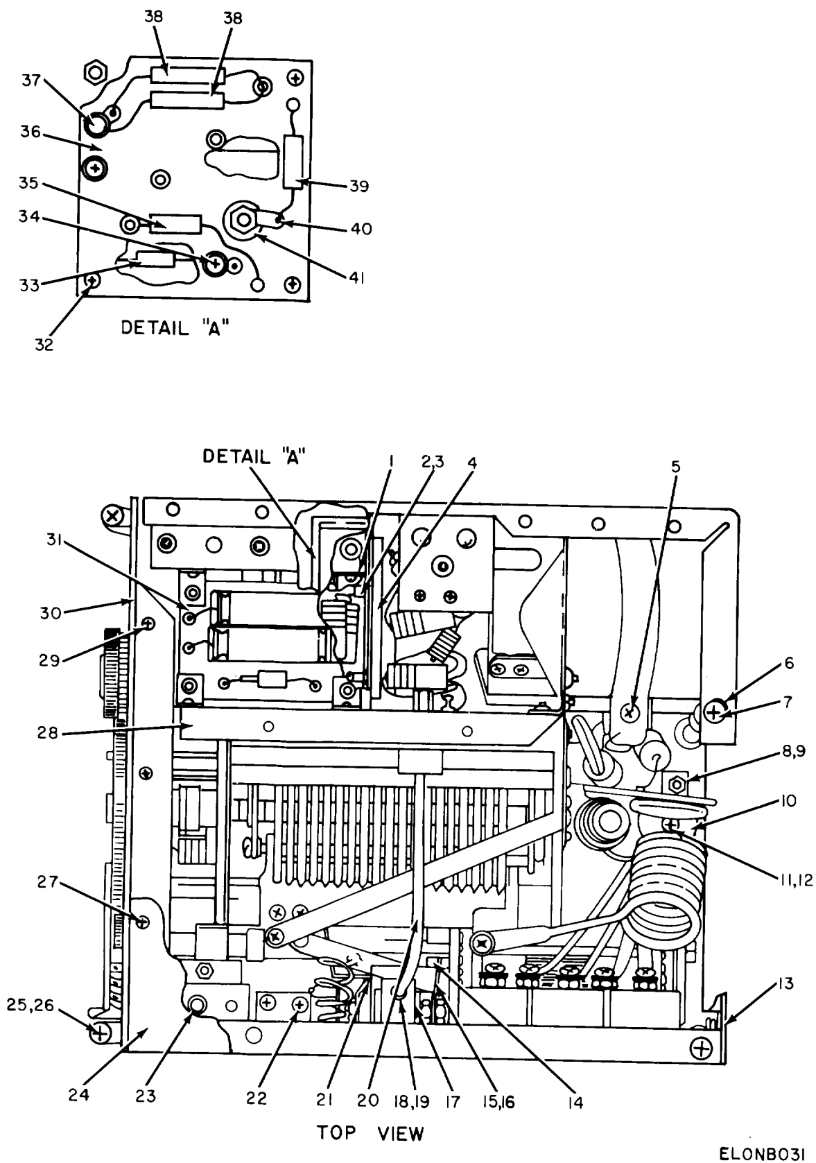
Figure 31. Amplifier Radio Frequency.
