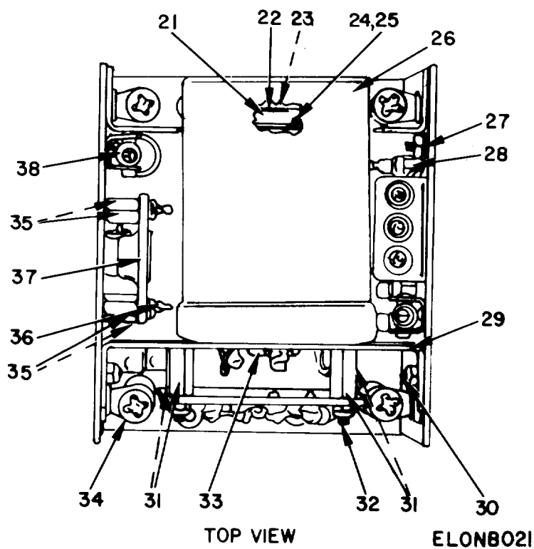
Figure 21. Low Voltage Power Supply Module.
