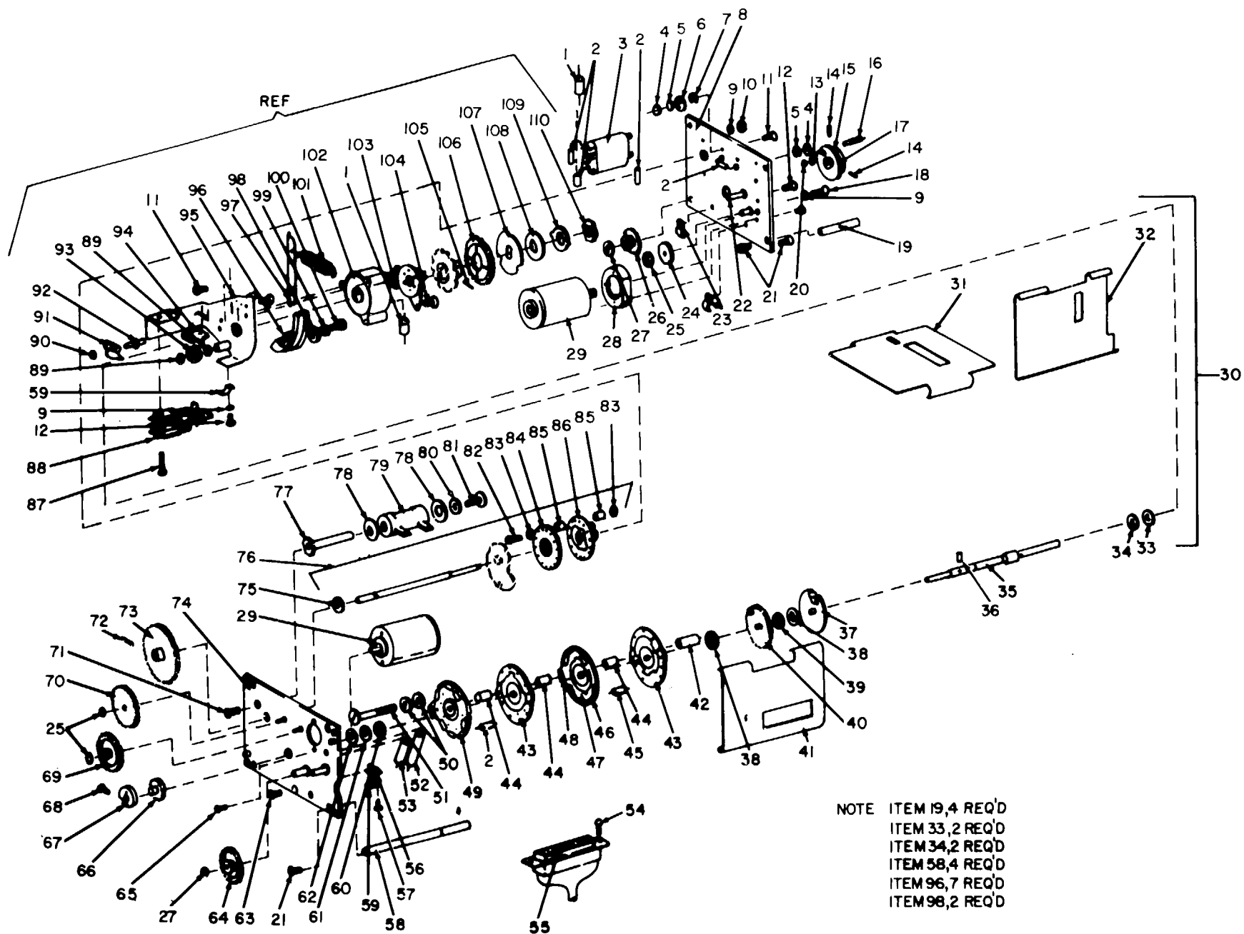
Figure 56. Autopositioner Submodule.
