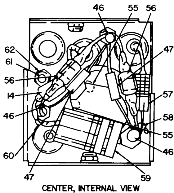
Figure 4. Chassis Assembly, Front and Center Internal Views.
