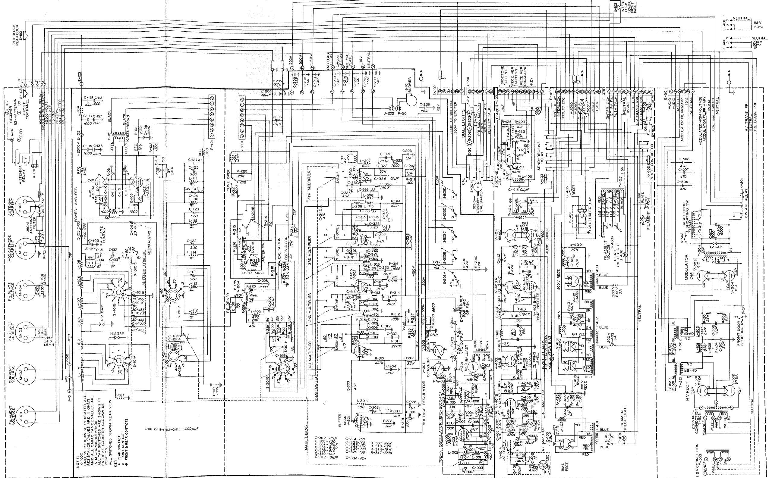
Figure 7-3. KW-1 Cabling Diagram
