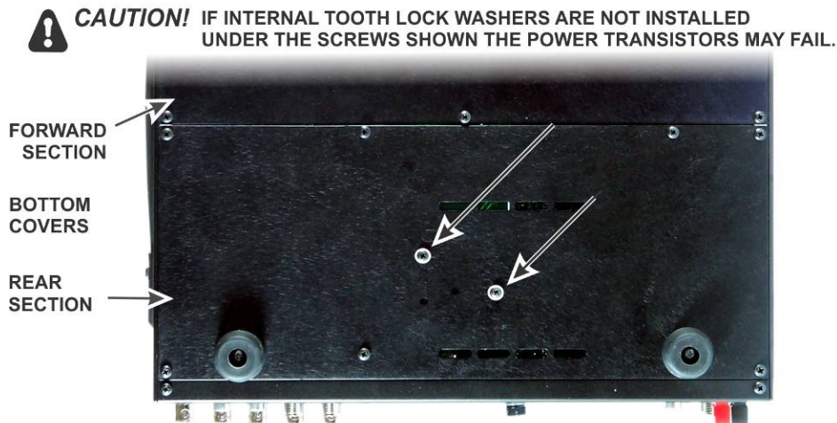
Figure 99. Checking Power Transistor Mounting Hardware.
