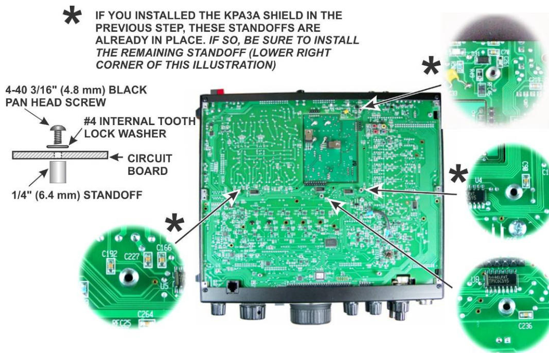
Figure 91. Installing Standoffs on RF Board.
