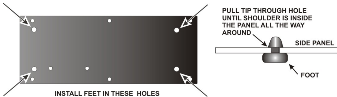
Figure 70. Installing Side Panel Feet.
