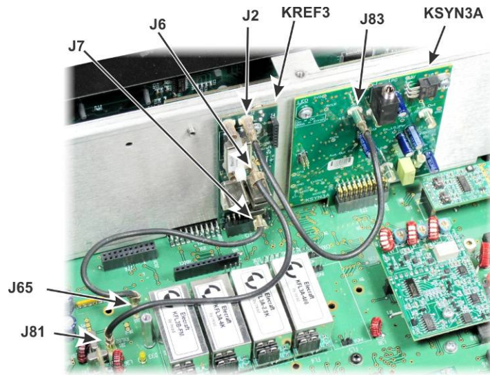
Figure 82. Installing KREF3 TMP Cables.
