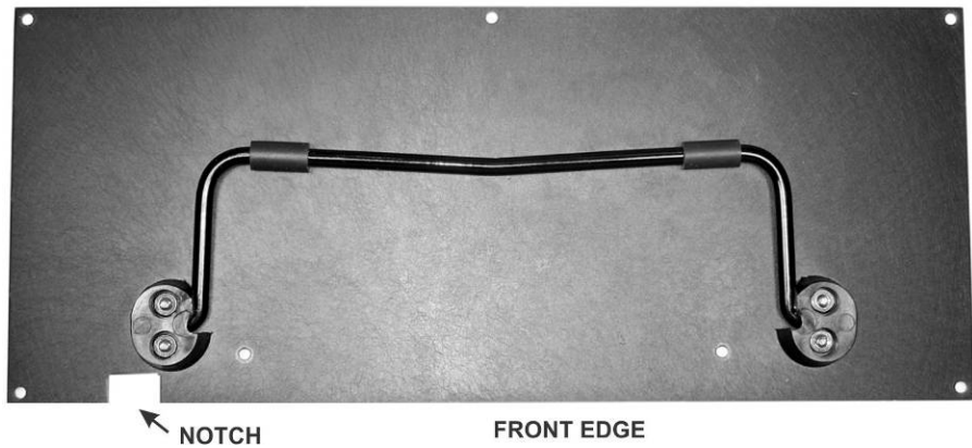
Figure 92. Installing Tilt Stand.
