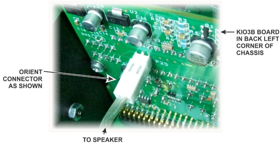
Figure 100. Connecting Speaker to KIO3B Board.
