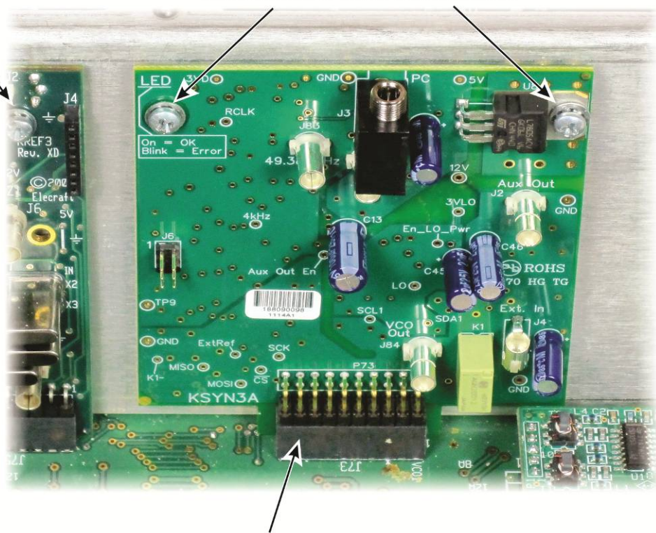
Figure 80. Installing the KSYN3 Board.
