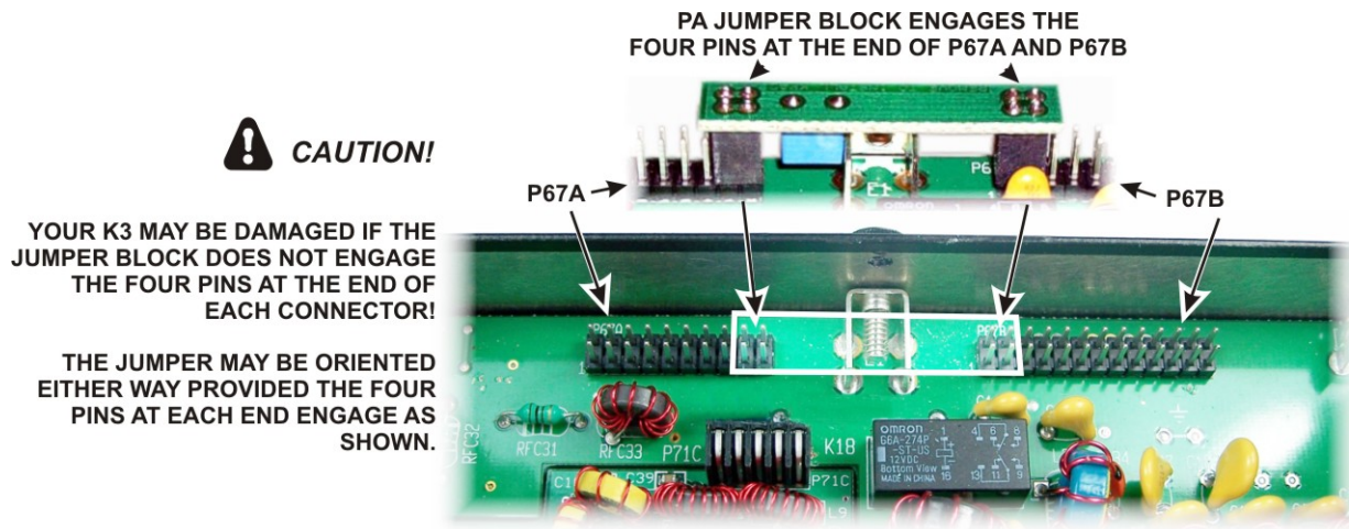
Figure 95. Installing the PA Jumper Block.
