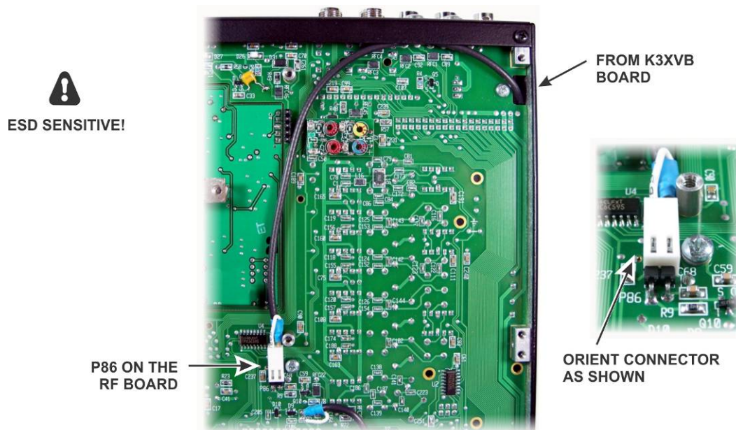
Figure 66. Routing the KXV3B Cable to P86.
