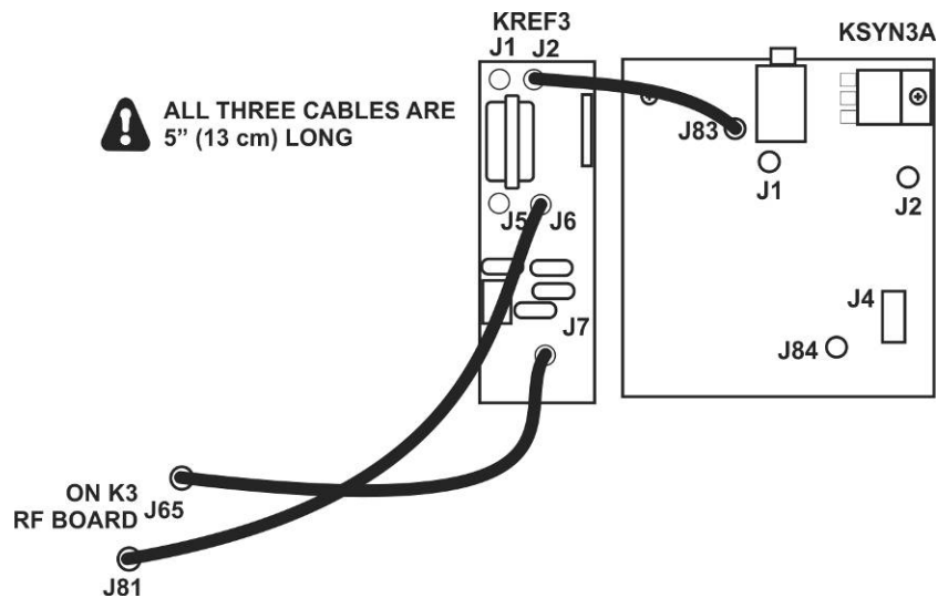
Figure 83. KREF3 TMP Cable Connections, Pictorial View.
