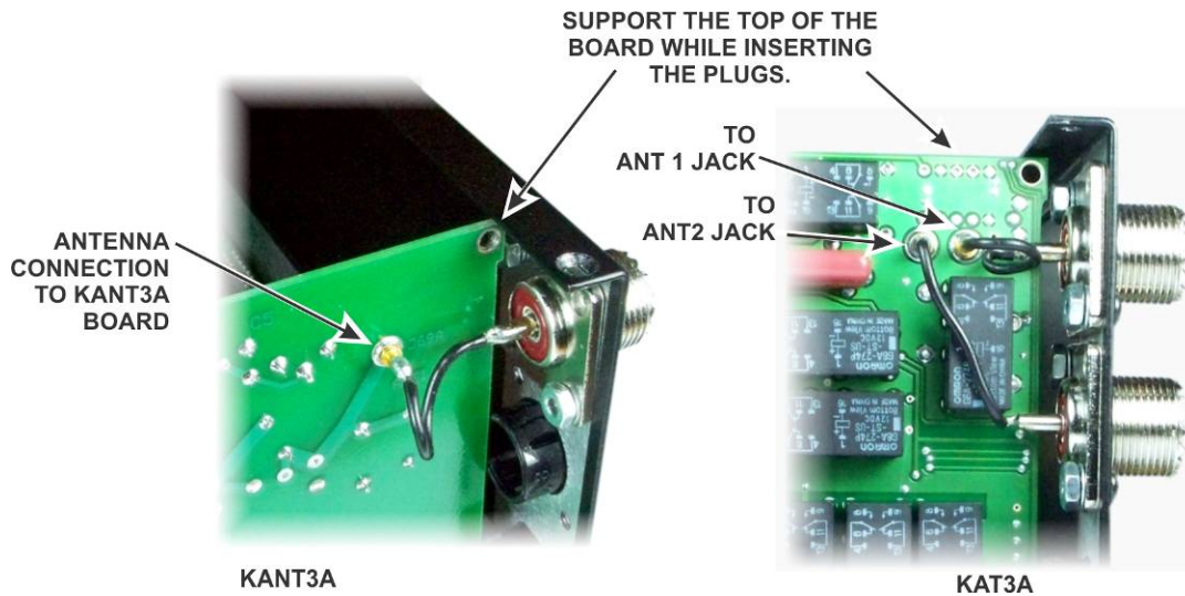
Figure 69. ANT Connections to KANT3A or KAT3A Boards.
