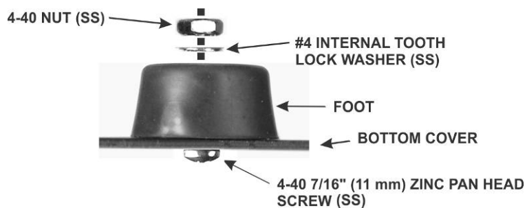
Figure 93. Installing Rear Feet.
