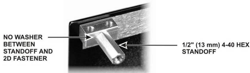
Figure 72. KAT3A/KANT3A Mounting Standoff.
