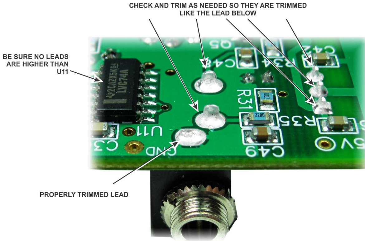
Figure 79. Trimming the Synthesizer Leads.
