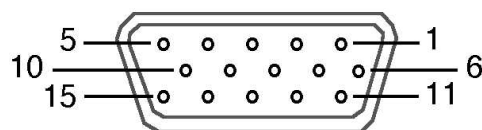
ACC Connector (female, on KIO3B panel)
