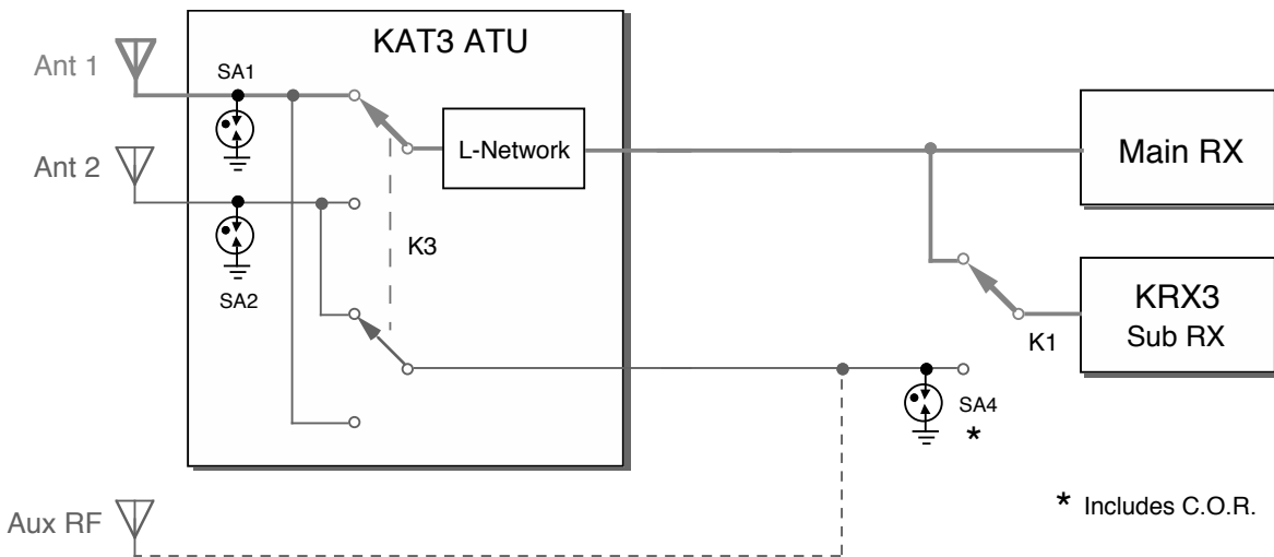
Figure 3. KAT3A ATU Antenna Routing
