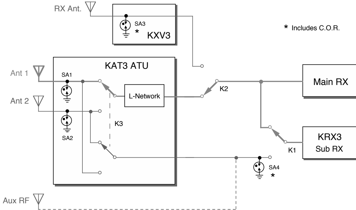
Figure 4. Complete Main/Sub Receiver Antenna Routing
