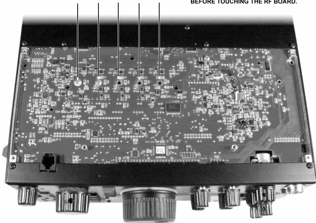
FILTER MOUNTING SCREW LOCATIONS (TWO FILTERS INSTALLED)
