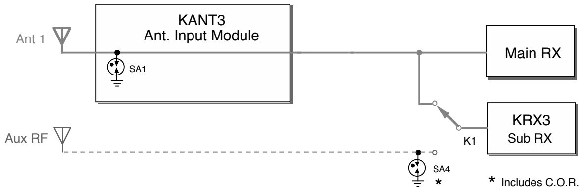
Figure 1. Basic Main/Sub Receiver Routing (no KAT3A)
