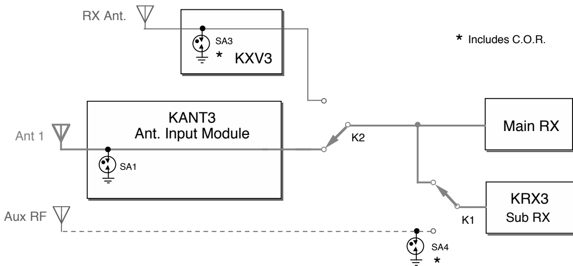
Figure 2. Main/Sub Receiver Routing Including RX ANT IN on KXV3B Module
