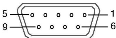
RS232 adapter cable DE9 connections (female)
