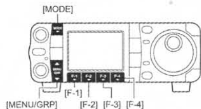
[MENU/GRP] [F-1] [F-2] [F-3] [F-4]
