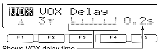
Shows VOX delay time
