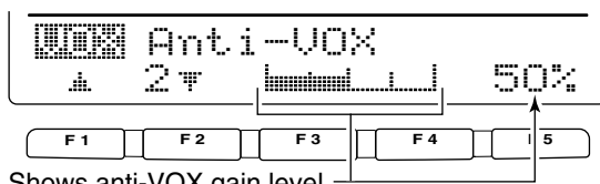
Shows anti-VOX gain level
