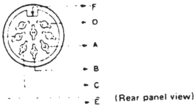
•Using the MIC CONNECTOR
