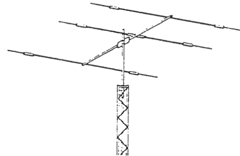
• Multi-band Yagi beam antenna
