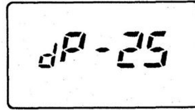
25 kHz tuning step
