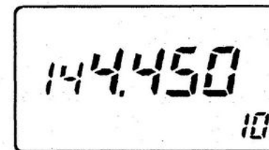
The display shows that the lock function is OFF.
