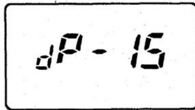
15 kHz tuning step
