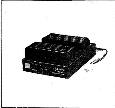
IC-50L LINEAR AMPLIFIER 50MHz 10W
