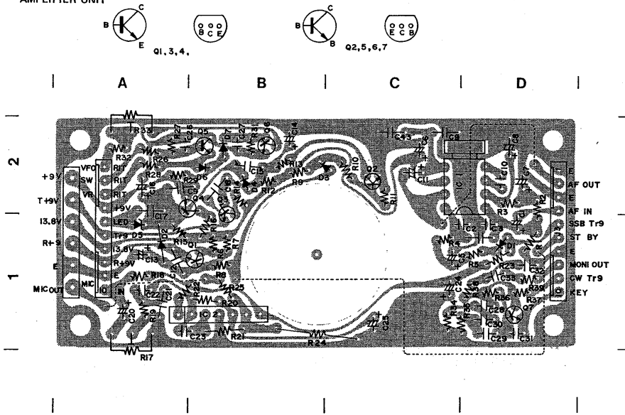
AMPLIFIER UNIT
