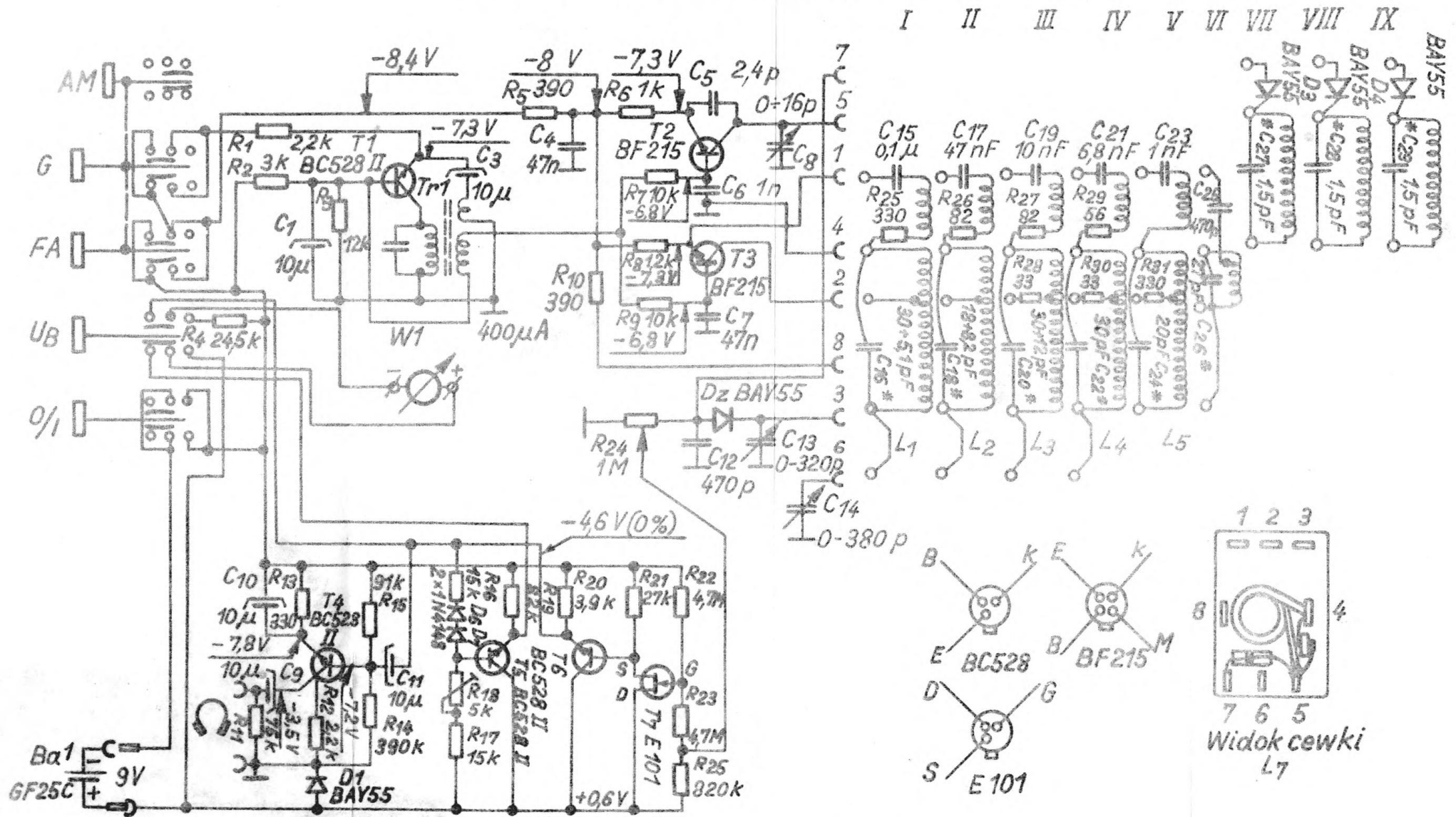
Rys.1 Schemat ideowy RUG-4 Draw.1 Circuit diagram of RUG-4
