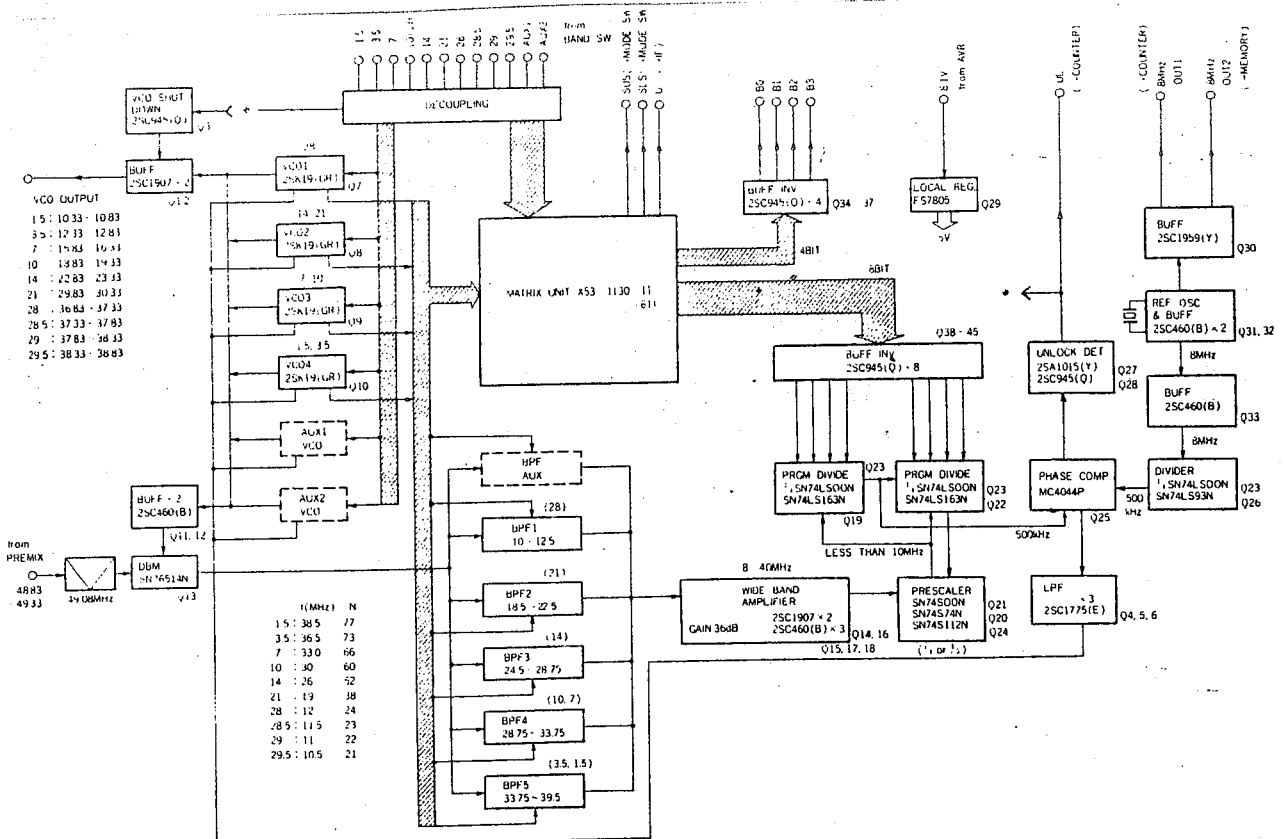
Fig. 6-5 PLL Circuit
