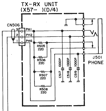
TS-60(K,E) (TX-RX UNIT)
