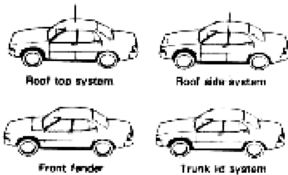
Installation for mobile operation
