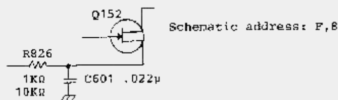
SIDETONE MIXER
