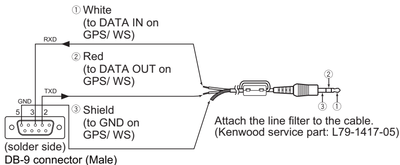
Figure 4-3 Cable Connection Example (Garmin GPS18xPC)
