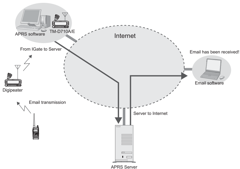
Figure 7-4 Transmission Flow for Email
