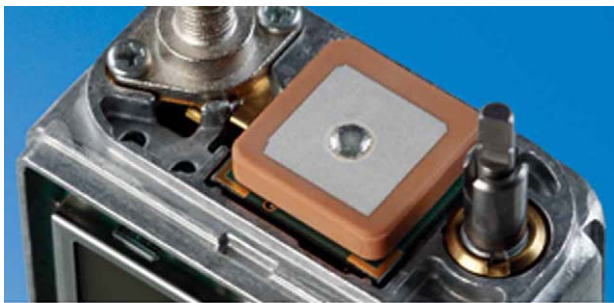
Internal GPS unit
