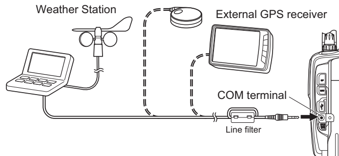
Figure 4-2 Connection Example of GPS Receiver
