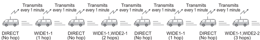
Figure 6-2 Example of path switchover operation of Proportional Pathing (when the packet path is set to WIDE1-1, WIDE2-2)
