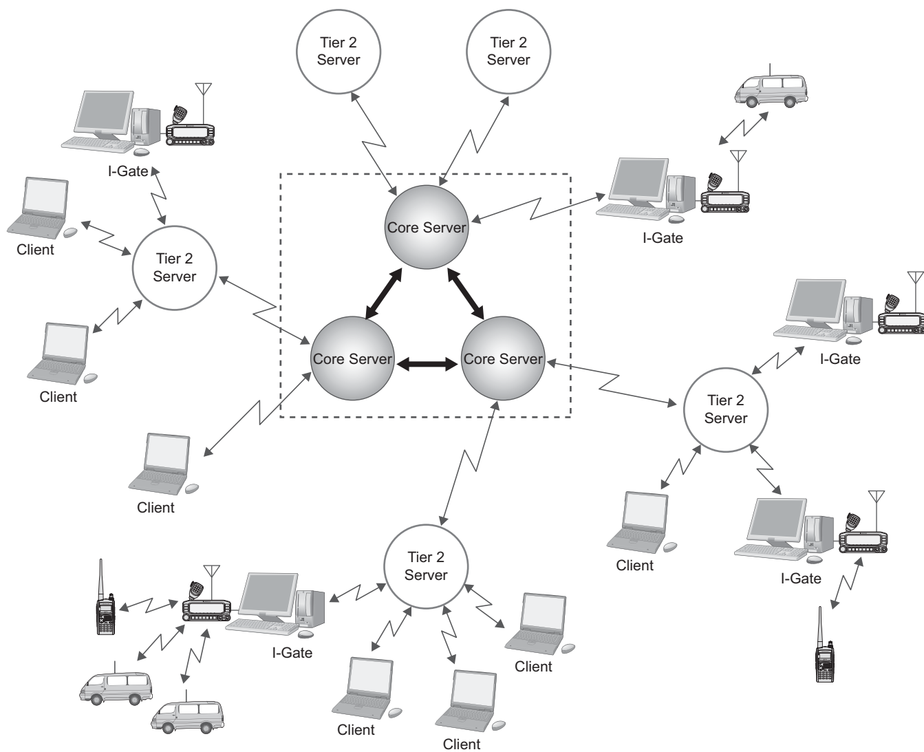
Figure 7-1 APRS Network Conceptual Drawing
