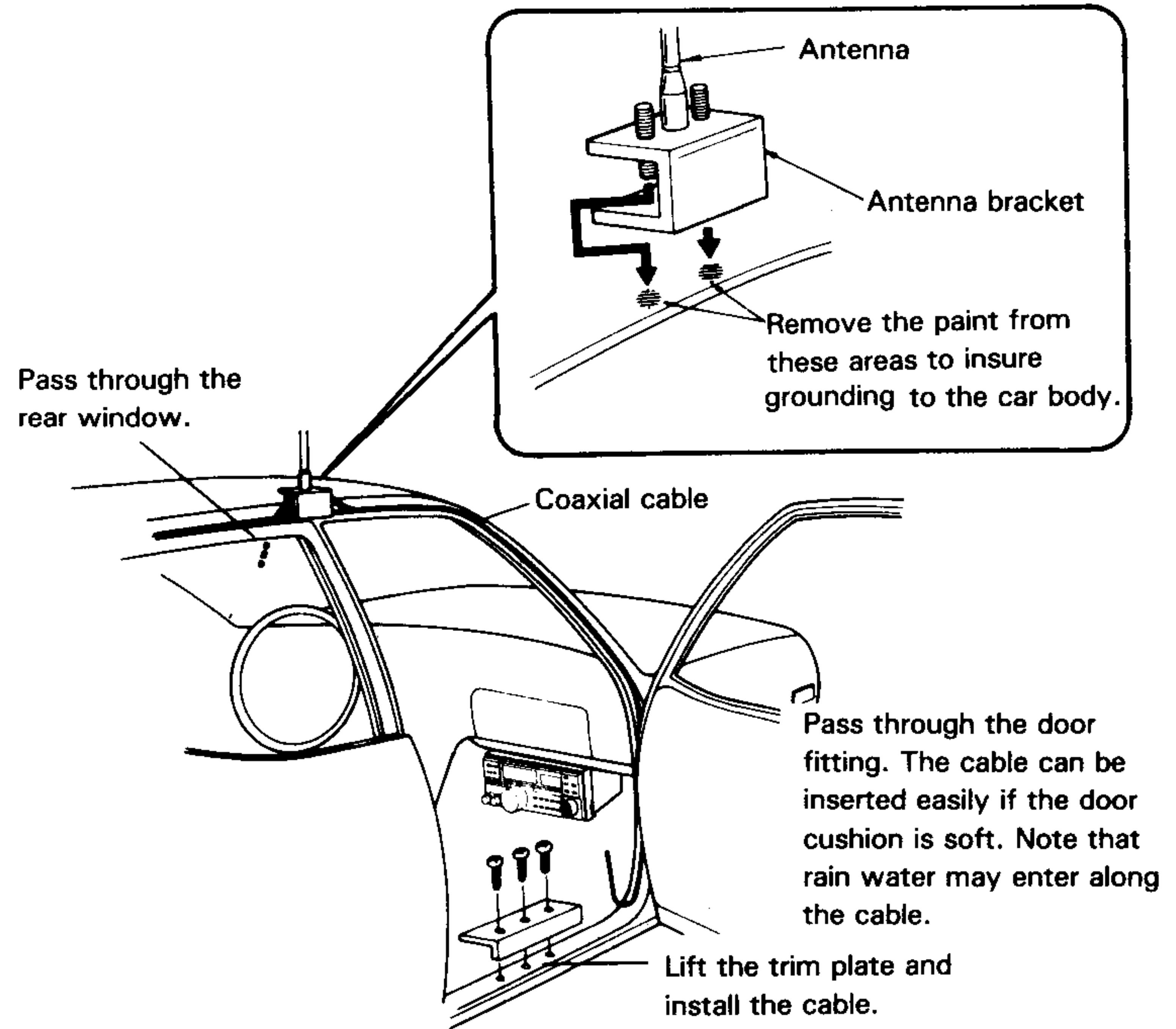
Coax. cable routing
