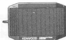
TH-7 144/430 MHz FM Dual Bander (General only)
