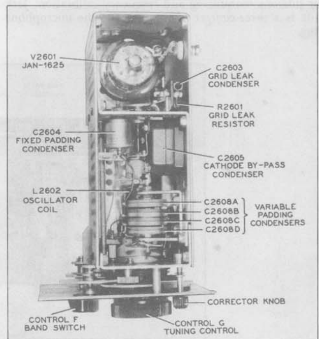
Figure 12. Oscillator O-17/ART-13A, Showing Top-Cover Plate Removed
