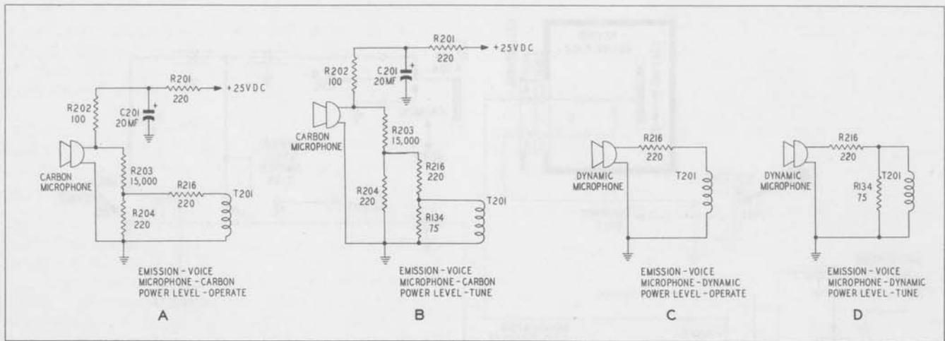
Figure 31. Microphone Circuits
