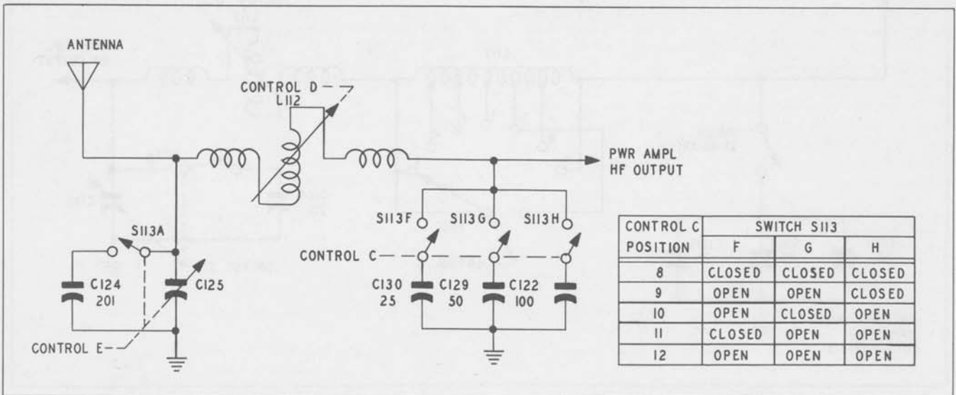
Figure 27. High-Frequency Output Circuit for Positions 8 through 12 of Control C
