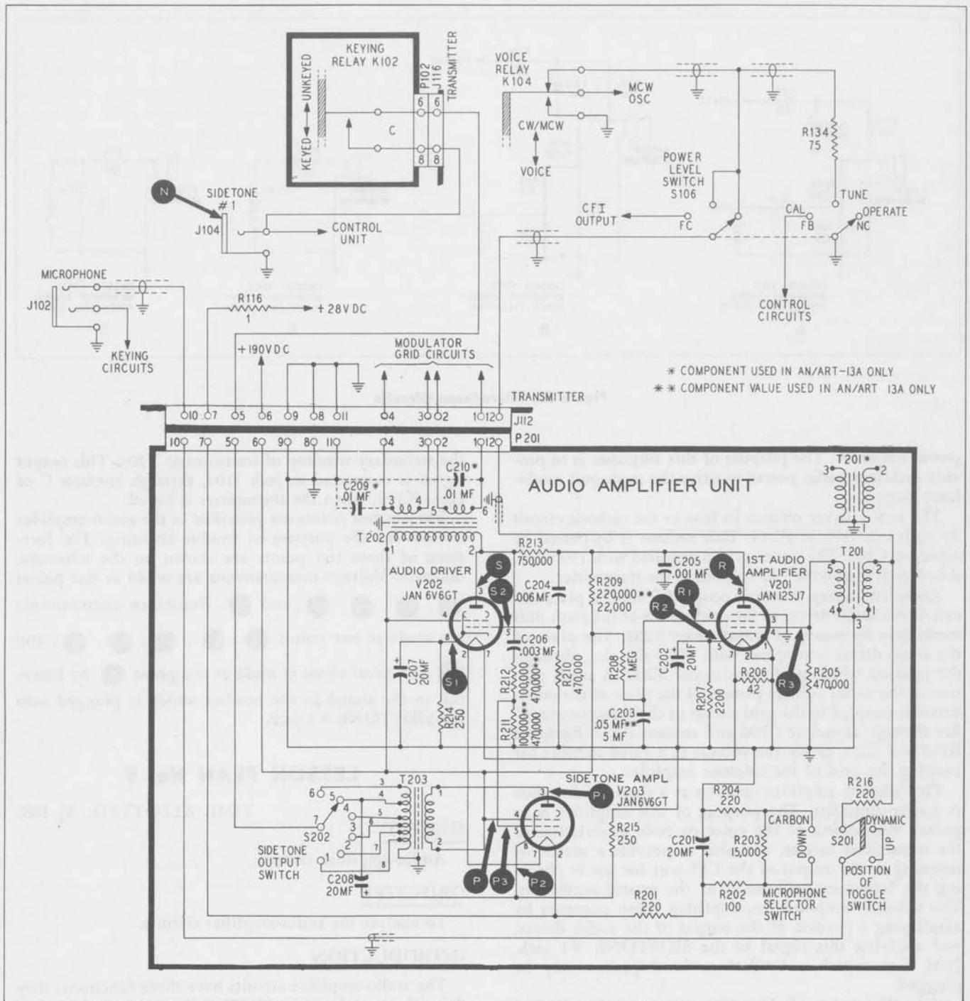
Figure 30. Audio-Amplifier Circuits
