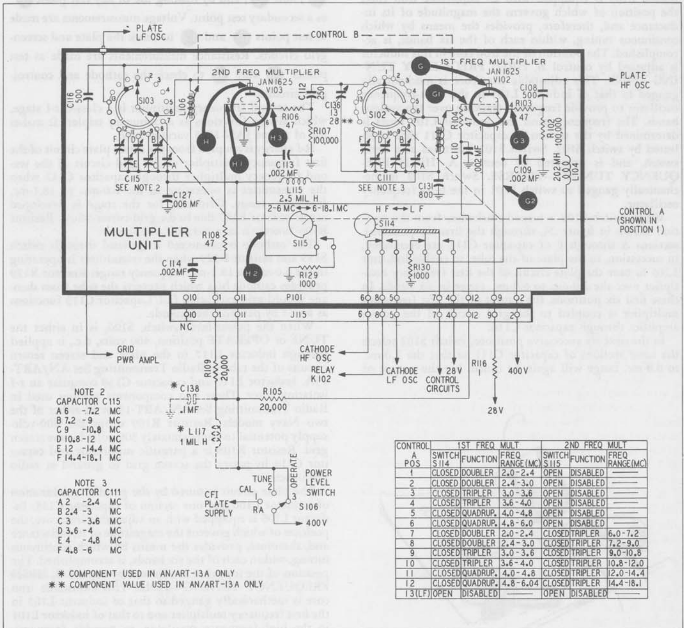
Figure 24. Frequency-Multiplier Circuits
