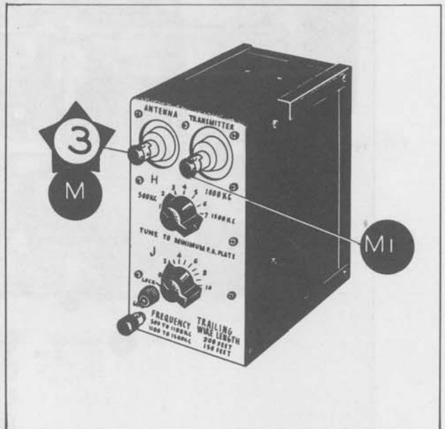
CU-26/ART-13 Type Antenna Loading Coil
