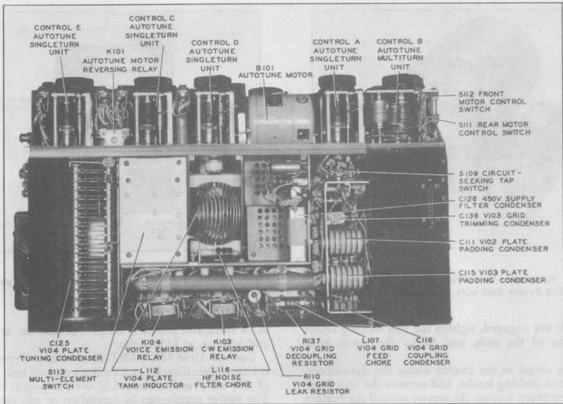
Figure 13. Radio Transmitter T-47A/ART-13, Showing Bottom-Cover Plate Removed
