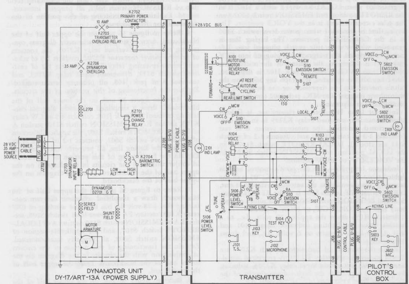
Figure 36. Power-Control Circuits
