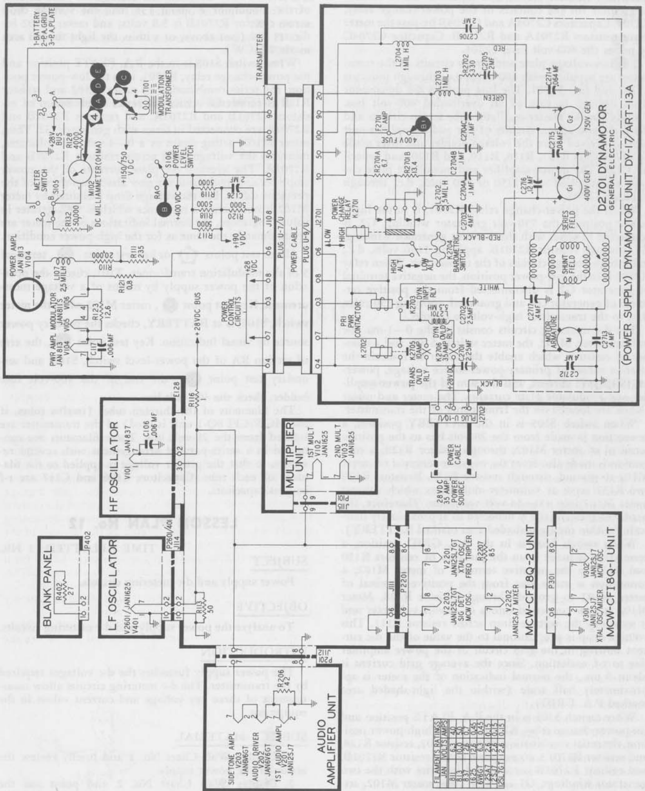
Figure 35. Power-Supply and D-C Metering Circuits
