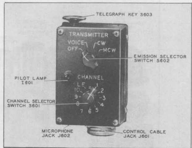
Figure 16. Control Unit C-87/ART-13 or Navy Type —23330
