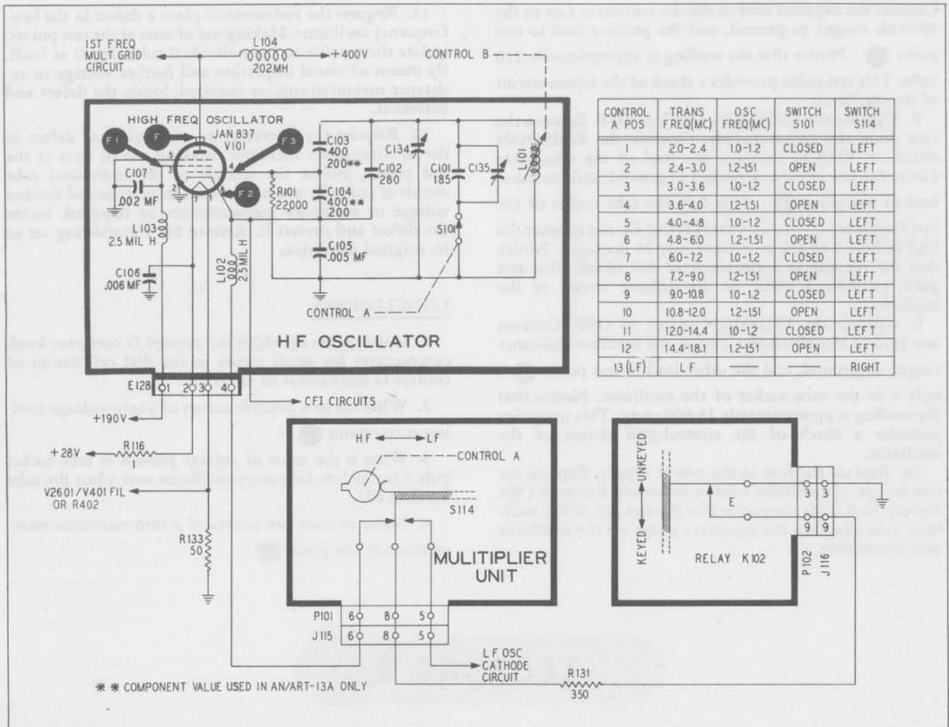
Figure 23. High-Frequency-Oscillator Circuit
