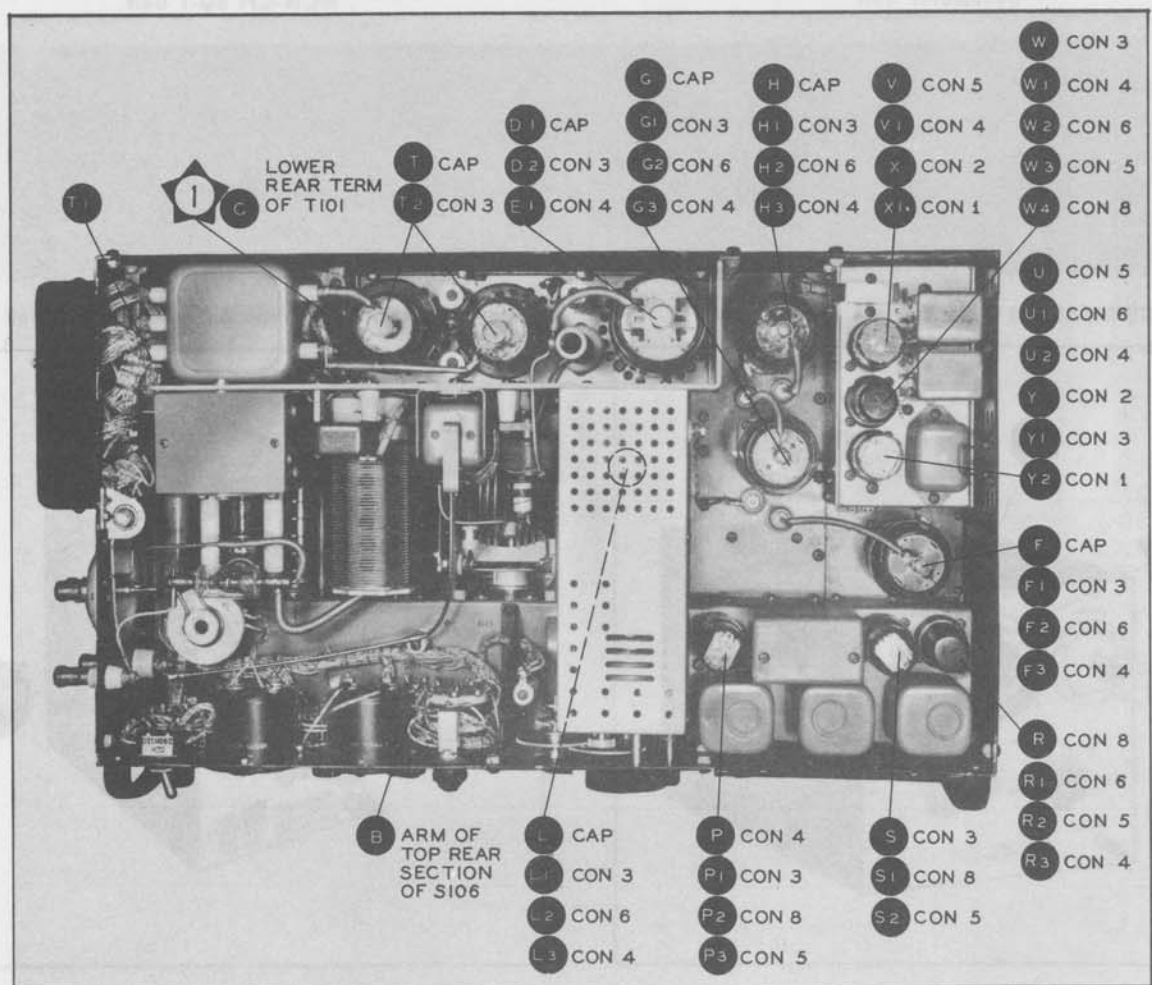
Figure 40. Physical Locations of Test Points
