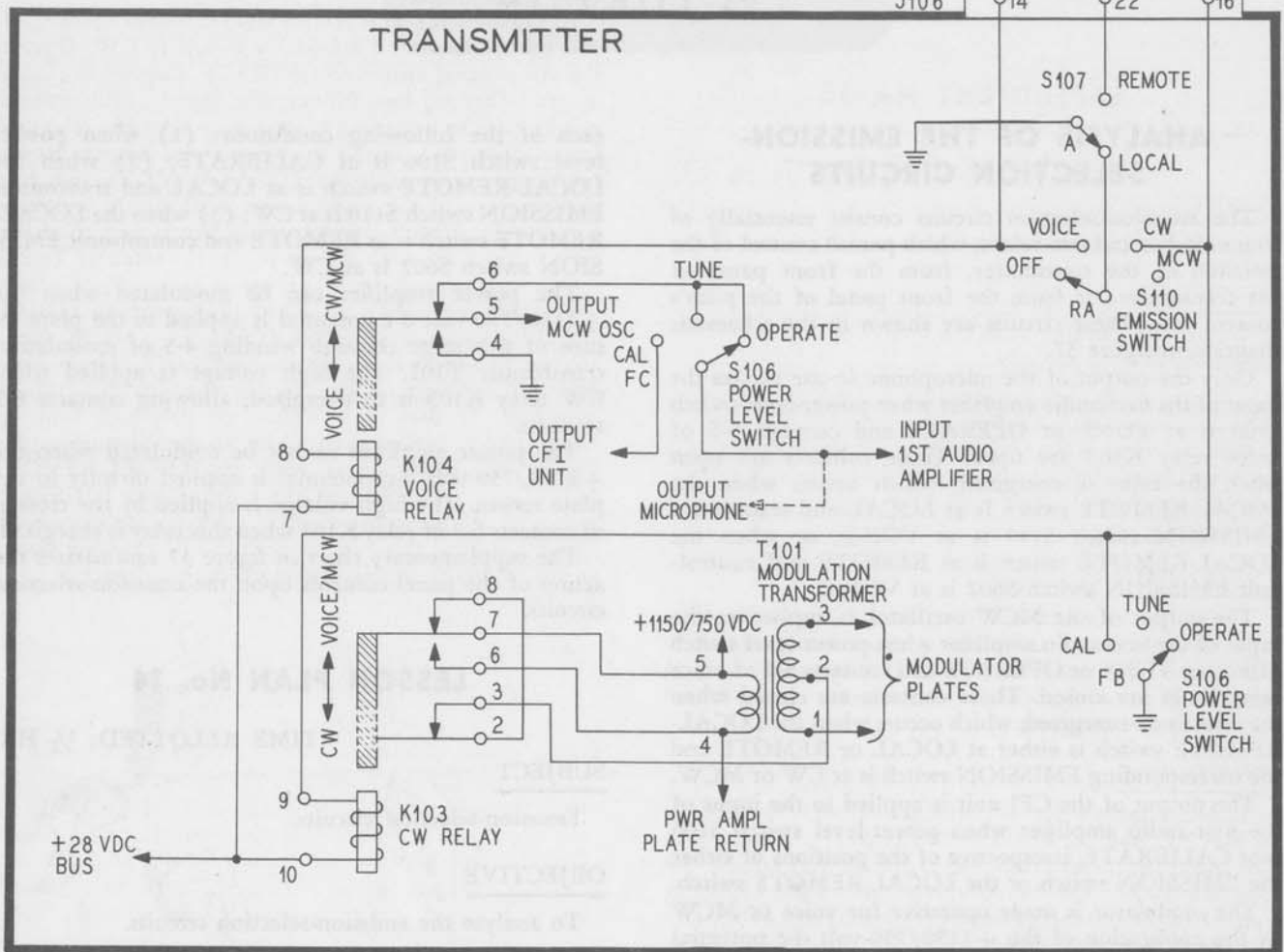
Figure 37. Emission-Selection Circuits
