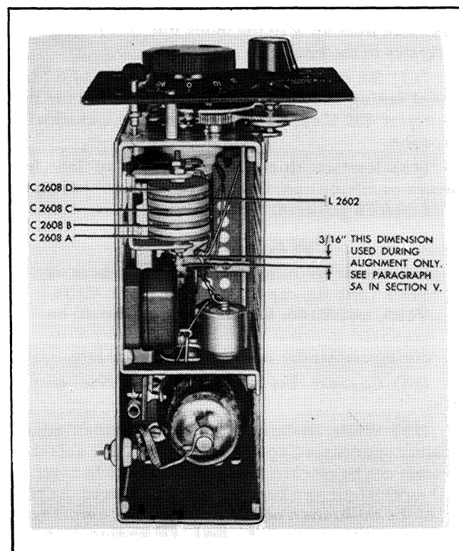
Figure 5-7. Low Frequency Oscillator
