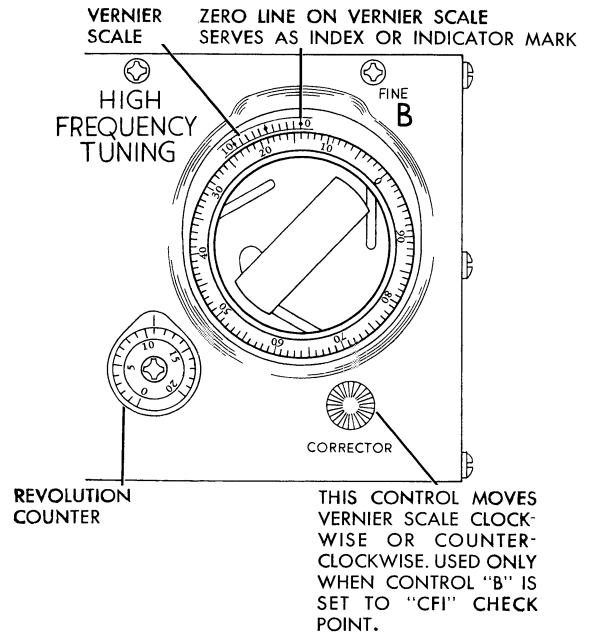
Figure 2-8. Illustration Showing Setting of Control "B" to 1114.1 (Per Example in the Text)
