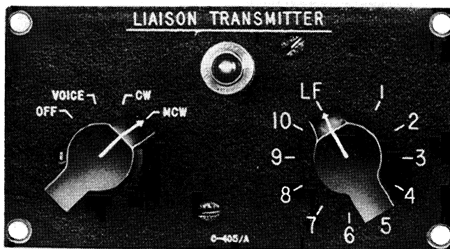
Figure 1-6. Control Panel C-405/A or C-405A/A
