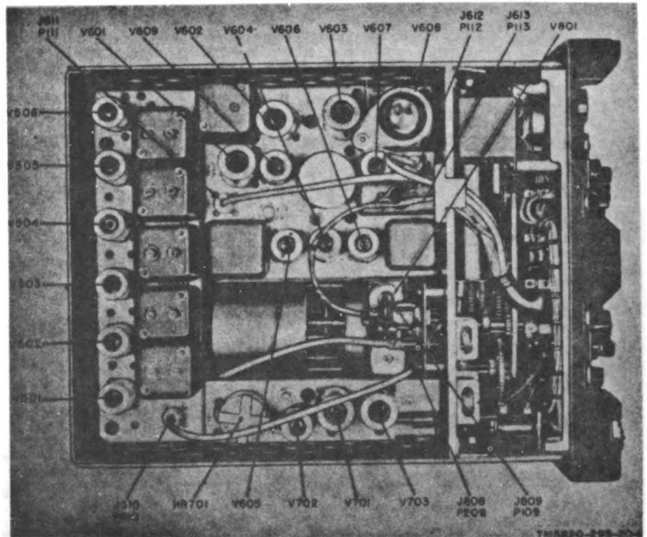
Figure 8. Receiver tube and plug locations, bottom view.
