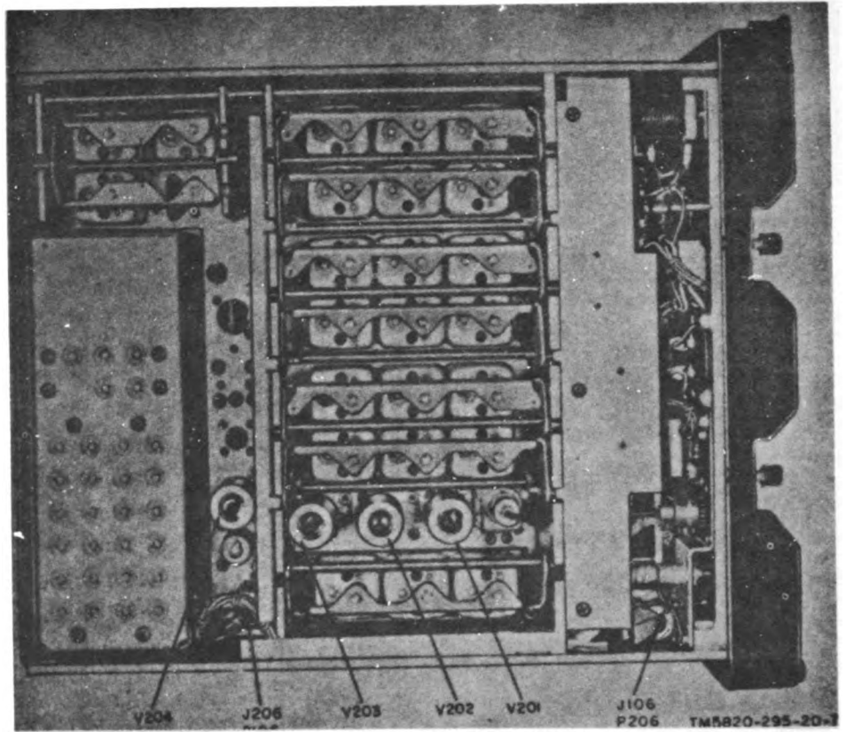
Figure 7. Receiver tube and plug locations, top view.
