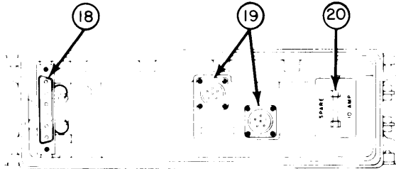
R/T UNIT, REAR PANEL
