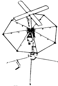
BATTERY BOX WITH BATTERIES INSTALLED
