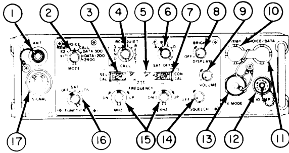
R/T UNIT, FRONT CONTROL PANEL
