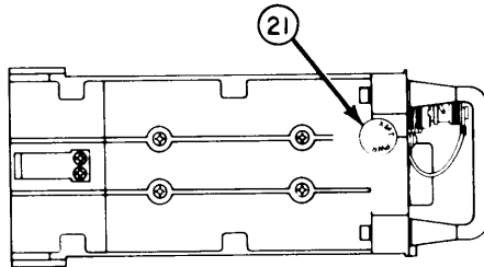
R/T UNIT, SIDE VIEW
