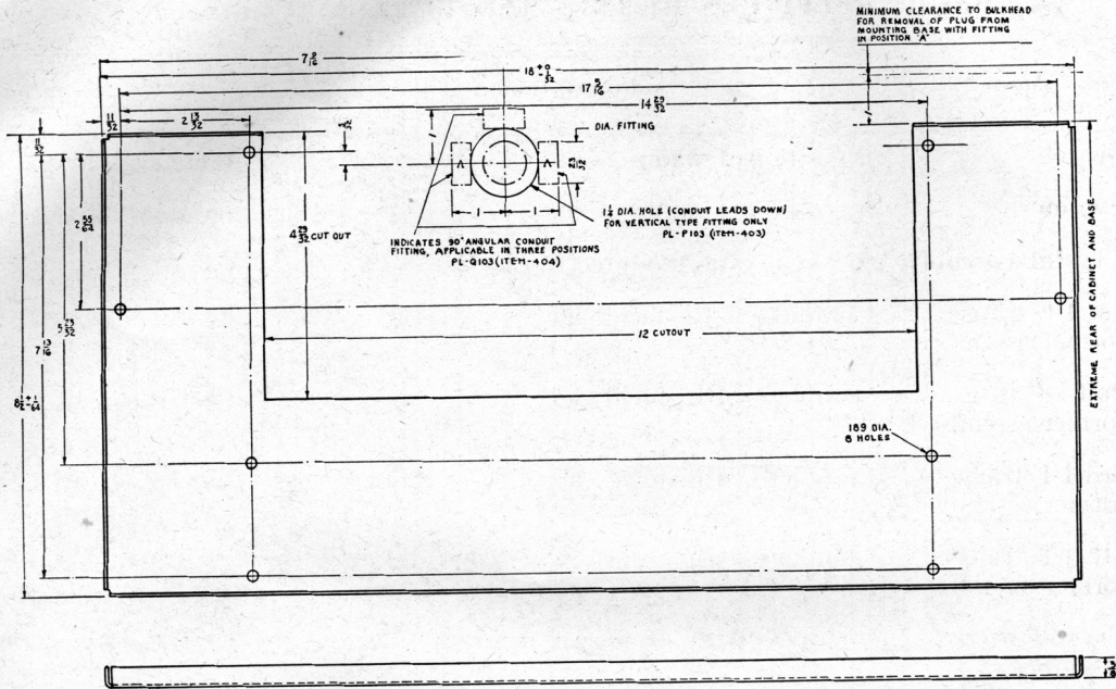
FIGURE 6—RADIO RECEIVER BC-348-S, DRILLING PLAN
