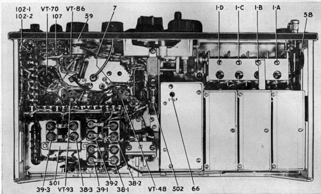
FIGURE 5—RADIO RECEIVER BC-348-S, BOTTOM VIEW OF CHASSIS
