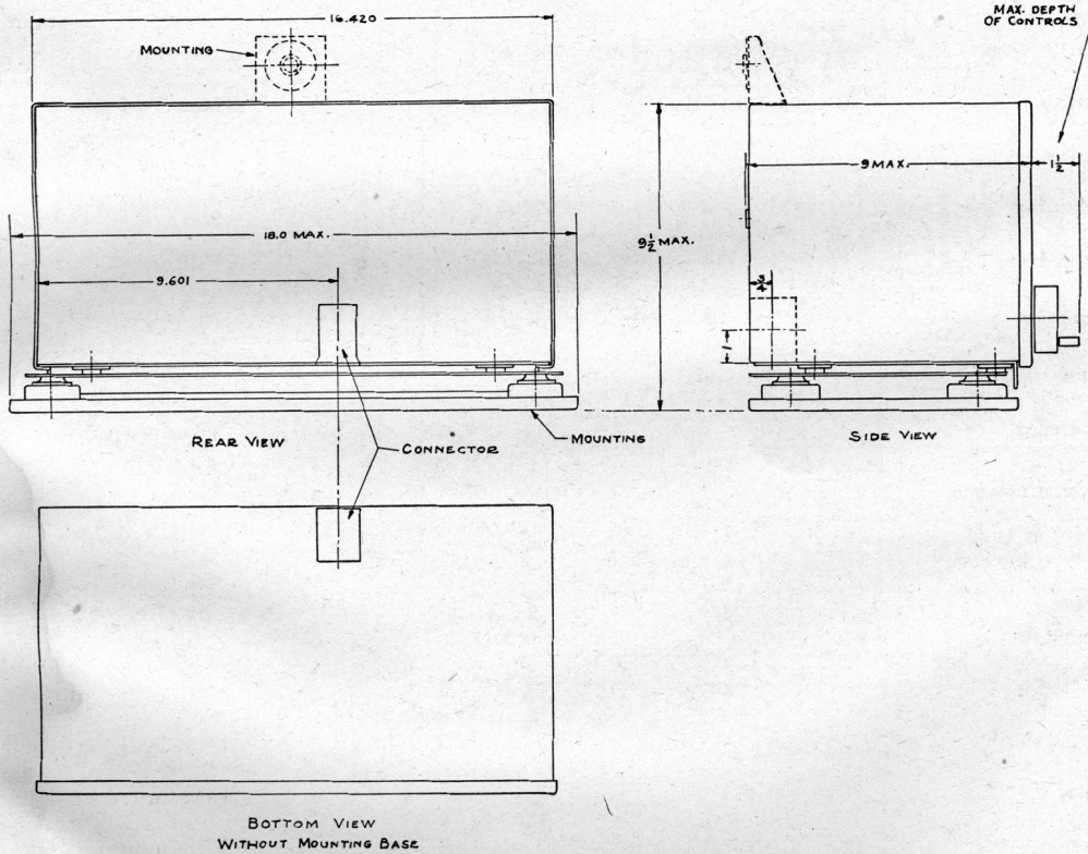
FIGURE 7—RADIO RECEIVER BC-348-S, OUTLINE DIMENSIONAL SKETCH
