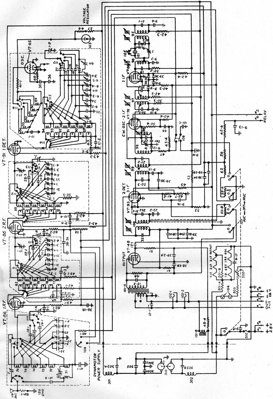
FIGURE 8—RADIO RECEIVER BC-348-S, SCHEMATIC DIAGRAM
