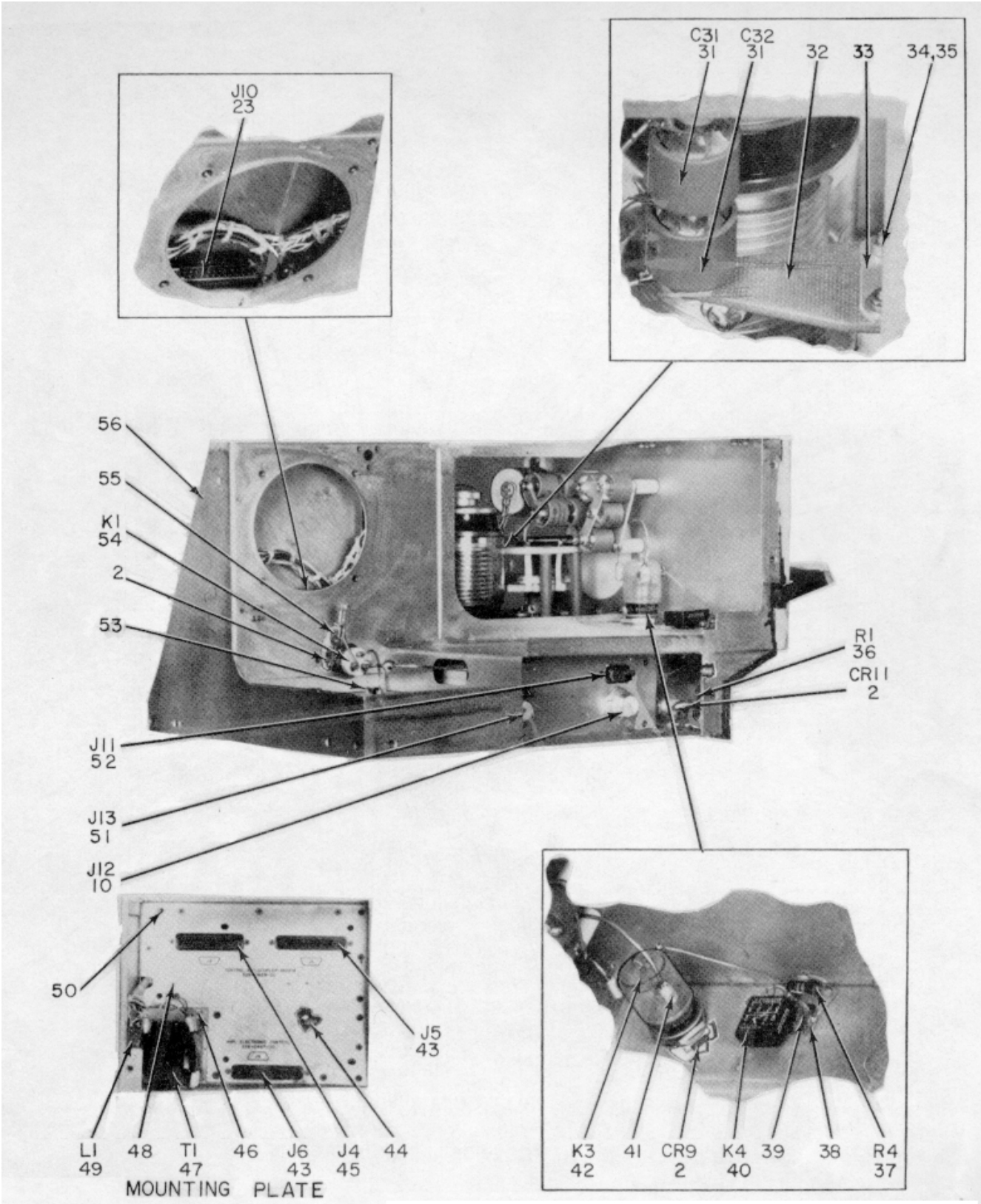
ASSEMBLY VIEW
