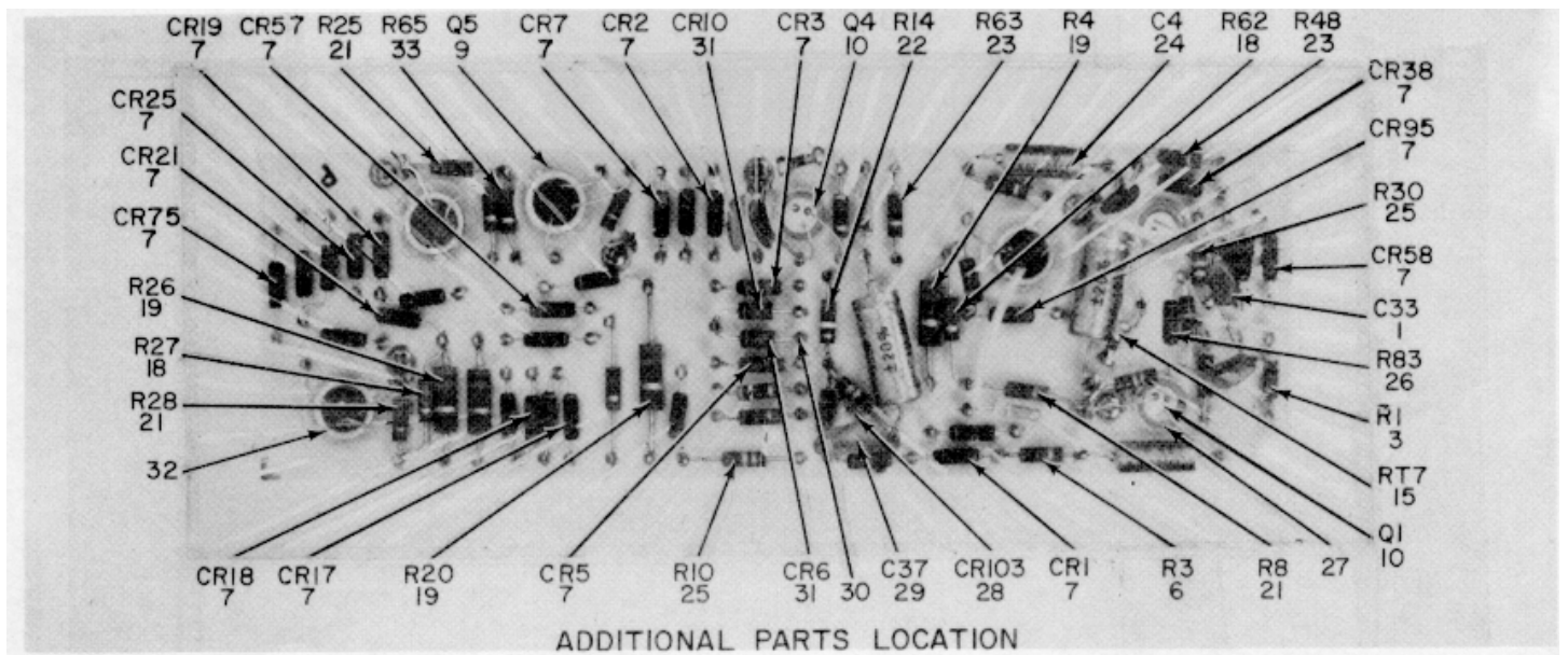
Figure 6. Control, Antenna Coupler (A2) Terminal Board, Rear.
