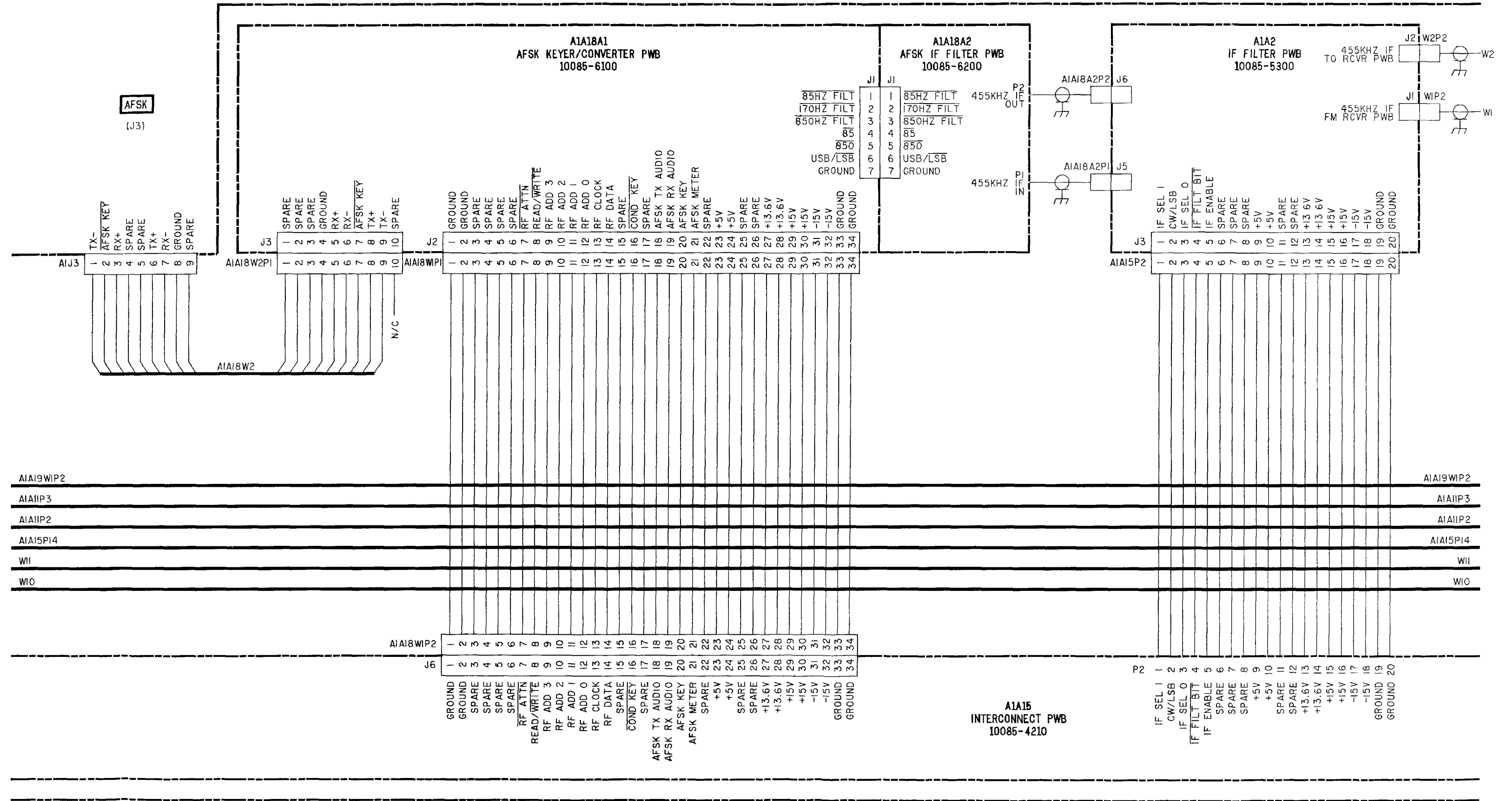
FO-2. TRANSCEIVER ASSY, A1, INTERCONNECTION DIAGRAM (Sheet 4 of 13)
