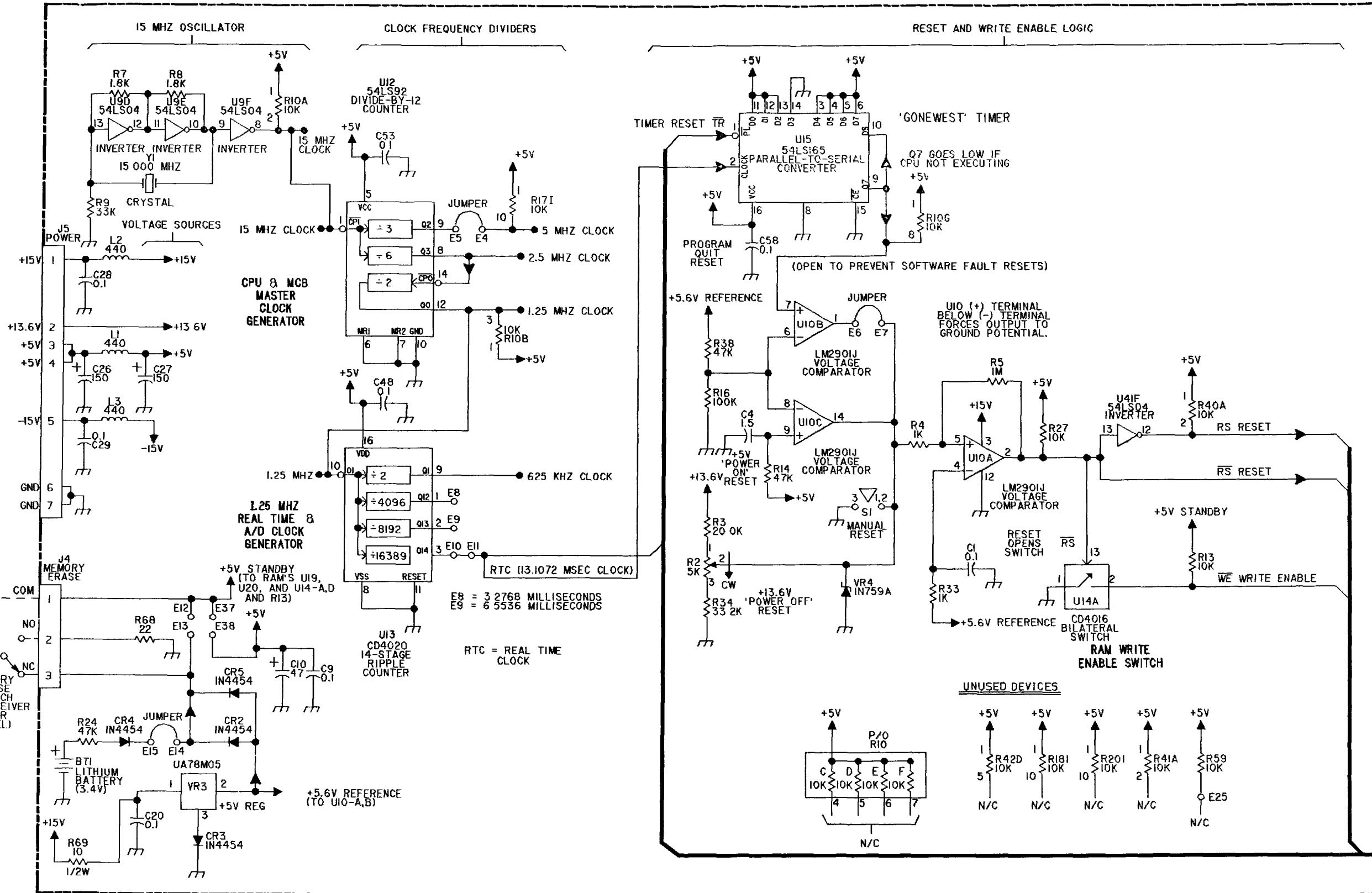
FO-15. TRANSCIVER CONTROL PWB ASSY, A1A12 (Sheet 1 of 9) FP-141(FP-142 Blank)
