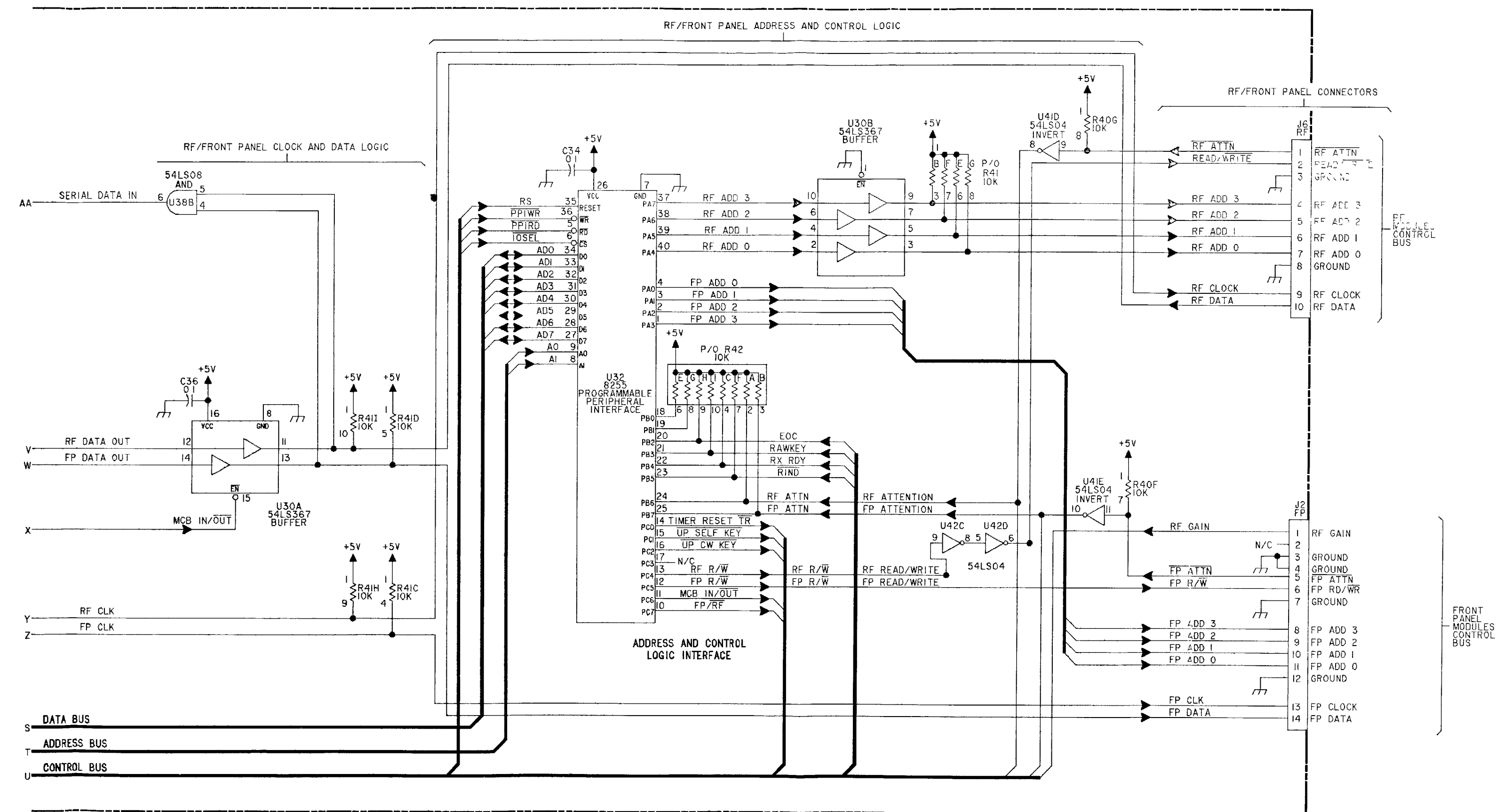
FO-15. TRANSCIVER CONTROL PWB ASSY, A1A12 (Sheet 9 of 9) FP-157/(FP-158 Blank)
