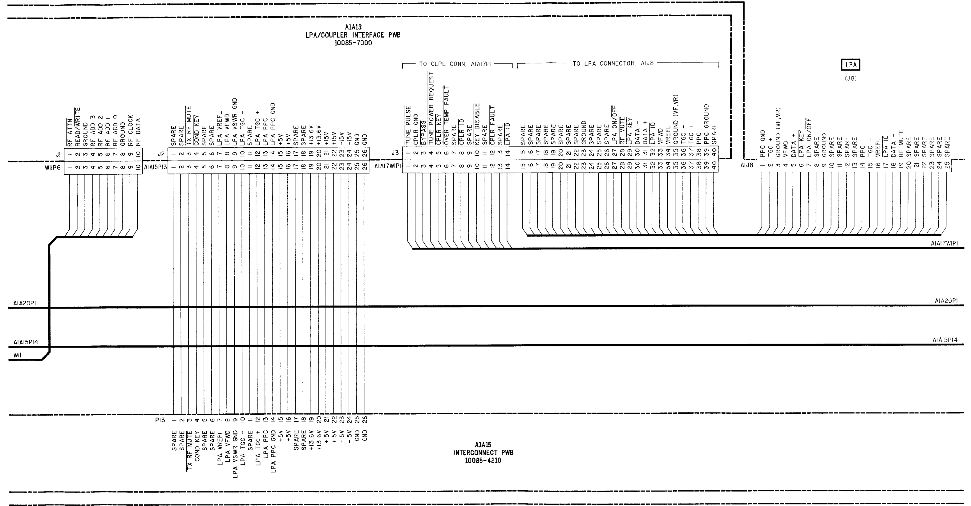
FO-2. TRANSDIVER ASSY, A1, INTERCONNECTION DIAGRAM (Sheet 11 of 13)
