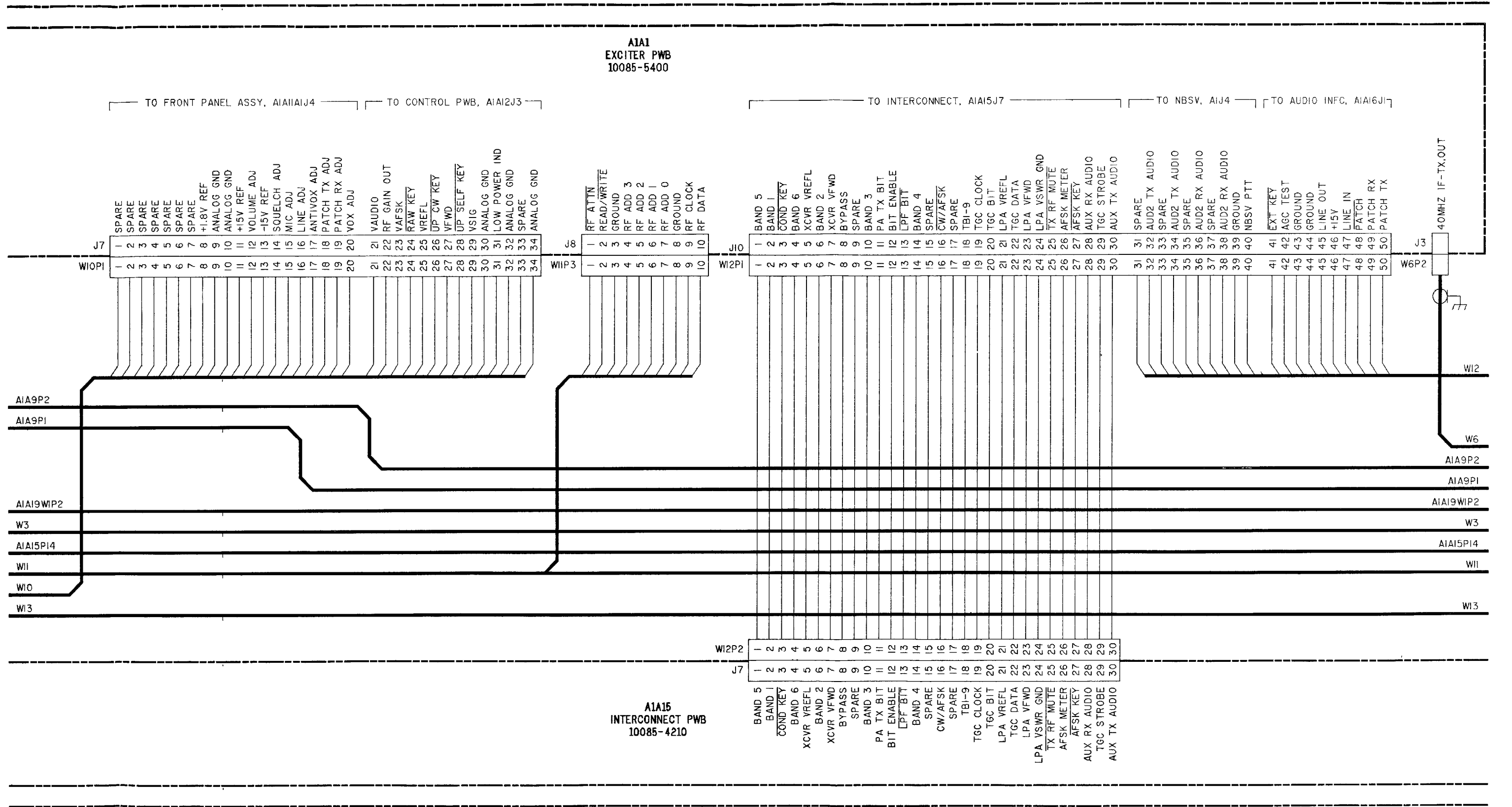
FO-2. TRANSCIVER ASSY, A1, INTERCONNECTION DIAGRAM (Sheet 7 of 13)
