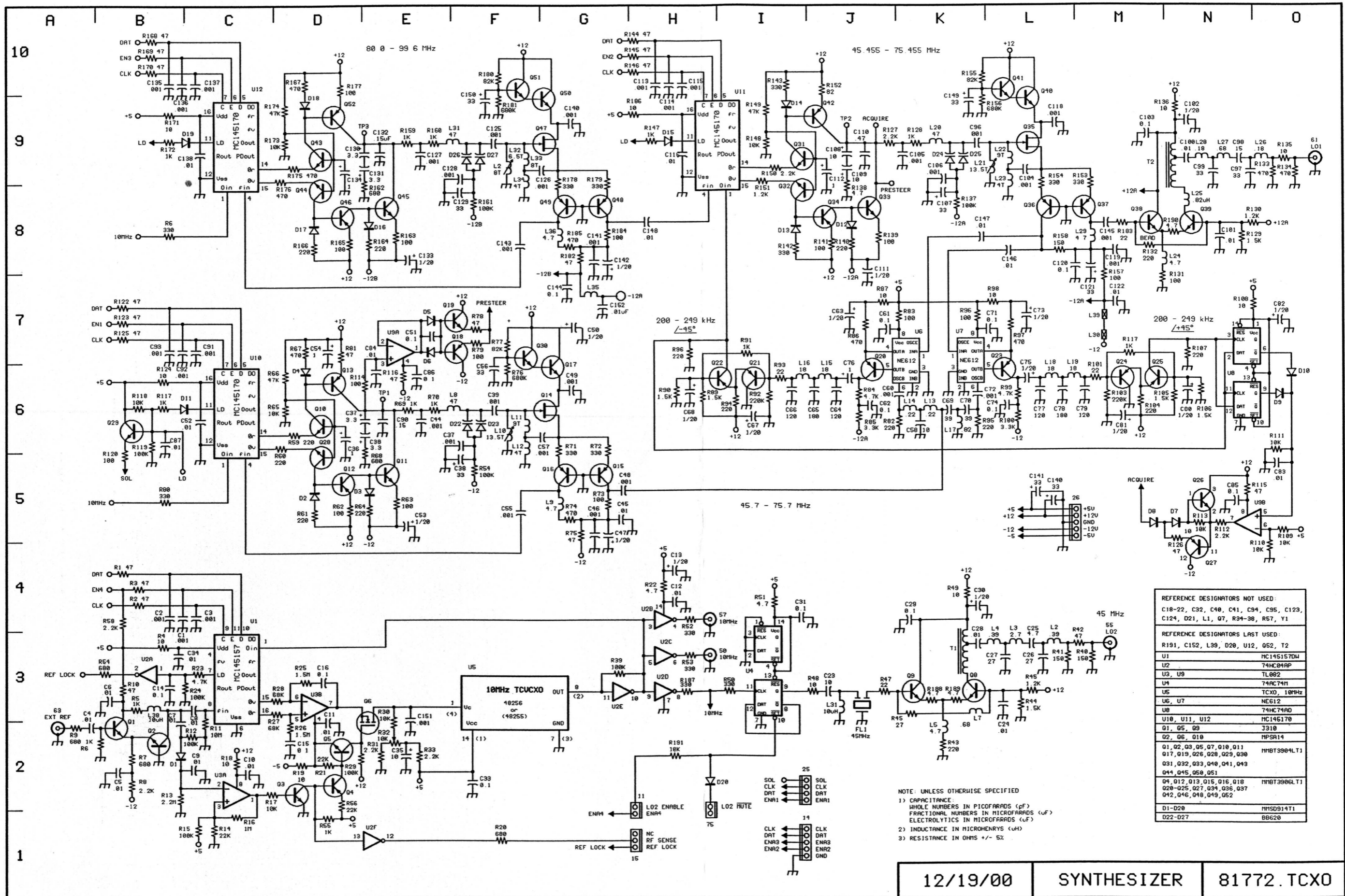
FIGURE 10-29 81772.TCXO SYNTHESIZER SCHEMATIC
