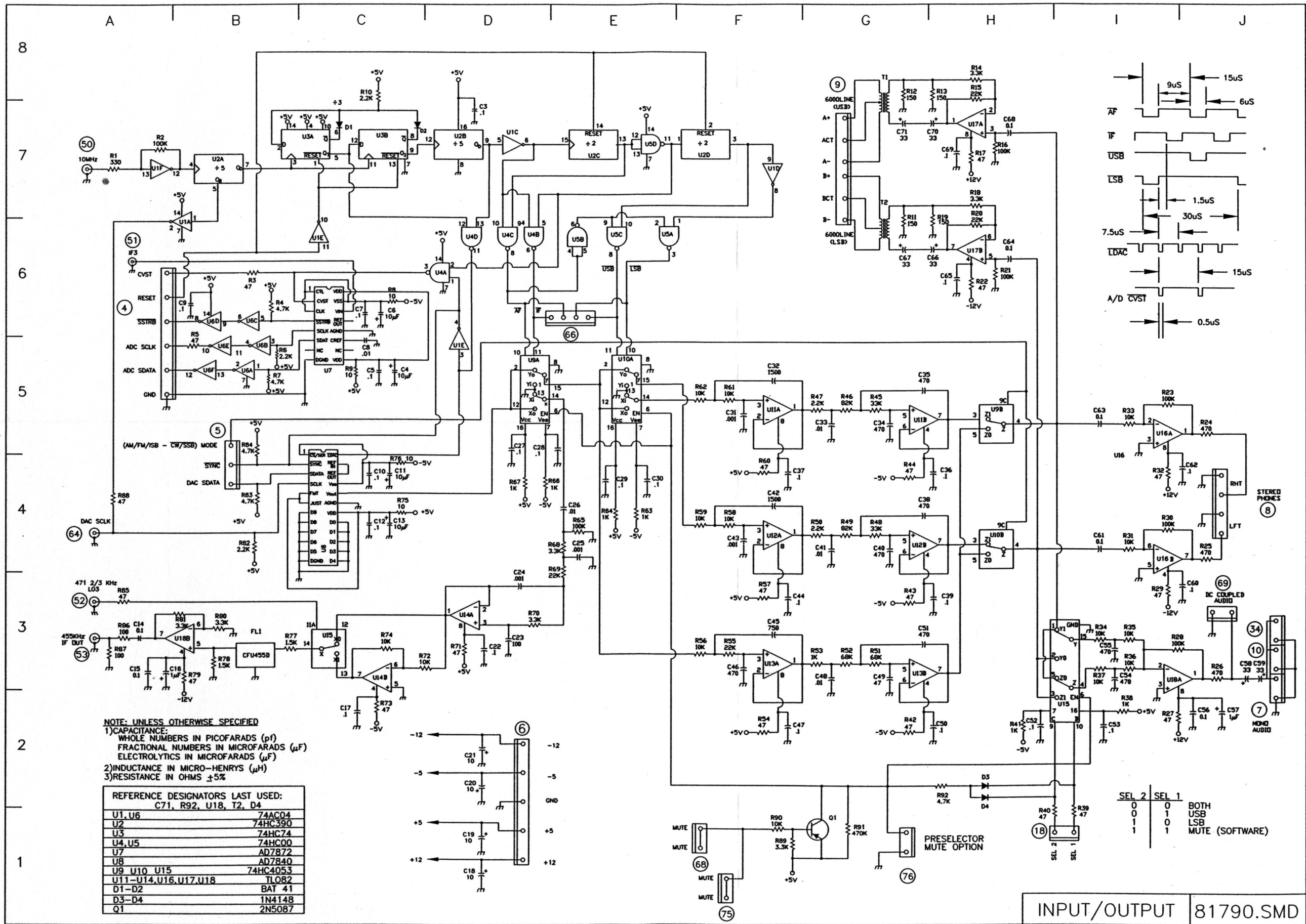
FIGURE 10-23 81790.SMD I/O CONVERTER SCHEMATIC
