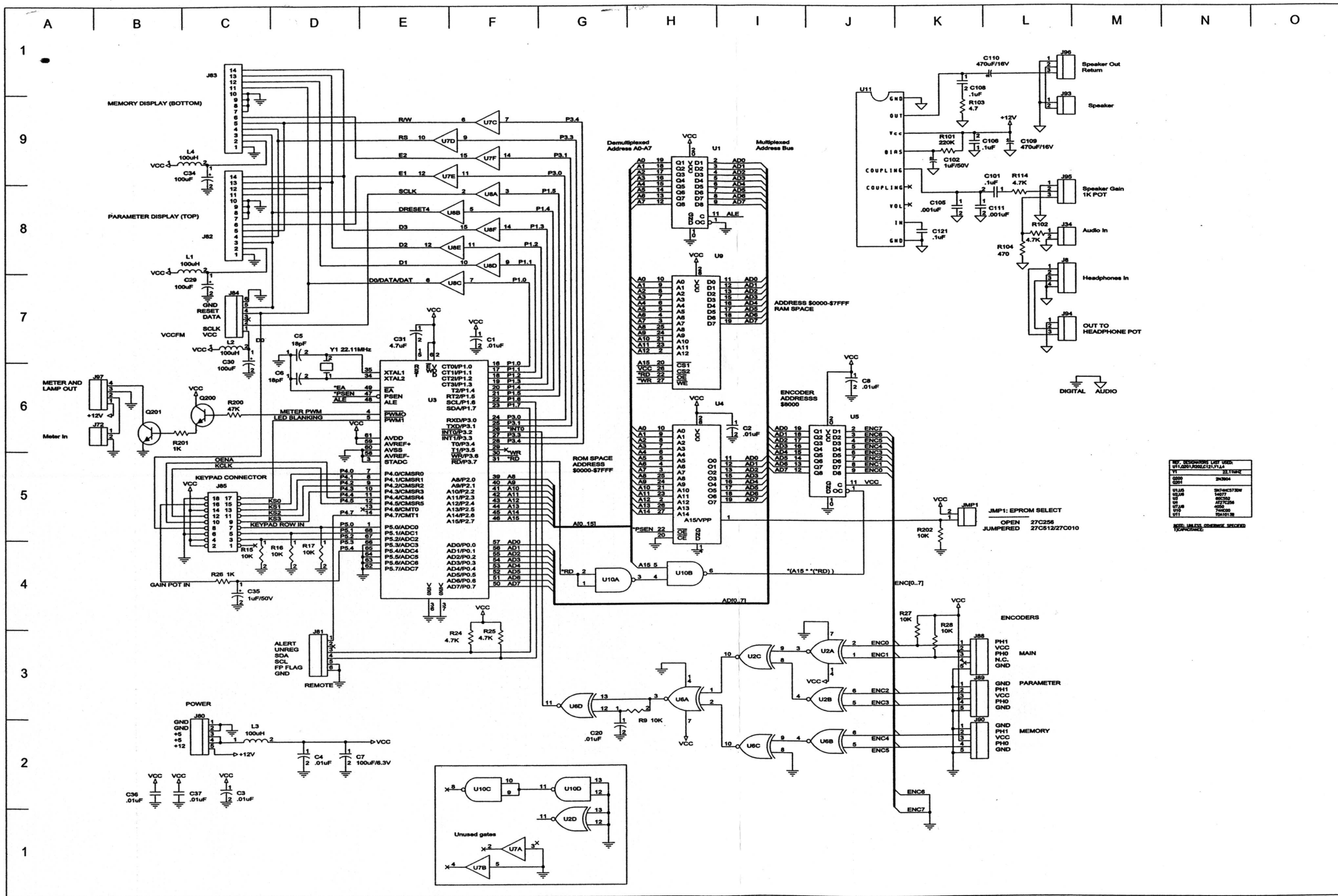
FIGURE 10-43 81819 FRONT PANEL CPU SCHEMATIC
