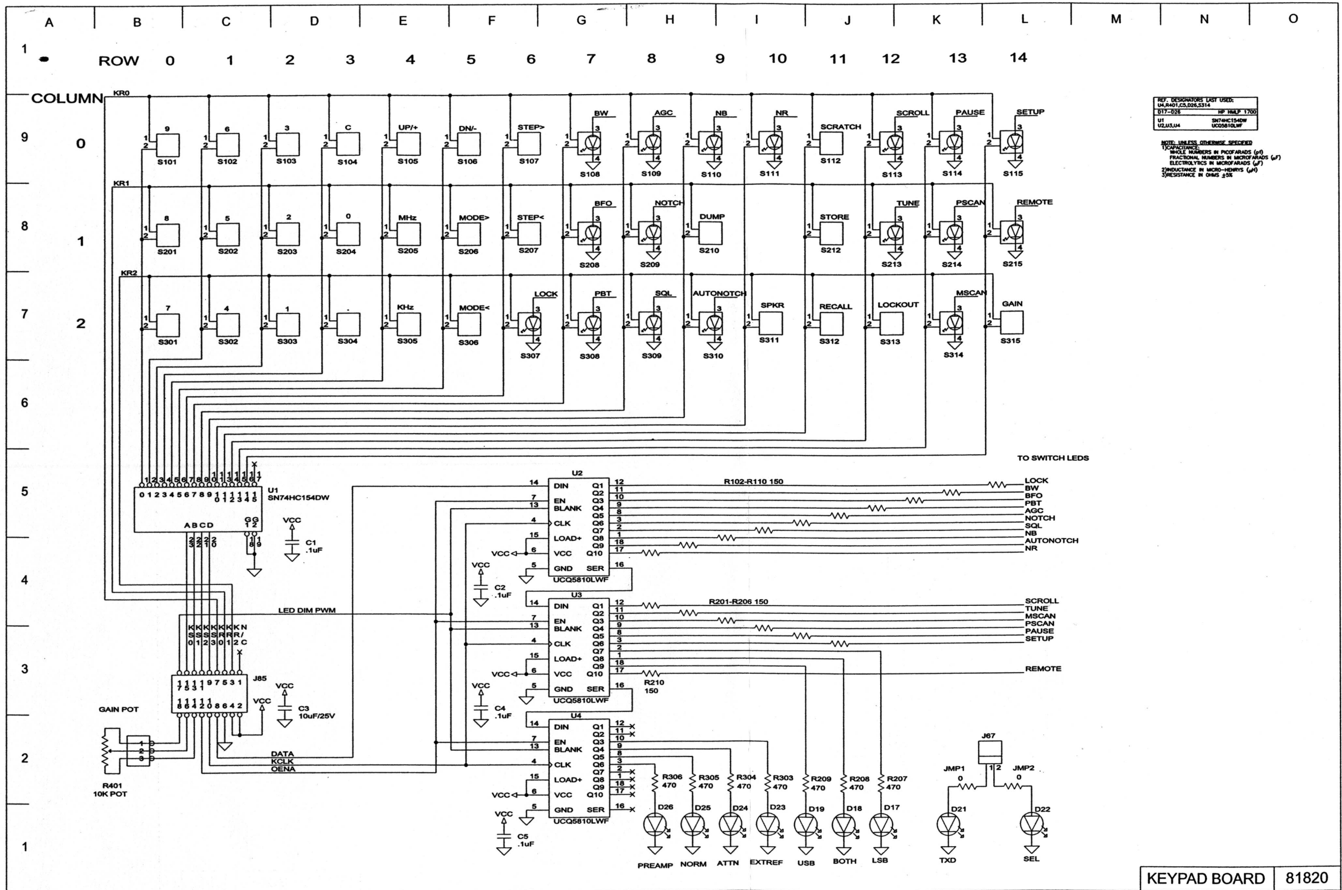
FIGURE 10-48 81820 KEYPAD SCHEMATIC
