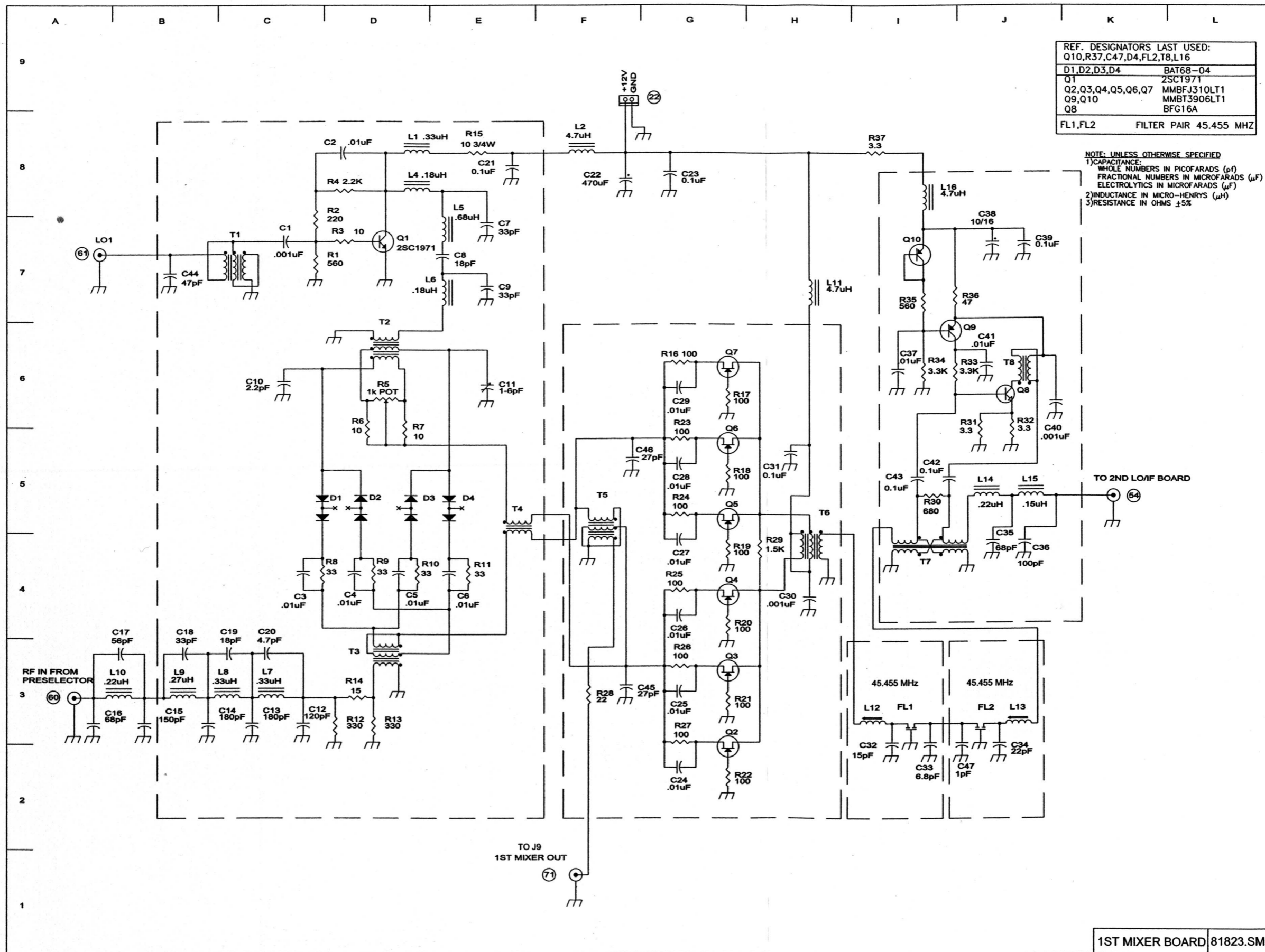
FIGURE 10-13 81823.SMD 1ST MIXER SCHEMATIC
