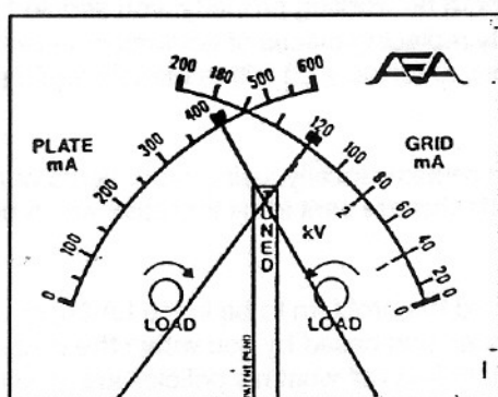
Figure 5.2.3 OPTIMUM LOADING
