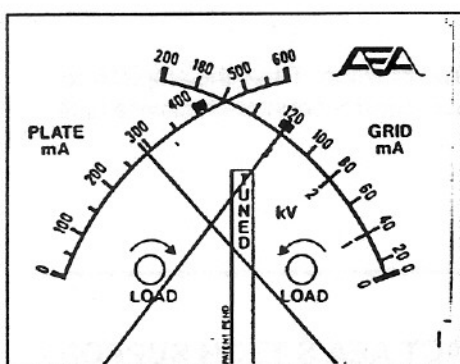
Figure 5.2.1 UNDERLOADED
