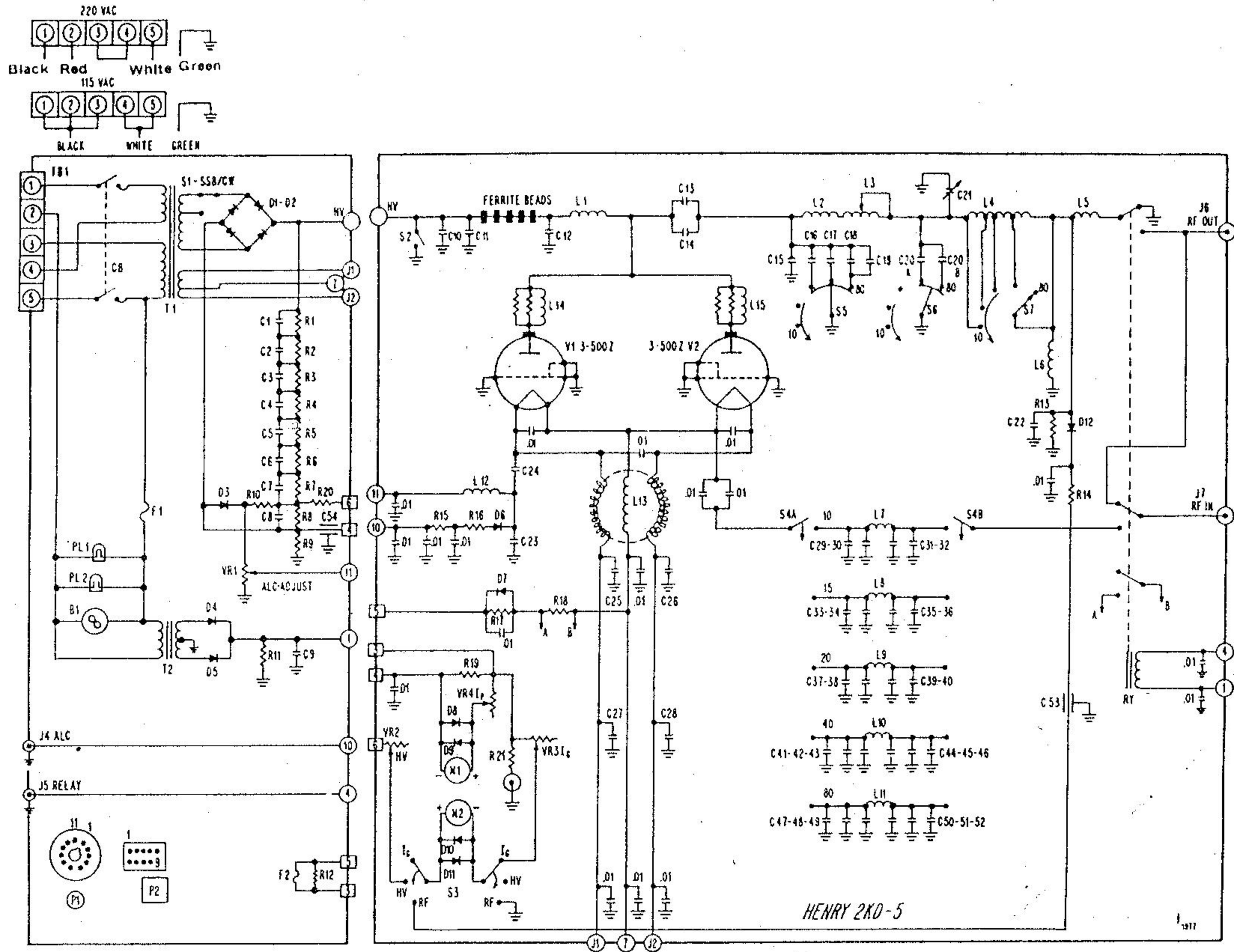
Figure 6. 2KD-5 Schematic Diagram.
