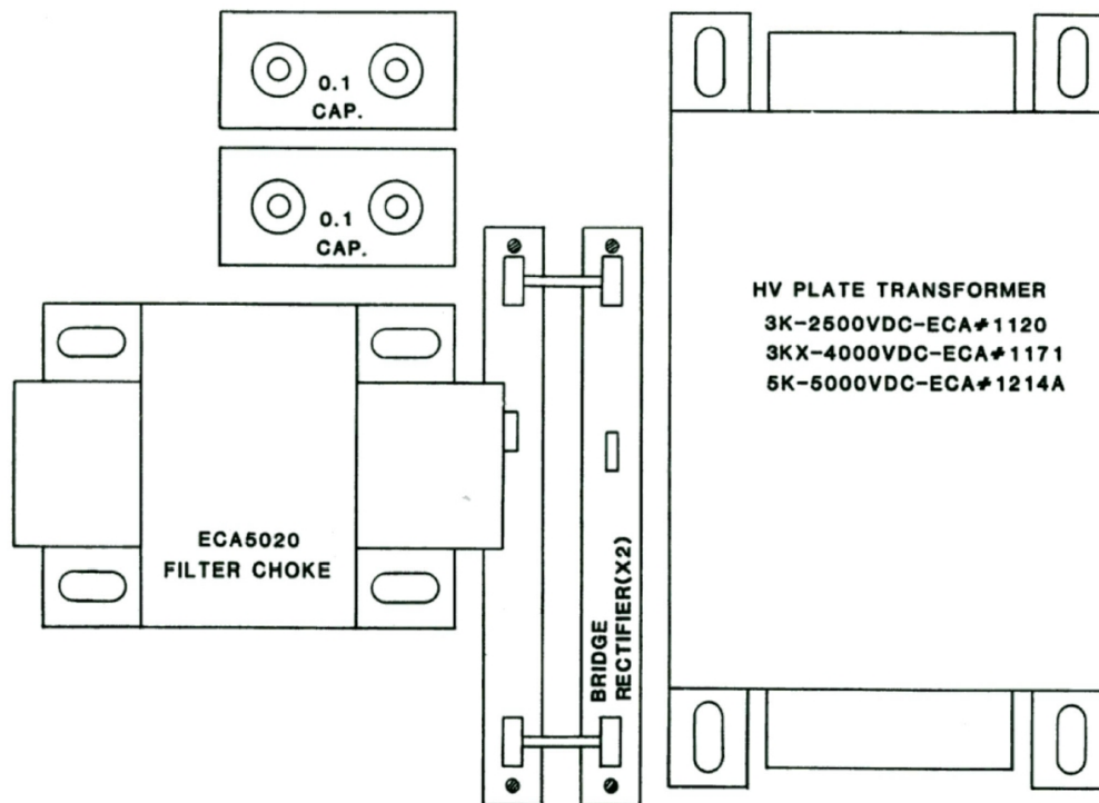
3K&5K CLASSIC POWER SUPPLY-LOWER DECK
