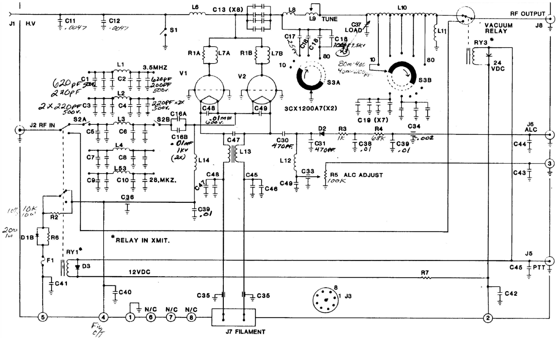
HENRY 5K CLASSIC RF DECK - MARK II
