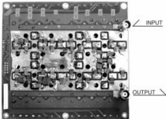
LPF : PC16B1 (BOTTOM VIEW)
