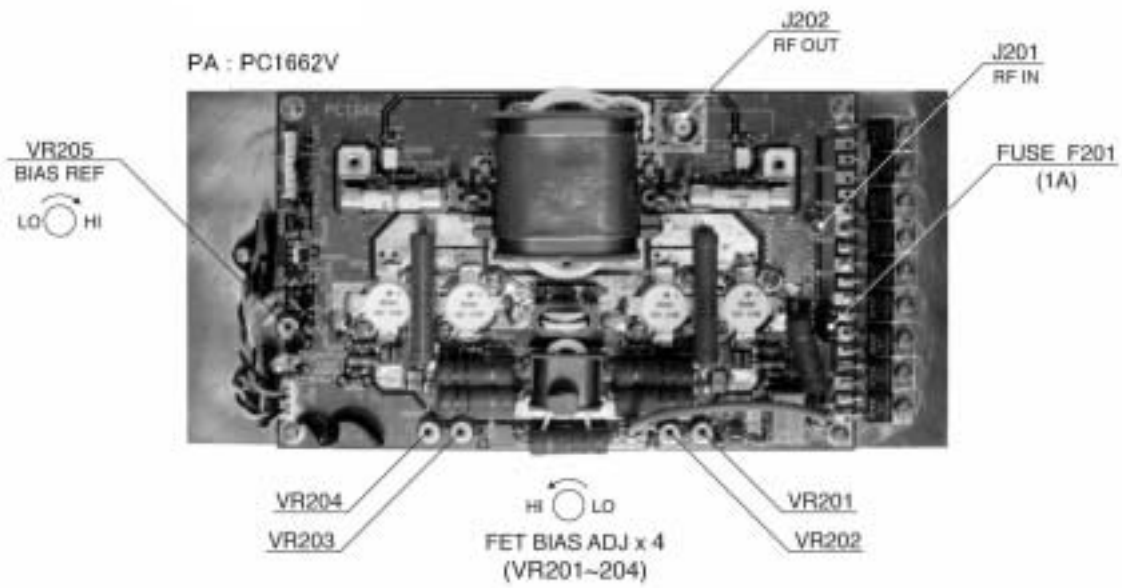
LPF : PC16B1 (TOP VIEW)
