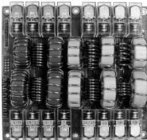
LPF : PC16B1 (TOP VIEW)
