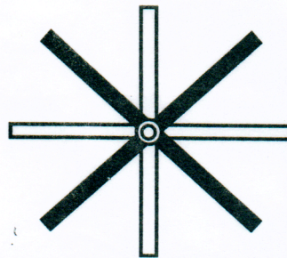
V 2 RADIALS AS SEEN FROM EITHER THE TOP OR THE BOTTOM
