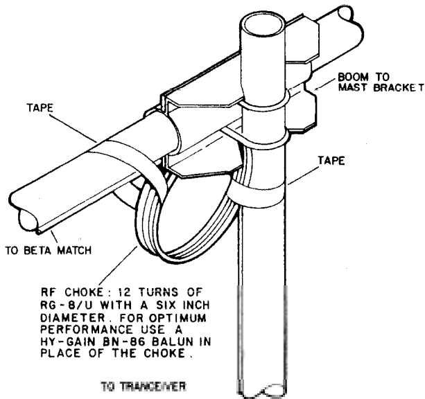
Figure 10 RF Choke
