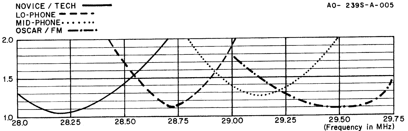
Figure 6 VSWR Chart
