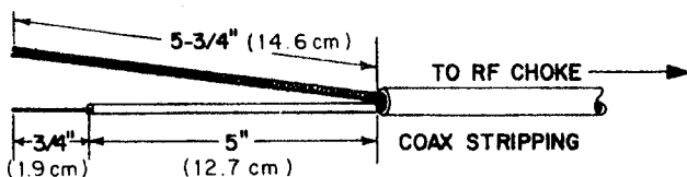
Figure 11 Stripping Coax
