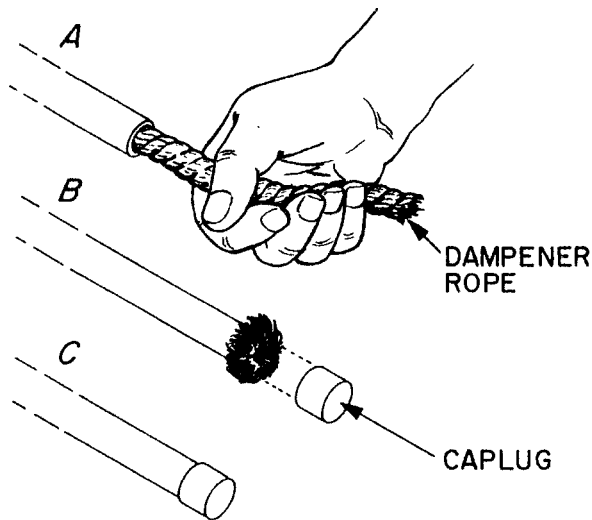
Figure 12 Rope Dampening
