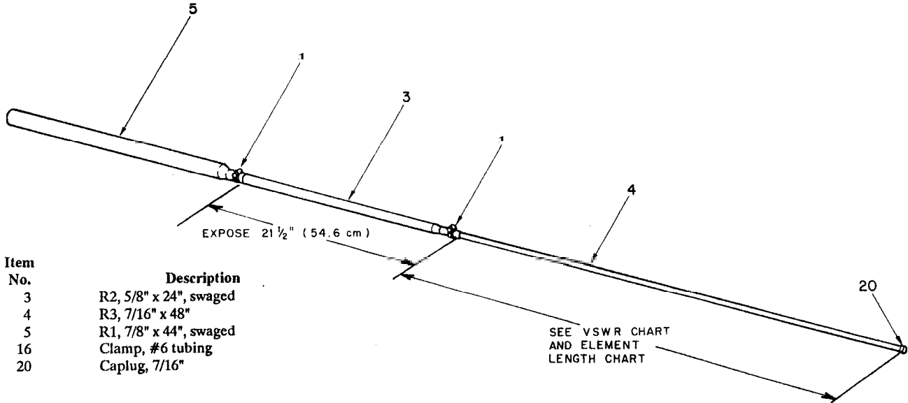
Figure 5 Reflector Element
