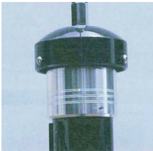
Model 75A "Stubby" -- 21.2 MHz with 5 ft. whip
