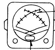
(Fig-1) Meter (Cross needles type) : Indicating SWR, Forward & Reflected Power. Power Range Selector: Set to required power range.
