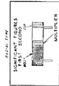
JAN COLOR CODE FOR FIXED COMPOSITION RESISTORS
