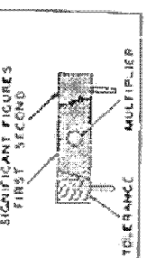
RMA COLOR CODE FOR FIXED COMPOSITION RESISTORS
