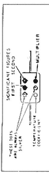
JAN 8-DOT COLOR CODE FOR PAPER DIELECTRIC CAPACITORS
