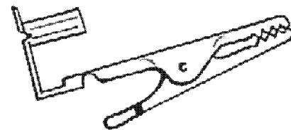
Fig. 2. Pin socket & clip detail
