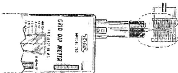
Fig. 1A. Preferred method (inductive coupling)
