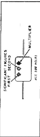
PMA 3-DOT COLOR CODE FOR MICA DIELECTRIC CAPACITORS
