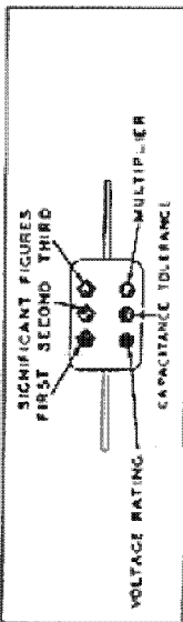
PMA 8-DOT COLOR CODE FOR MICA-DIELECTRIC CAPACITORS
