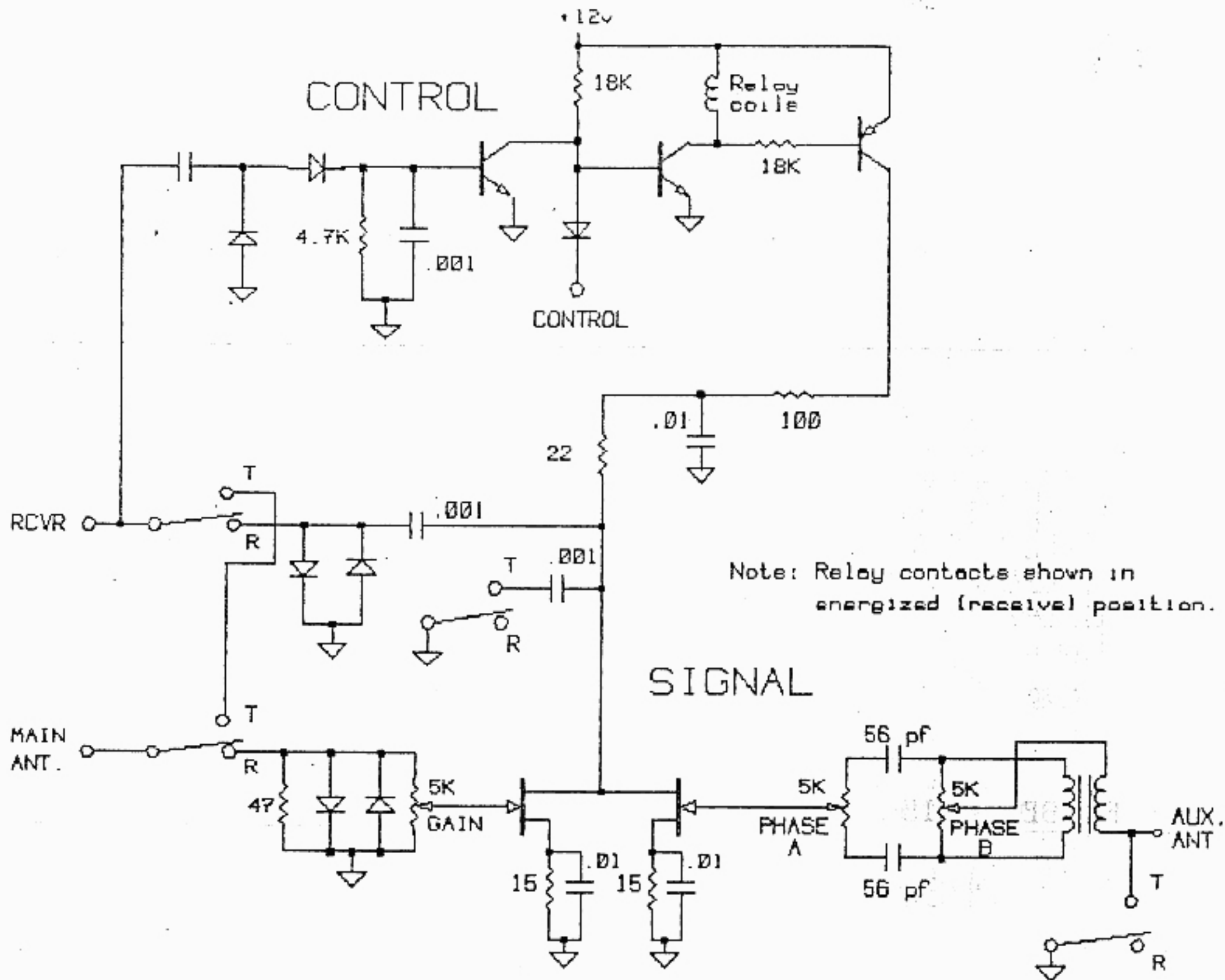
S.E.M. QRM ELIMINATOR Schematic
